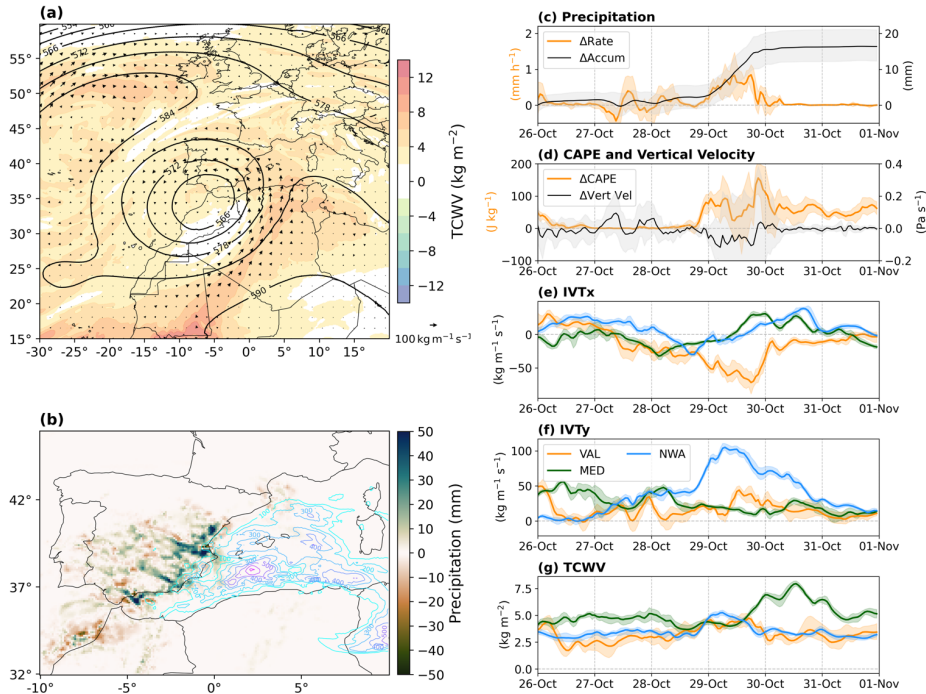
585 Figure 4: (a) Composite of mean daily differences (Factual – Counterfactual) on 29 October for IVT (arrows) and TCWV (shading). Contours show the daily mean 500-hPa geopotential height (dam) in the Factual scenario (as in Figure 1a–b). (b) Mean daily precipitation differences (shading, mm) and CAPE (contours, \text{J kg}^{-1} ) on 29 October. For CAPE, only positive differences above 100 \text{ J kg}^{-1} are shown. (c) Hourly differences in precipitation rate (orange) and accumulated precipitation (black) over VAL. Solid lines indicate the mean difference, and shading shows the minimum–maximum range. Accumulated precipitation is computed starting at 00 UTC on 24 October. (d) As in (c), but for CAPE (orange) and vertically-averaged vertical velocity (black). (e) As in (d), but for hourly differences in IVTx over VAL (orange), NWA (blue), and MED (green). (f) As in (e), but for IVTy. (g) As in (f), but for TCWV. The shading in panels (c) to (g) shows the minimum–maximum range obtained using all the ensemble members. 590
