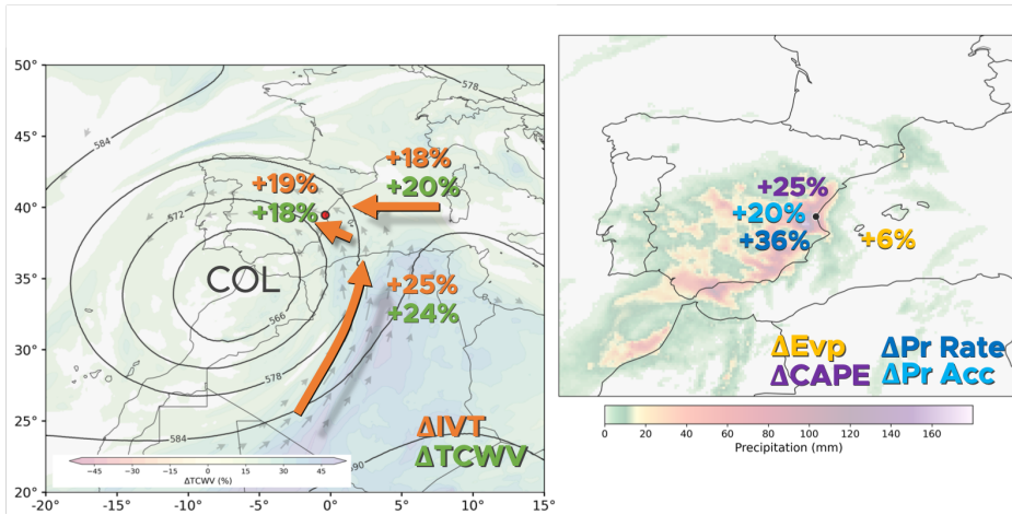
Figure 8: Schematic figure of the relative changes between Factual and Counterfactual scenarios. Total column water vapor ( \Delta TCWV, in green) and integrated water vapour transport ( \Delta IVT, in orange) on the left. Precipitation rate ( \Delta Pr Rate, in dark blue), accumulated precipitation ( \Delta Pr Acc, in light blue), evaporation ( \Delta Evap, in yellow) and most unstable convective available potential energy ( \Delta CAPE, in purple) on the right.
