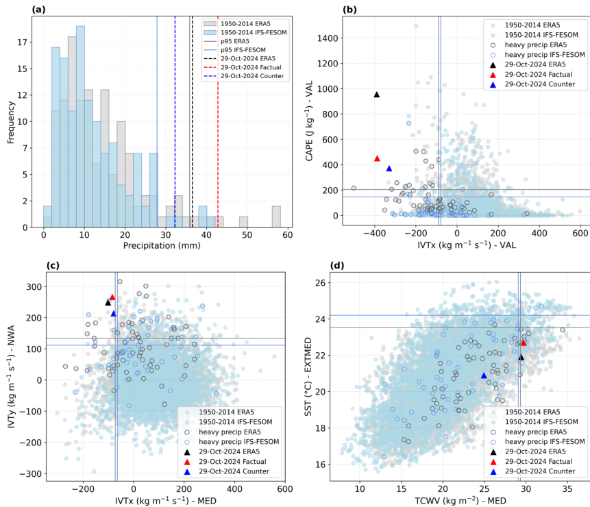
500 Figure 3: (a) Distribution of maximum daily precipitation (Rx1day) in Valencia (VAL box) for October–November during 1950– 2014 in ERA5 (light grey bars) and IFS-FESOM free run (light blue bars). (b) Daily mean IVTx and CAPE values spatially averaged over VAL for October–November during 1950–2014 in ERA5 (light grey circles) and IFS-FESOM (light blue circles). (c) 505 As in (b), but for the 3-day mean IVTx values spatially averaged over the Mediterranean box (MED) and IVTy over northwestern Africa box (NWA). (d) As in (c), but for TCWV over MED and SST over an extended Mediterranean box (EXTMED; 36.5°– 40.5°N; 0.0°–8.5°E). Thin vertical lines (light grey for ERA5, light blue for IFS-FESOM) indicate the 5th or 95th percentiles of the 1950–2014 reference period, as appropriate. Dashed vertical lines in (a) and triangles in (b)–(d) denote the values on 29 October for ERA5 (black) and for the Factual (red) and Counterfactual (blue) scenarios. Bordered circles in (b) indicate days with heavy precipitation in VAL (defined as exceeding the 75th percentile). In (c) and (d), bordered circles indicate heavy-precipitation days based on the last day of the 3-day period.
