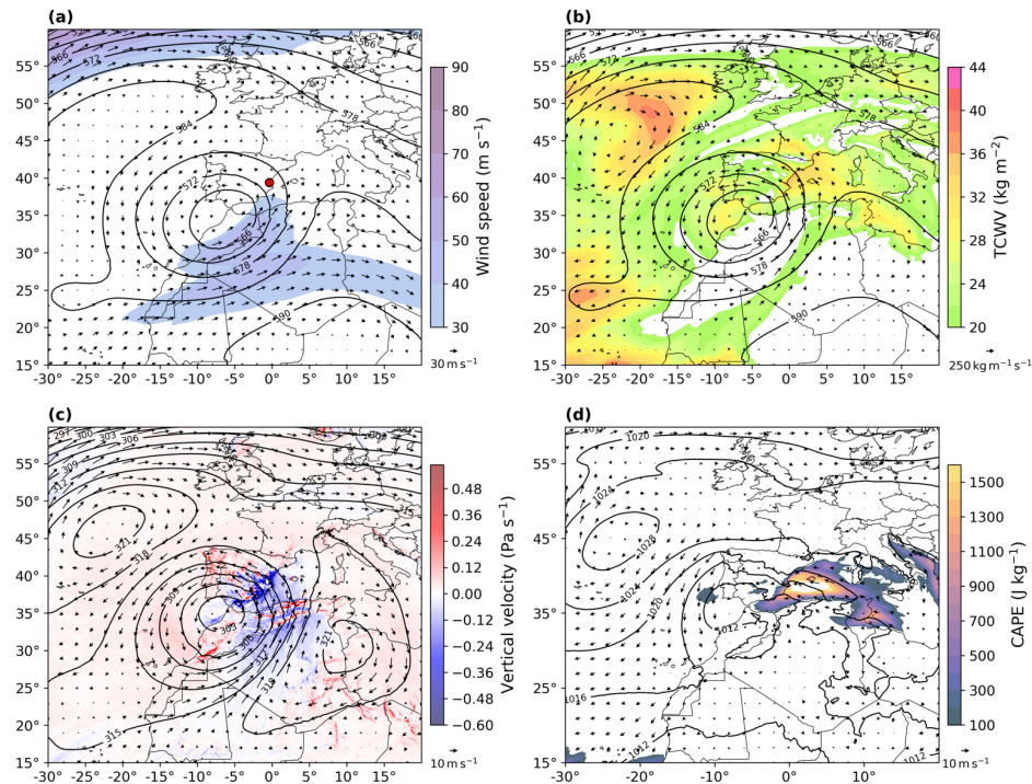
Figure 1: Daily composite for the 29 October 2024 from the Factual scenario for (a) 500-hPa geopotential height (contours, dam), 300-hPa wind (arrows, \text{m s}^{-1} ) and 300-hPa wind speed (colours, \text{m s}^{-1} ), (b) 500-hPa geopotential height (contours, dam), integrated water vapour transport (IVT, arrows, \text{kg m}^{-1} \text{ s}^{-1} ) and total column water vapour (TCWV, colours, \text{kg m}^{-2} ), (c) 700-hPa
