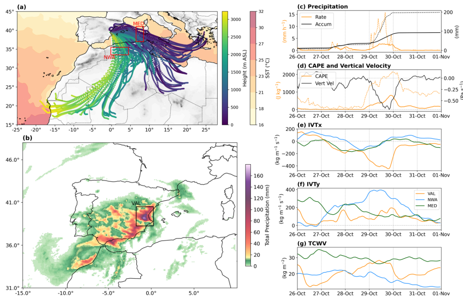
475 Figure 2: (a) 72-hour backward trajectories from the HYSPLIT model for air parcels arriving in Valencia at 12Z on 29 October, and 7-day mean (24-30 Oct) SSTs ( ^{\circ}\text{C} ) from NOAA OISSTv2. Red boxes indicate the Mediterranean (MED) and Northwestern Africa (NWA) boxes. (b) 24-hour accumulated precipitation on 29 October from the Factual scenario, with the Valencia (VAL) box shown in black. (c) Hourly precipitation rate (orange) and accumulated precipitation (black) over the Valencia box. Solid lines indicate the box mean, and dashed lines indicate the grid cell with the highest accumulation. Accumulated precipitation is computed starting at 00 UTC on 24 October. (d) Vertically-averaged vertical velocity (black) and CAPE (orange) over the Valencia box. Solid lines show the box mean, and the orange dashed line indicates the highest hourly CAPE within the box. (e) Hourly mean zonal IVT (IVTx) over VAL (orange), NWA (blue), and MED (green). (f) As in (e), but for meridional IVT (IVTy). (g) As in (f), but for TCWV. 480
