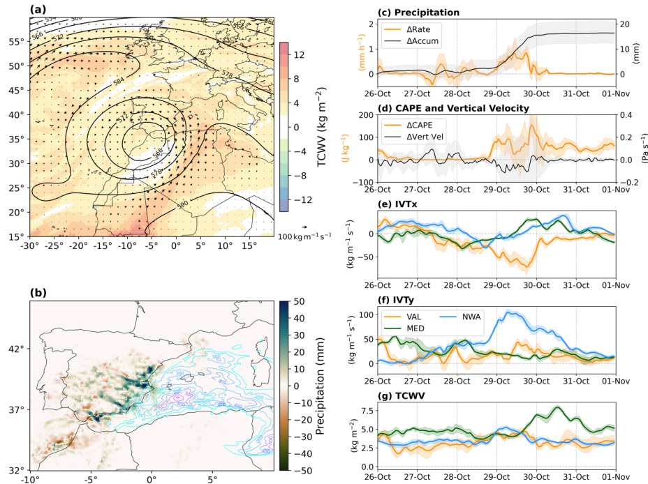
450 Figure 4: (a) Composite of mean daily differences (Factual – Counterfactual) on 29 October for IVT (arrows) and TCWV (shading). Contours show the daily mean 500-hPa geopotential height (dam) in the Factual scenario (as in Figure 1a–b). (b) Mean daily precipitation differences (shading, mm) and CAPE (contours, J kg -1 ) on 29 October. For CAPE, only positive differences above 100 J kg -1 are shown. (c) Hourly differences in precipitation rate (orange) and accumulated precipitation (black) over VAL. Solid lines indicate the mean difference, and shading shows the minimum–maximum range. Accumulated precipitation is computed starting at 00 UTC on 24 October. (d) As in (c), but for CAPE (orange) and vertically-averaged vertical velocity (black). (e) As in (d), but for hourly differences in IVT over VAL (orange), NWA (blue), and MED (green). (f) As in (e), but for IVT. (g) As in (f), but for TCWV. The shading in panels (c) to (g) shows the minimum–maximum range obtained using all the ensemble members.
