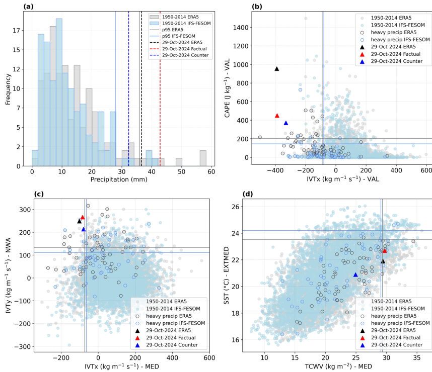
365 Figure 3: (a) Distribution of maximum daily precipitation (Rx1day) in Valencia (VAL box) for October–November during 1950– 2014 in ERA5 (light grey bars) and IFS-FESOM free run (light blue bars). (b) Daily mean IVTx and CAPE values spatially 370 averaged over VAL for October–November during 1950–2014 in ERA5 (light grey circles) and IFS-FESOM (light blue circles). (c) As in (b), but for the 3-day mean IVTx values spatially averaged over the Mediterranean box (MED) and IVTy over northwestern Africa box (NWA). (d) As in (c), but for TCWV over MED and SST over an extended Mediterranean box (EXTMED; 36.5°– 40.5°N; 0.0°–8.5°E). Thin vertical lines (light grey for ERA5, light blue for IFS-FESOM) indicate the 5th or 95th percentiles of the 1950–2014 reference period, as appropriate. Dashed vertical lines in (a) and triangles in (b)–(d) denote the values on 29 October for ERA5 (black) and Counterfactual (blue) scenarios. Bordered circles in (b) indicate days with heavy precipitation in VAL (defined as exceeding the 75th percentile). In (c) and (d), bordered circles indicate heavy-precipitation days based on the last day of the 3-day period.
