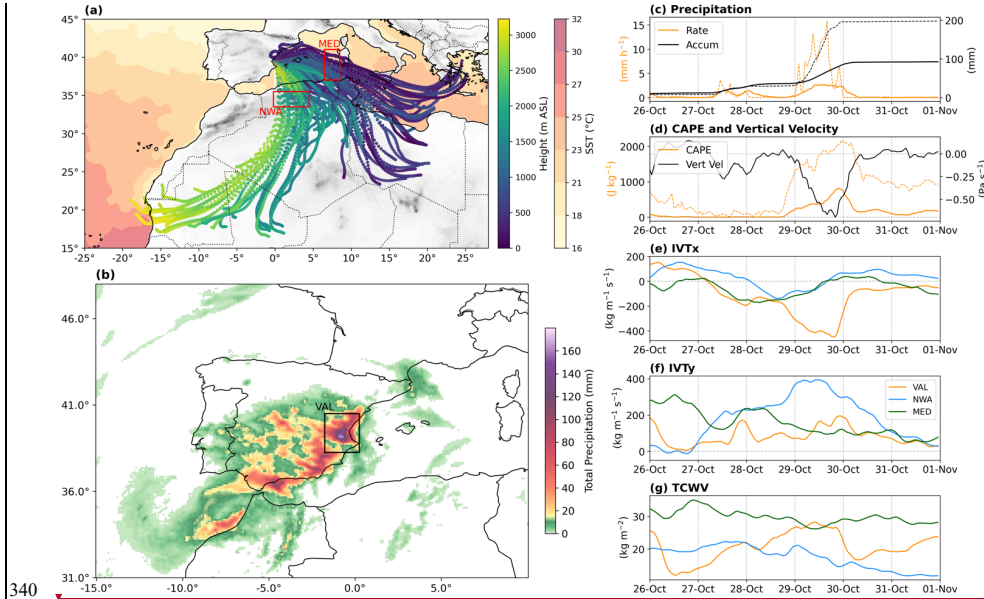
Figure 2: (a) 72-hour backward trajectories from the HYSPLIT model for air parcels arriving in Valencia at 12Z on 29 October, and 7-day mean (24-30 Oct) SSTs ( ^{\circ}\text{C} ) from NOAA OISSTv2. Red boxes indicate the Mediterranean (MED) and Northwestern Africa (NWA) boxes. (b) 24-hour accumulated precipitation on 29 October from the Factual scenario, with the Valencia (VAL) box shown in black. (c) Hourly precipitation rate (orange) and accumulated precipitation (black) over the Valencia box. Solid lines indicate the box mean, and dashed lines indicate the grid cell with the highest accumulation. Accumulated precipitation is computed starting at 00 UTC on 24 October. (d) Vertically-averaged vertical velocity (black) and CAPE (orange) over the Valencia box. Solid lines show the box mean, and the orange dashed line indicates the highest hourly CAPE within the box. (e) Hourly mean zonal IVT (IVTx) over VAL (orange), NWA (blue), and MED (green). (f) As in (e), but for meridional IVT (IVTy). (g) As in (f), but for TCWV.
