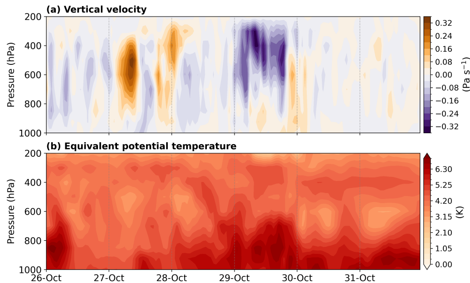
475 Figure 5: Time-pressure evolution of Factual – Counterfactual differences in (a) vertical velocity ( \Omega , in Pa/s) and (b) equivalent potential temperature ( \theta_e , in K) over the VAL region.
