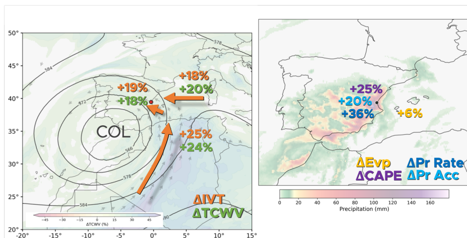
600 Figure 8: Schematic figure of the relative changes between Factual and Counterfactual scenarios. Total column water vapor (ATCWV, in green) and integrated water vapour transport (ΔIVT, in orange) on the left. Precipitation rate (ΔPr Rate, in dark blue), accumulated precipitation (ΔPr Acc, in light blue), evaporation (ΔEvp, in yellow) and convective available potential energy (ΔCAPE, in purple) on the right.
