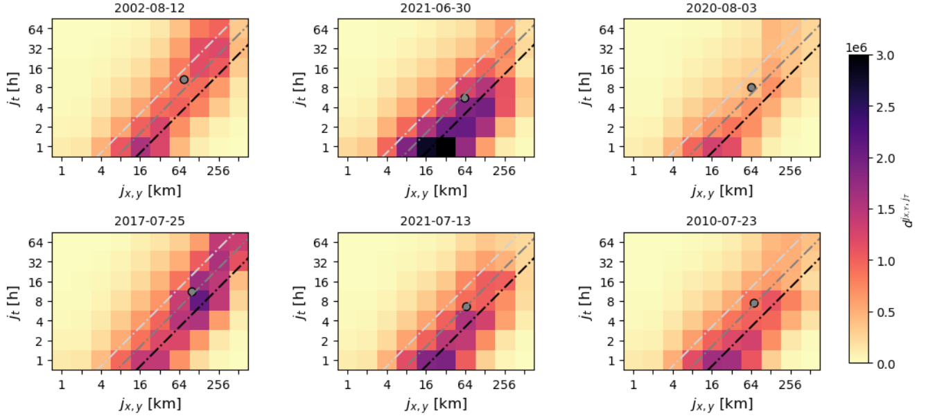
Figure 4. Wavelet spectrum (Eq. 9) of the top six precipitation events identified Sect. 3. The white lightgray , gray and lightgray -black solid lines denote a characteristic speed of 5km/h, 10km/h and 20km/h. The centre of mass (Eq. 10) is indicated by a gray dot.
