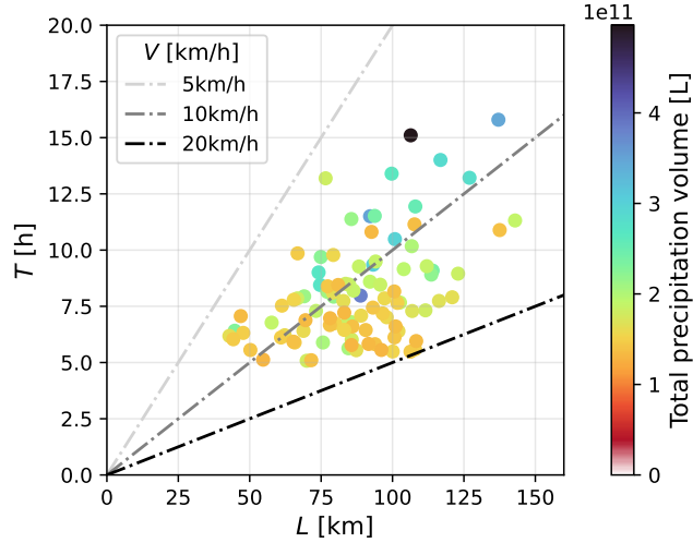
Figure 5. Scatter plot of the characteristic length L and characteristic time T (Eq. 10), for the top 100 precipitation events identified in Sect. 3. Point color colour indicates total precipitation volume similar to Fig. 2. Straight lines indicate a characteristic speed V of 5 km/h (light gray), 10 km/h (gray) and 20 km/h (black).
