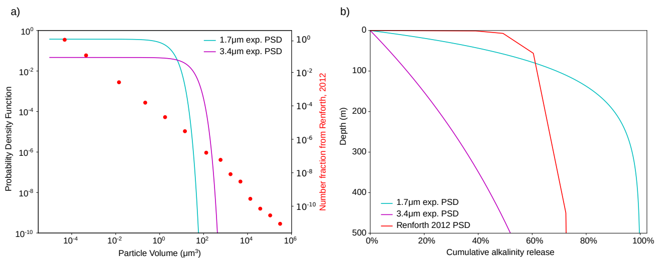
Figure A7. (a) Discretized sieve-based particle size distribution from Renforth (2012) compared to the exponential particle size distributions from this study for mean particle volumes corresponding to radii volume diameters of 0.8617 \mu\text{m} and 1.7234 \mu\text{m} , respectively. The PSDs are plotted on a log-log scale as that from Renforth (2012) spans many orders of magnitudes in particle volume, with its near-linear evolution resembling a heavy-tailed power-law distribution. (b) Cumulative alkalinity release over the upper 500 m assuming T=25^\circ\text{C} and \text{pH}=8.2 .
