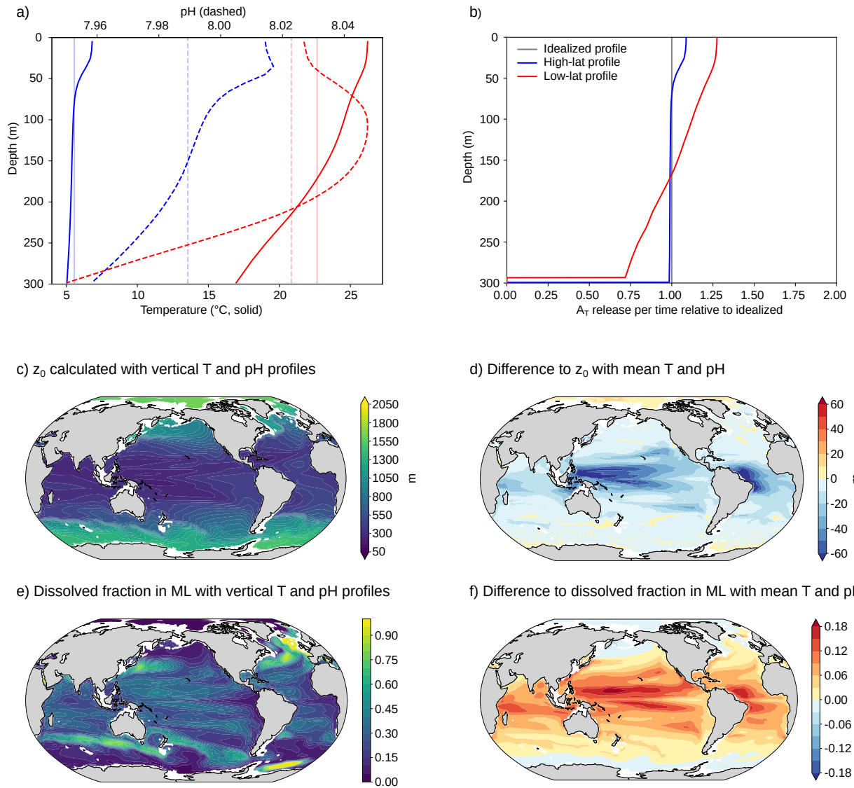
Figure A6. Numerical simulation used to test the influence of variations in temperature and pH along the water column on the alkalinity release profile. Panel a shows two exemplary temporal mean profiles, one from the Southern Ocean ( -57.5^\circ\text{N} , 177.5^\circ\text{E} ) in blue and one from the subtropical Atlantic ( 20.9^\circ\text{N} , -58.5^\circ\text{E} ) in red. Light vertical lines in panel a show mean temperature and pH over the upper 300 m. Under the idealized dissolution profile approach (Section 2.3), particles with a radius-diameter of 0.861.7 \mu\text{m} in the subtropical Atlantic column and particles with a radius-diameter of 1.292.6 \mu\text{m} in the Southern Ocean column both penetrate down to 300 m ( reference-penetration depth z_0 of 300 m). The numerical alkalinity release profiles with explicit vertical temperature and pH profiles are shown in panel b. Panel c shows the reference-penetration depth with explicit temperature and pH profiles for particles with radius r=1.29 \mu diameter d=2.6 \mu\text{m} globally, and panel d shows the difference to the reference-penetration depth assuming mean temperature and pH (Figure 2e). Regions where the water column is shallower than the reference-penetration depth are left blank as they do not allow a direct comparison. Panel e shows the fraction dissolved in the annual maximum mixed layer with explicit temperature and pH profiles and panel f shows the difference to the dissolved fraction assuming mean temperature and pH (Figure 2h).
