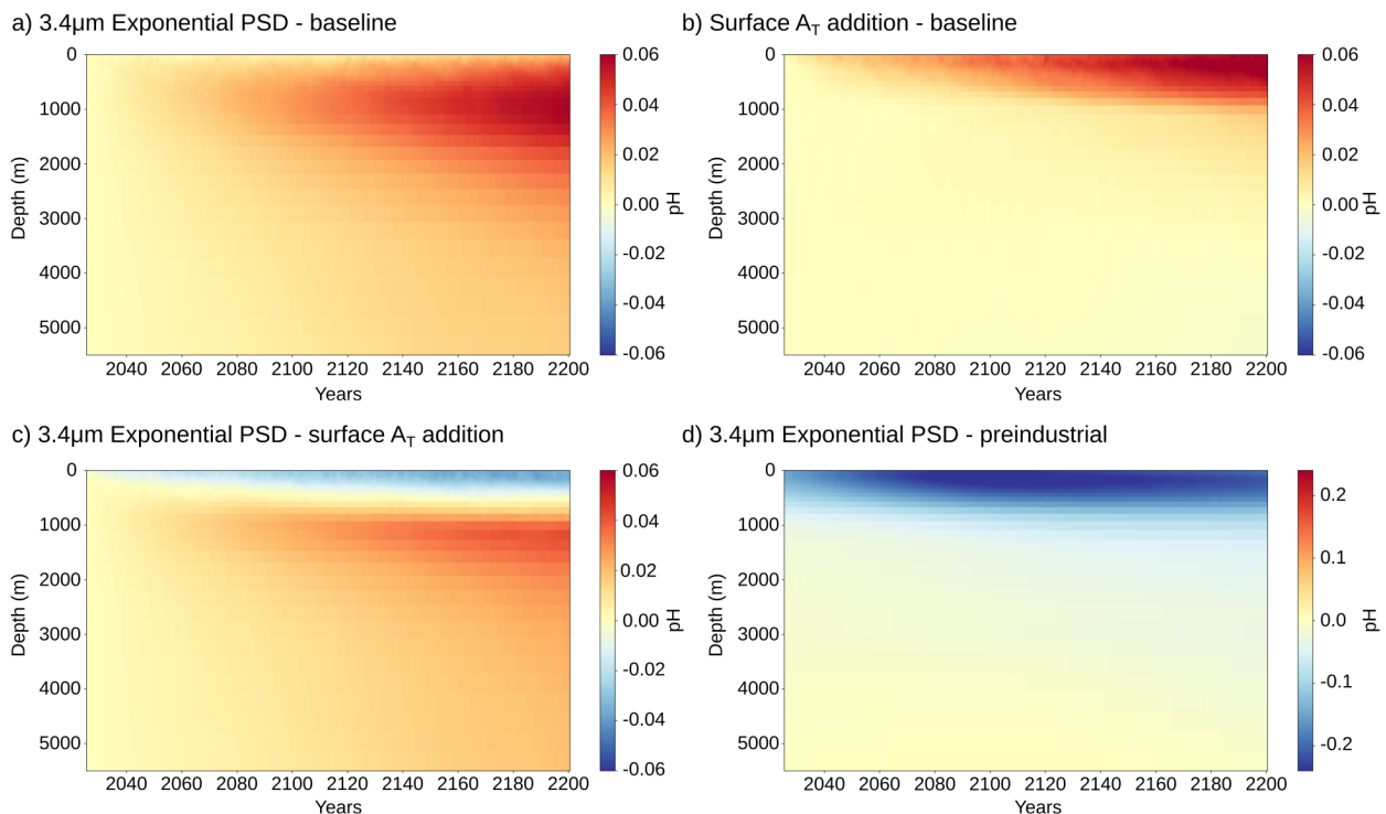
Figure A8. Global-mean pH difference along the water column between OAE and the baseline simulation without OAE, for (a) the exponential PSD with reference radius mean volume diameter of 1.723.4 \mu\text{m} and (b) surface alkalinity addition. The pH change is averaged over the period 2026-2200. Panel c shows the pH difference between the exponential PSD with reference radius mean volume diameter of 1.723.4 \mu\text{m} and surface alkalinity addition. Panel d shows the total change in pH from the baseline \text{CO}_2 emissions and OAE with the exponential PSD relative to the pre-industrial state.
