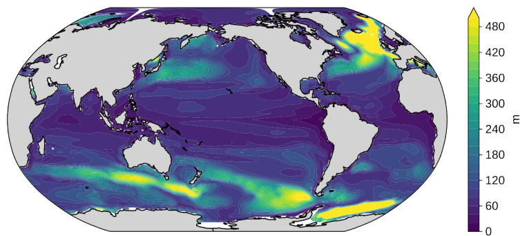
Figure A4. Annual maximum mixed layer depth in the GFDL-ESM2M GFDL-ESM2M model. Mixed layer depth is defined as the depth where density increases by 0.03 \text{ kg m}^{-3} relative to the surface. It is calculated as the annual maximum of monthly mixed layer depth, averaged over the period 2016-2025 and over five ensemble members. Global average annual maximum mixed layer depth is 123 m.
