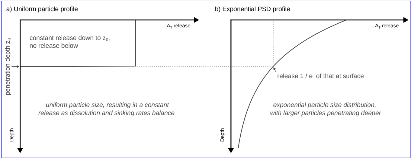
Figure 1. Alkalinity release profiles for a) uniform particles (section 2.1.2) and b) for particles with an exponential particle size distribution (section 2.1.3).
