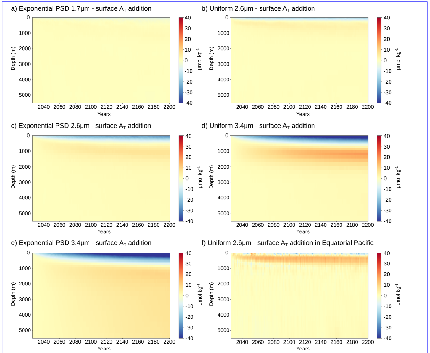
Figure A5. Global mean vertical distribution of additional alkalinity relative to that for surface alkalinity addition over time for the uniform and exponential PSDs with mean volume diameters of 1.7\mu\text{m} , 2.6\mu\text{m} , and 3.4\mu\text{m} (panels a-e). We do not show the alkalinity difference for the uniform particle profile with d = 1.7\mu\text{m} , as differences are minor. Panel f shows the alkalinity difference in the eastern and central equatorial Pacific ( -8^\circ\text{N} to 8^\circ\text{N} , -190^\circ\text{E} to -85^\circ\text{E} ) for the uniform case with d = 2.6\mu\text{m} .
