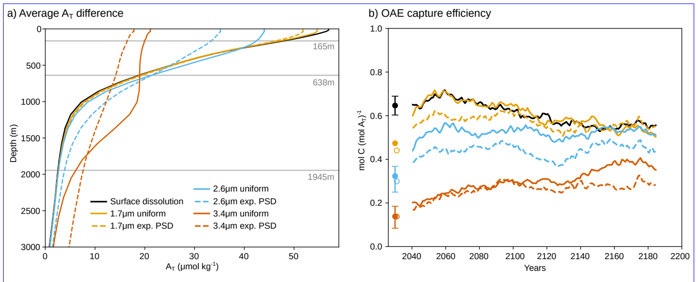
Figure 3. (a) Global mean difference in total alkalinity between the OAE simulations (surface dissolution and uniform as well as exponentially distributed particle size distributions) and the baseline simulation without OAE, averaged over 2026-2200. The horizontal gray lines indicate the global mean penetration depths z_0 for the three particle diameters 1.7 \mu\text{m} , 2.6 \mu\text{m} , and 3.4 \mu\text{m} . (b) The OAE efficiency for these simulations over time, defined as the number of moles of additional carbon uptake in the OAE simulations divided by the number of moles alkalinity added. The lines show 31-year running means. The dots indicate averages over the first 10 years of the experiment, with open dots for the PSD experiments. For surface dissolution and the 2.6 \mu\text{m} and 3.4 \mu\text{m} uniform cases, the five-member ensemble ranges and ensemble means shown.
