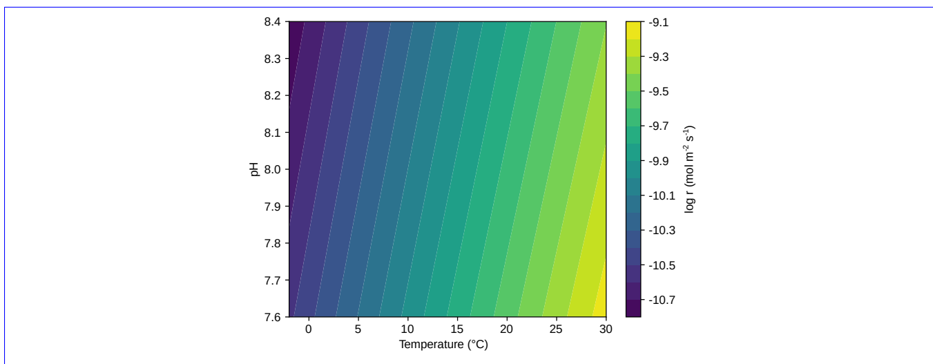
Figure A3. The base-10 logarithm of the area-normalized dissolution rate of forsterite from Rimstidt et al. (2012) as a function of temperature and pH.
