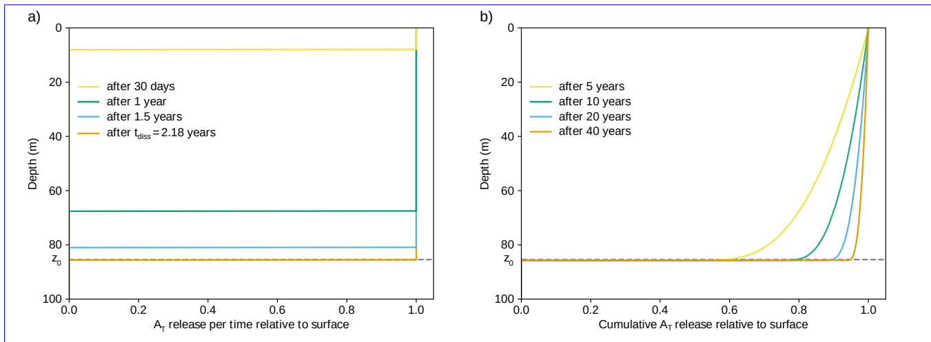
Figure A2. Numerical simulation used to validate the analytical uniform particle flux profile. Particles of diameter d = 1.7 \mu\text{m} are continuously added at the surface ( T = 25^\circ\text{C} , \text{pH} = 8.2 ) and sink through a vertical grid of 0.1 \text{ m} resolution with a timestep of 1 \text{ h} . (a) The alkalinity release in each time step at different time points. The release is constant with depth but only reaches down to the depth the first particle reached. At the dissolution time t_{\text{diss}} and afterwards, the alkalinity release profile extends down to the penetration depth z_0 . (b) The cumulative alkalinity release is not strictly rectangular, since particles that were released less than t_{\text{diss}} = 2.18 years before have not reached z_0 yet and have only released alkalinity at shallower depths. For longer time periods since the start of the experiment, these particles matter relatively less, such that the cumulative alkalinity release is eventually also approximately rectangular. For example, the cumulative alkalinity released at depth z_0 is 95 % of that at the surface after 40 years.
