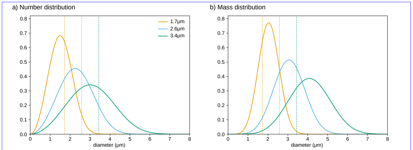
Figure A1. Probability density functions as a function of particle diameter for the exponential PSDs analyzed in this study. Panel a shows the distribution of particle number across diameters (a Rosin-Rammler distribution with shape 3 and scale given by the mean-volume diameter d ) and panel b displays the distribution of particle mass (a generalized gamma distribution with shape parameters p=3 and d=6 and scale d ). Vertical dotted lines display the mean volume diameters d of the three distributions.
