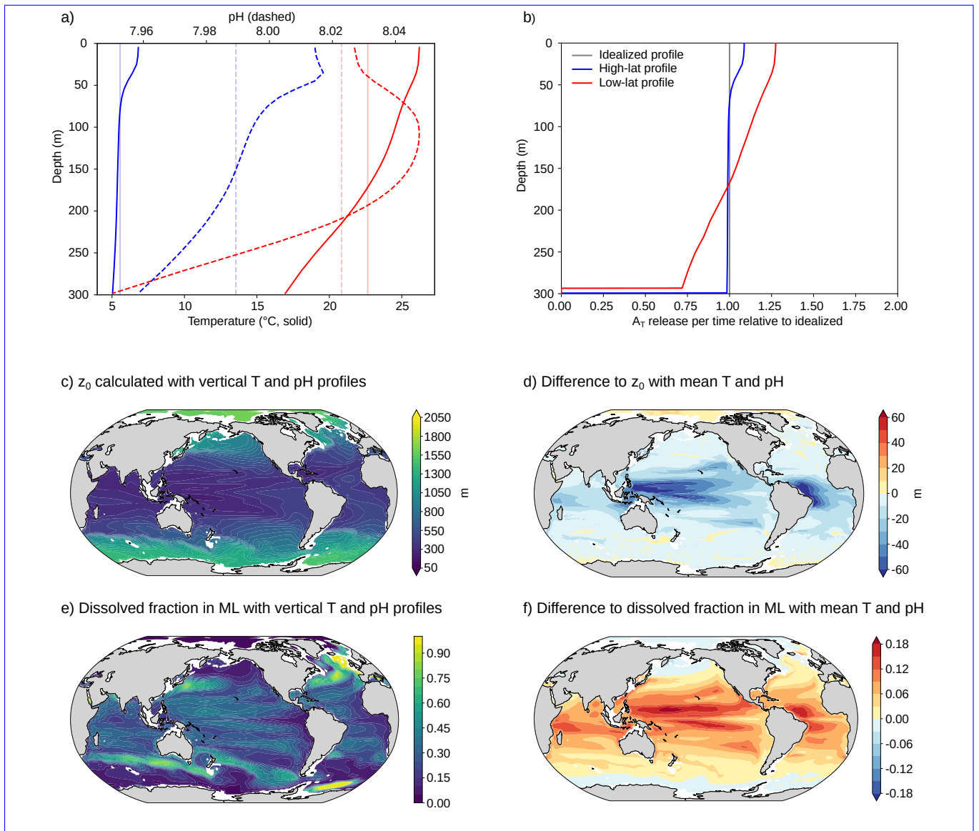
Figure A6. Numerical simulation used to test the influence of variations in temperature and pH on the total scale along the water column on the alkalinity release profile. Panel a shows two exemplary temporal mean profiles, one from the Southern Ocean ( -57.5^\circ\text{N} , 177.5^\circ\text{E} ) in blue and one from the subtropical Atlantic ( 20.9^\circ\text{N} , -58.5^\circ\text{E} ) in red. Light vertical lines in panel a show mean temperature and pH over the upper 300 m. Under the idealized dissolution profile approach (Section 2.3), particles with a diameter of 1.7\ \mu\text{m} in the subtropical Atlantic column and particles with a diameter of 2.6\ \mu\text{m} in the Southern Ocean column both penetrate down to 300 m (penetration depth z_0 of 300 m). The numerical alkalinity release profiles with explicit vertical temperature and pH profiles are shown in panel b. Panel c shows the penetration depth with explicit temperature and pH profiles for particles with diameter d = 2.6\ \mu\text{m} globally, and panel d shows the difference to the penetration depth assuming mean temperature and pH (Figure 2e). Regions where the water column is shallower than the penetration depth are left blank as they do not allow a direct comparison. Panel e shows the fraction dissolved in the annual maximum mixed layer with explicit temperature and pH profiles and panel f shows the difference to the dissolved fraction assuming mean temperature and pH (Figure 2h).
