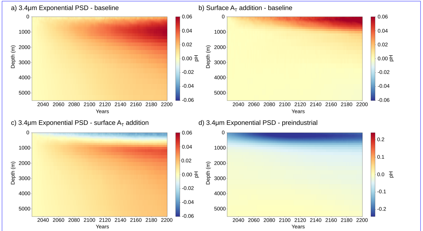
Figure A8. Global-mean pH difference along the water column between OAE and the baseline simulation without OAE, for (a) the exponential PSD with mean volume diameter of 3.4 \mu\text{m} and (b) surface alkalinity addition. The pH change is on the total scale and averaged over the period 2026-2200. Panel c shows the pH difference between the exponential PSD with mean volume diameter of 3.4 \mu\text{m} and surface alkalinity addition. Panel d shows the total change in pH from the baseline \text{CO}_2 emissions and OAE with the exponential PSD relative to the pre-industrial state.
