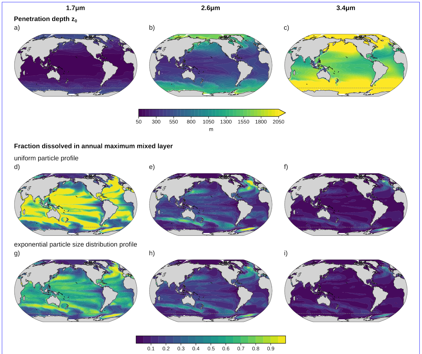
Figure 2. Regional variation in penetration depth and mixed layer alkalinity release for particle diameters d = 1.7 \mu\text{m} (left column), d = 2.6 \mu\text{m} (middle column), and d = 3.4 \mu\text{m} (right column). (a-c) Penetration depth determined with temperature and pH data from GFDL ESM2M over the period 2016-2025 (see Sections 2.3 and 2.4). The fraction of alkalinity released above the annual maximum mixed layer depth ( \chi ) for uniform particle profiles are shown in panels d-f and those for exponential particle size distribution profiles in panels g-i for each penetration depth. The gray dashed lines enclose the region between 60^\circ\text{S} and 70^\circ\text{N} , where alkaline minerals are added to the surface ocean in this study.
