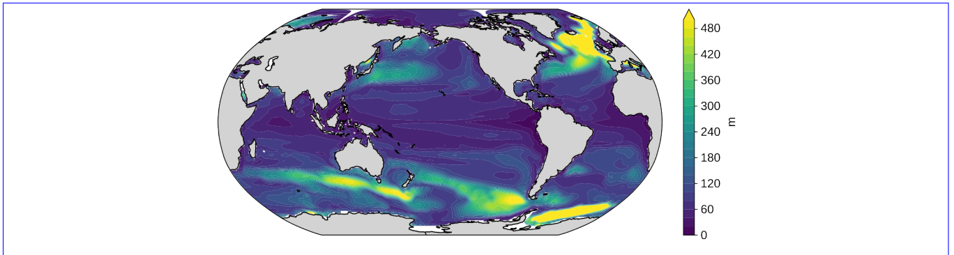
Figure A4. Annual maximum mixed layer depth in the GFDL ESM2M model. Mixed layer depth is defined as the depth where density increases by 0.03 \text{ kg m}^{-3} relative to the surface. It is calculated as the annual maximum of monthly mixed layer depth, averaged over the period 2016-2025 and over five ensemble members. Global average annual maximum mixed layer depth is 123 m.
