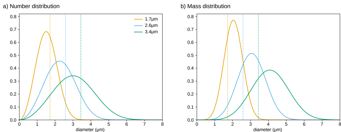
Figure A1: Probability density functions for the exponential PSDs analyzed in this study as a function of particle diameter. Panel a shows the distribution of particle number across diameters (a Rosin-Rammler distribution with shape 3 and scale given by the mean-volume diameter d ) and panel b displays the distribution of particle mass (a generalized gamma distribution with shape parameters p=3 and d=6 and scale d ). Vertical dotted lines display the mean volume diameters d of the three distributions.
