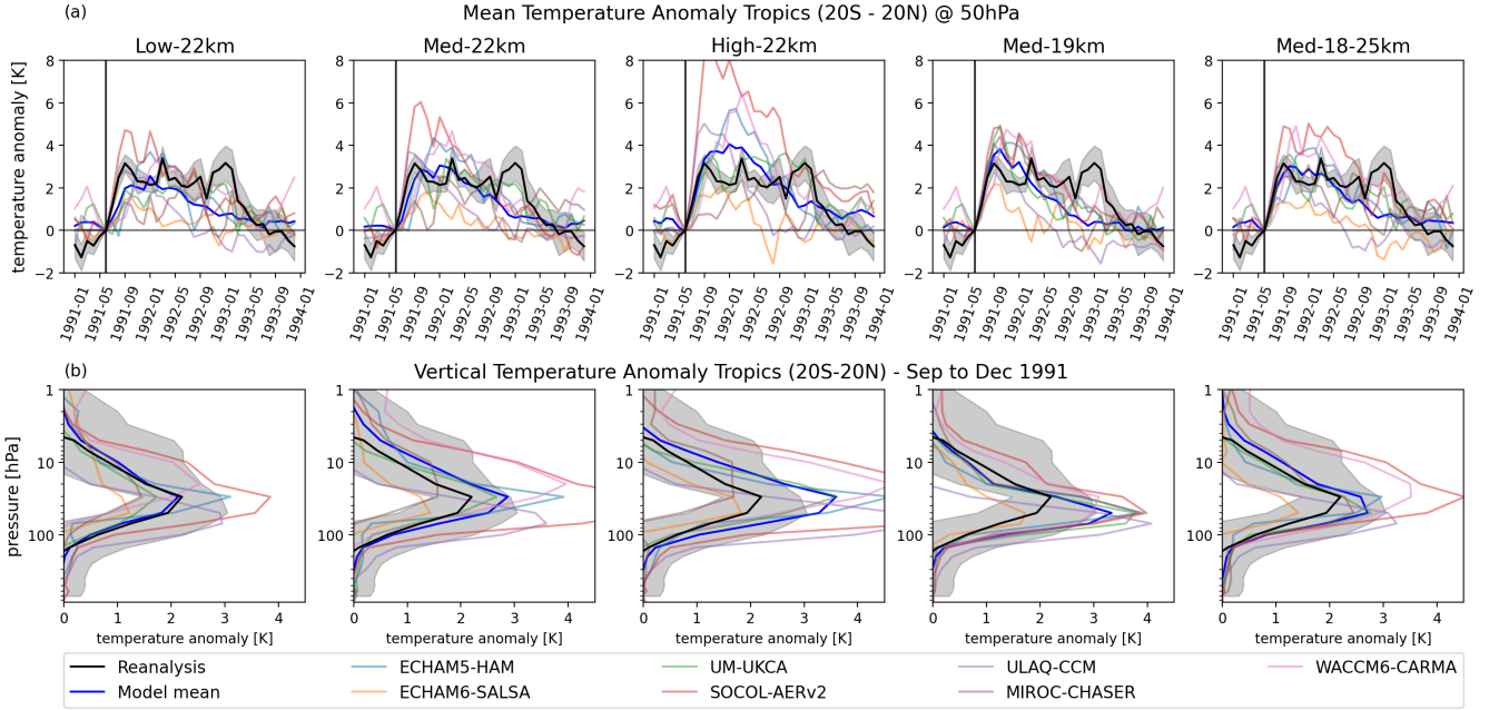
Figure 1. Time evolution of the observed (multi-reanalysis mean) and model-derived tropical mean temperature anomaly normalized to June 1991 (a) and tropical vertical temperature anomaly for the period September to December 1991 (b). In all panels, the multi-model mean is provided as a blue bold line, and the grey shading indicates the \pm 3\sigma confidence bound for the reanalysis mean (black, bold).
