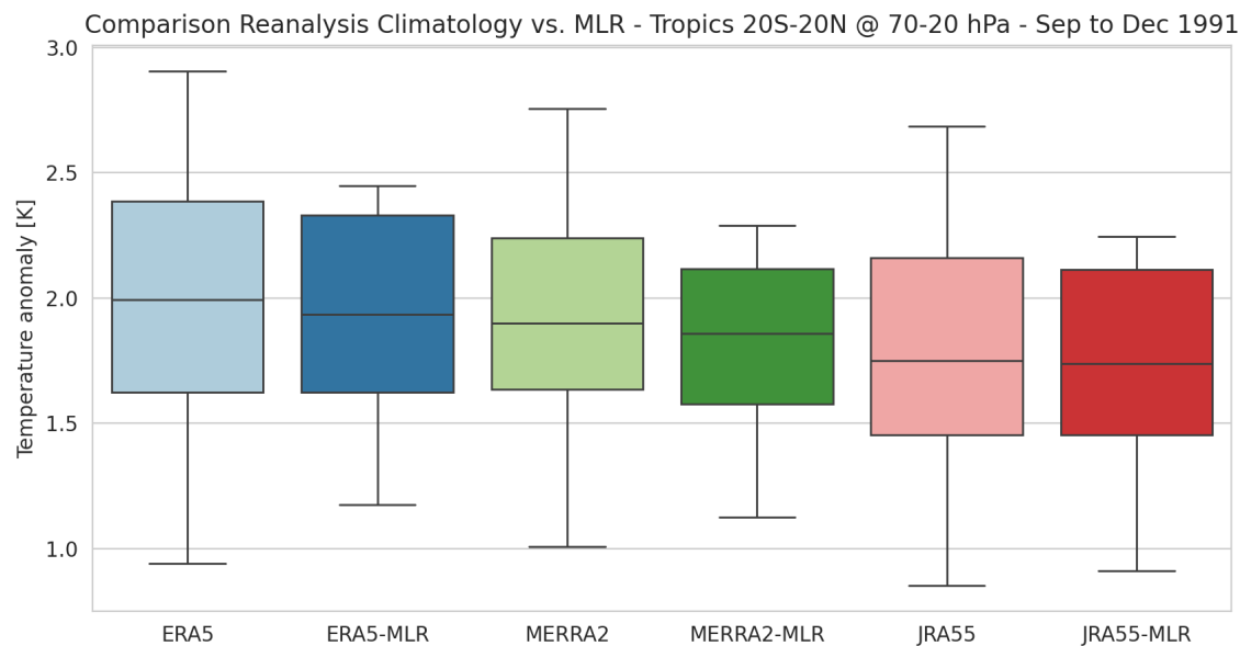
Figure A1. Temperature anomaly distribution of reanalysis data before (bright colours) and after MLR (dark colours) in the tropics between 70 and 20 hPa in the period from September to December 1991. All calculations use 1980-2000 as the base period.
