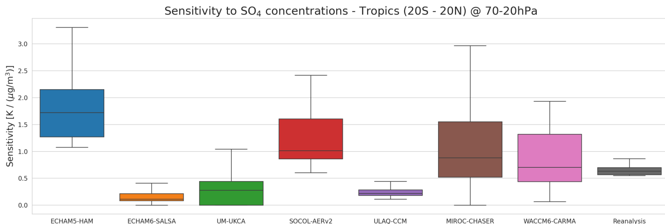
Figure 5. Stratospheric temperature sensitivity to \text{SO}_4 absorptive-heating of the ISA-MIP models and reanalysis in the tropics ( 20^\circ \text{S} - 20^\circ \text{N} ) between 70 and 20 hPa. The boxplots contain data for altitude weighted longitude - latitude pairs, obtained by regressing temperature anomalies against \text{SO}_4 concentrations over time.
