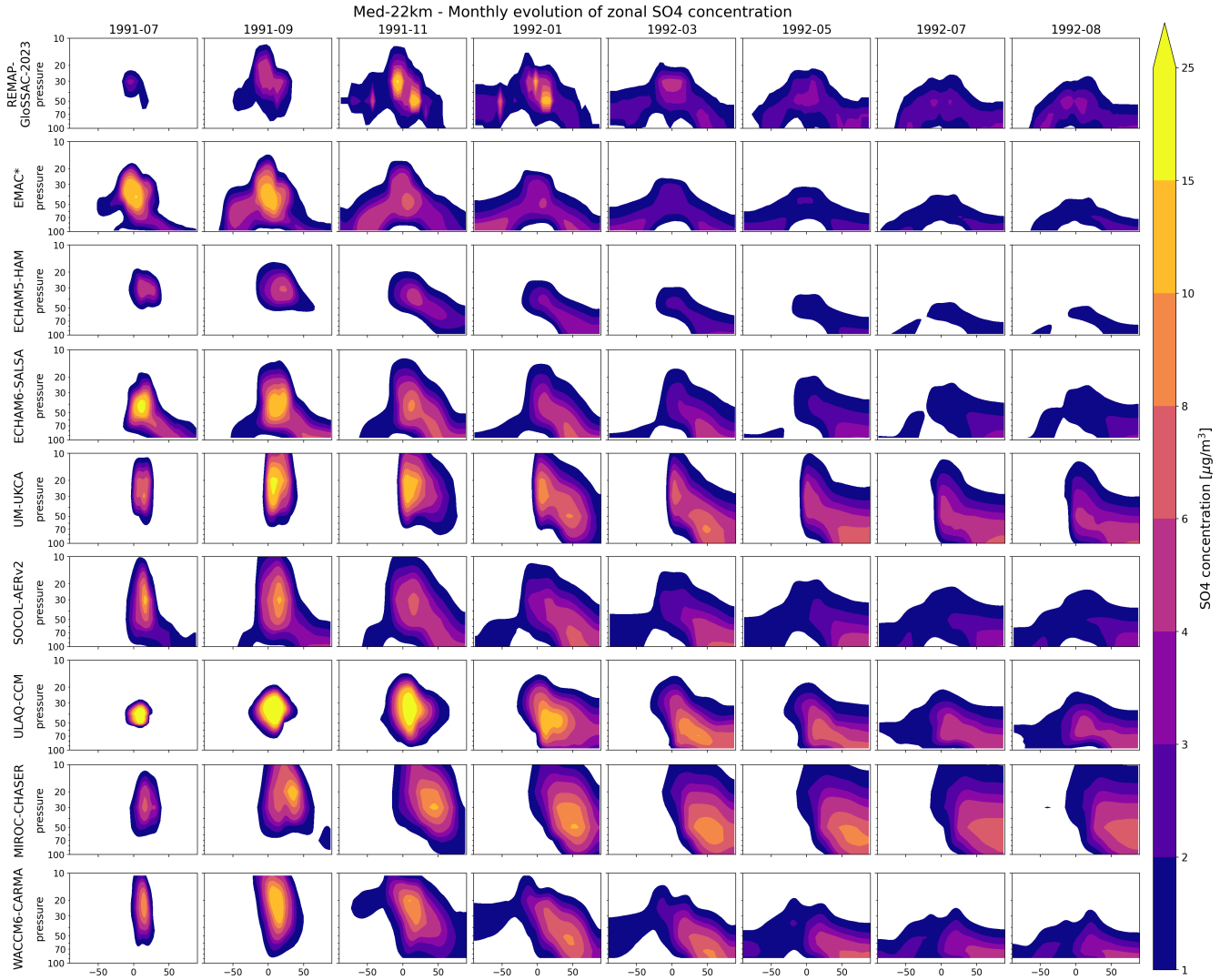
Figure 2. Vertical evolution of zonal mean \text{SO}_4 concentrations in experiment Med-22km for individual models, from July 1991 to August 1992 (bi-monthly; columns) in comparison with REMAP-GloSSAC-2023 observations (first row). Note, EMAC is flagged with * as it did not fully adhere to the ISA-MIP protocol, see section 2.2.8.
