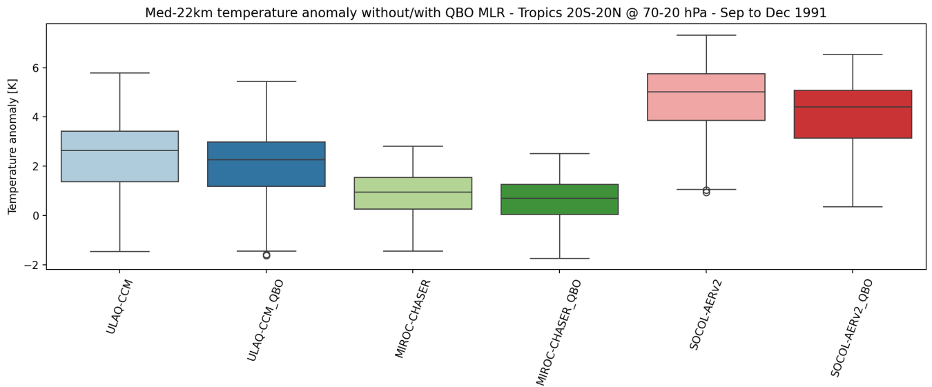
Figure A2. Temperature anomalies in the Med-22km experiment for selected ISA-MIP models with QBO effects included or regressed out. For ULAQ-CCM, MIROC-CHASER and SOCOL-AERv2 temperature anomalies are derived by using the Control runs as reference. For ULAQ-CCM_QBO, MIROC-CHASER_QBO and SOCOL-AERv2_QBO the QBO signal was removed in experiment and Control, using the wind field at 30 and 50 hPa before anomalies were derived.
