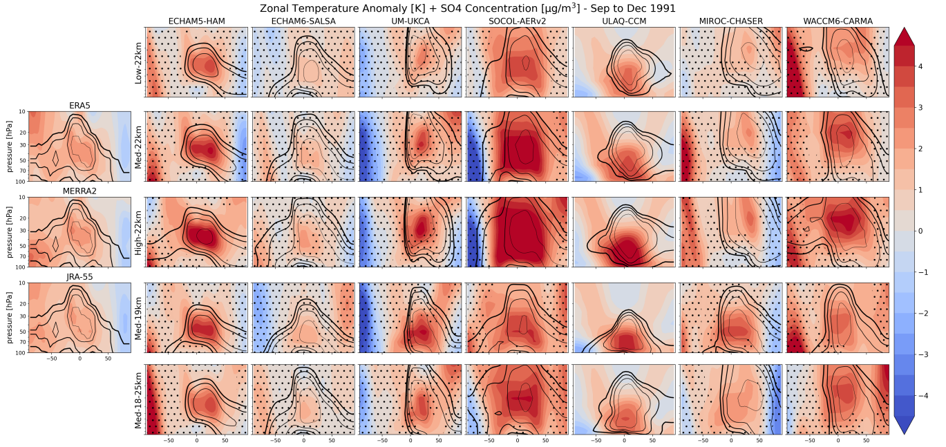
Figure A5. Vertical zonal temperature anomaly for all experiments and models for the period September to December 1991. In all panels: SO 4 concentrations are shown as contours (levels are 0.5, 1, 2, 5 \mu\text{g}/\text{m}^3 ), dots indicate non-significant areas (p-value > 0.05) for reanalysis and models with the exception of ULAQ-CCM where only one ensemble member is available, and the vertical lines embed the tropical region (20° S - 20° N).
