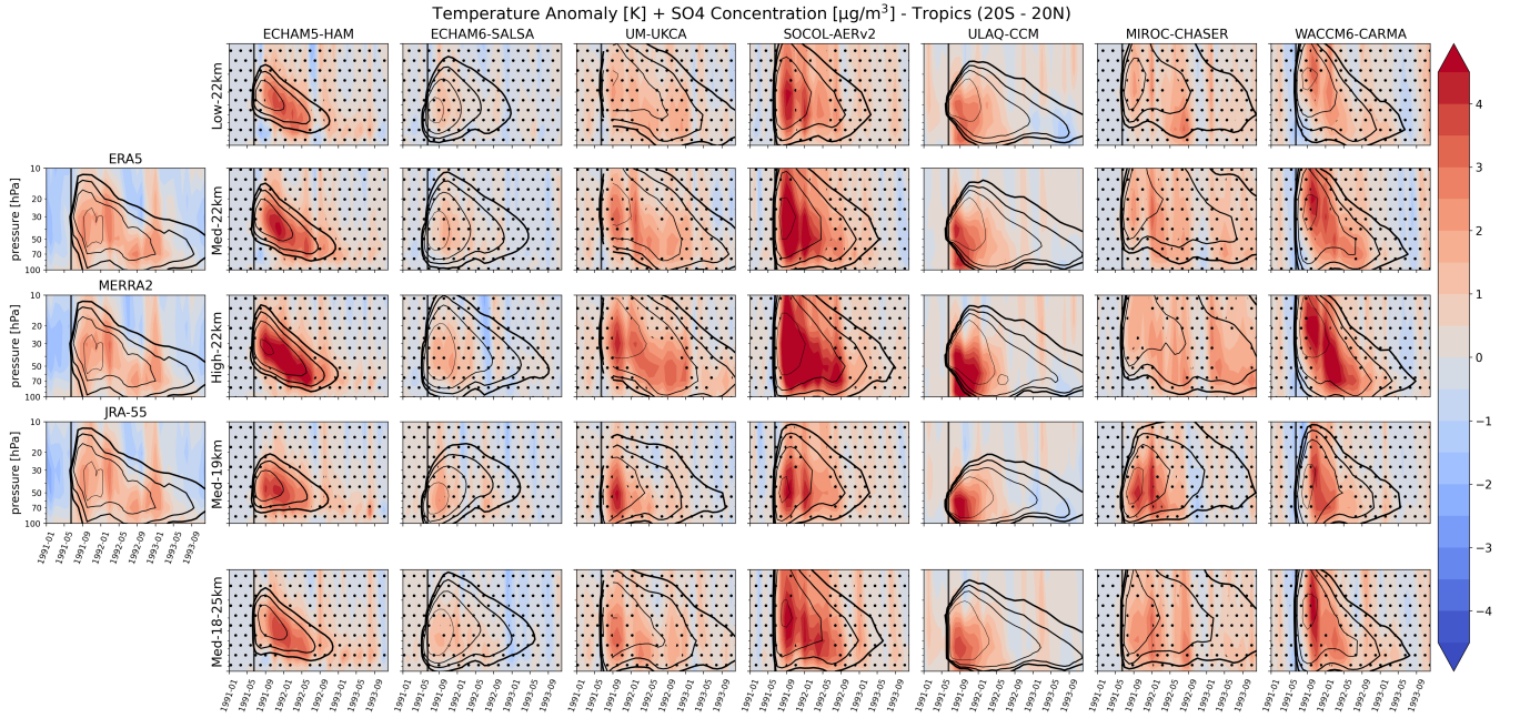
Figure A4. Vertical time evolution of the temperature anomalies for all experiments and models in the tropics ( 20^{\circ} S - 20^{\circ} N). In all panels: \text{SO}_4 concentrations are shown as contours (levels are 0.5, 1, 2, 5 \mu\text{g}/\text{m}^3 ), dots indicate non-significant areas ( p\text{-value} > 0.05 ) for reanalysis and models with the exception of ULAQ-CCM where only one ensemble member is available, and the thick black vertical line represents the Mt. Pinatubo eruption time.
