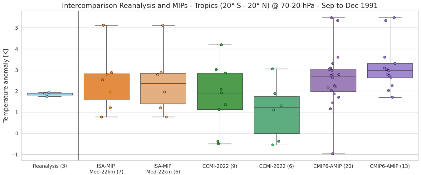
Figure 6. Temperature anomaly distributions for reanalyses (left), ISA-MIP and CCMI-2022 (center) and CMIP6-AMIP (right) in the tropics ( 20^{\circ} S - 20^{\circ} N) averaged between 70 and 20 hPa in the period September to December 1991. The number in brackets indicates the number of models used. Solid vertical line separates reanalysis from models. Light orange, light green and light purple boxplots represent models with more than one ensemble member. Individual model results are provided as dots in the same colour of the corresponding MIP/sample. For convenient reference we note the order of ISA-MIP models in descending temperature anomaly: SOCOL-AERv2, ECHAM5-HAM, WACCM6-CARMA, ULAQ-CCM, UM-UKCA, ECHAM6-SALSA, MIROC-CHASER.
