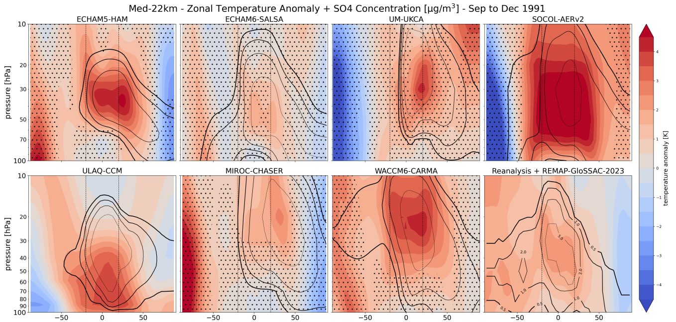
Figure 4. Vertical zonal temperature anomaly in experiment Med-22km for the period September to December 1991 for individual models. In all panels: SO 4 concentrations are shown as contours (levels are 0.5,1,2,5 \mu\text{g}/\text{m}^3 ), dots indicate non-significant areas (p-value \leq 0.05 ), and the vertical lines show embed the tropical region (20° S - 20° N). REMAP-GloSSAC-2023 SO 4 concentrations are shown as contours in the reanalysis panel.
