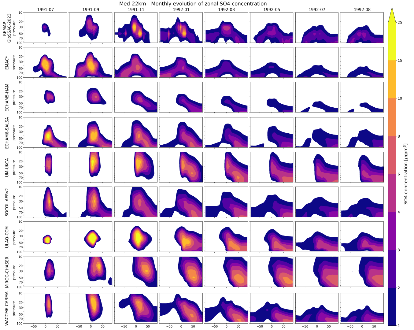
Figure 2. Vertical evolution of zonal mean SO 4 concentrations in experiment Med-22km for individual models, from July 1991 to August 1992 (bi-monthly; columns) in comparison with REMAP-GloSSAC-2023 observations (first row).
