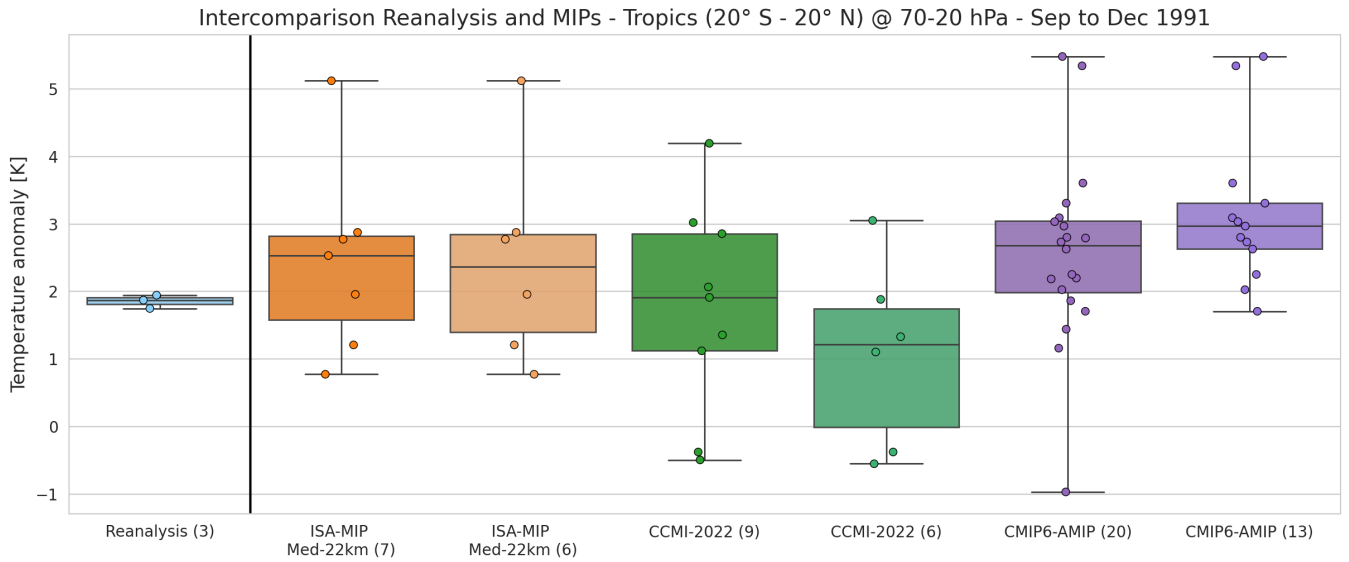
Figure 6. Temperature anomaly distributions for reanalyses (left), ISA-MIP and CCM1-2022 (center) and CMIP6-AMIP (right) in the tropics ( 20^{\circ} S - 20^{\circ} N) averaged between 70 and 20 hPa in the period September to December 1991. Number The number in brackets indicated indicates the number of models used. Solid vertical line separates reanalysis from models. Light orange, light green and light purple boxplots represent models with more than one ensemble member. Individual model results are provided as dots in the same colour of the corresponding MIP/sample. For convenient reference we note the order of ISA-MIP models in descending temperature anomaly: SOCOL-AERv2, ECHAM5-HAM, ULAQ-CCM , WACCM6-CARMA, ULAQ-CCM , UM-UKCA, ECHAM6-SALSA, MIROC-CHASER.
