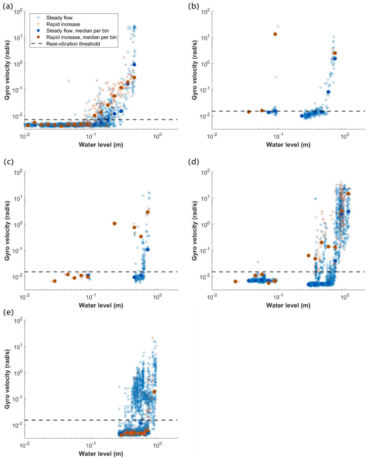
Figure 4. The variation of smartrock gyro velocity with water level for rapid rise time windows (red) and steady time windows (blue). (a) Nahal Anim; (b-e) Nahal Yatir, events Y1-4. Dashed black line indicates the gyro threshold of average rest-vibration.
