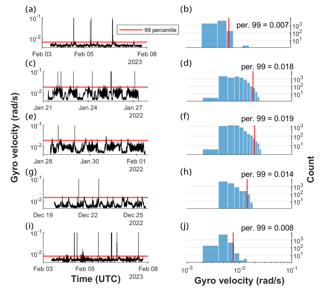
210 Figure 3. Pre-flood gyro velocity time series (left side column) and the corresponding gyro velocity histogram (right side column). The red line represents the 99 th percentile value for each pre-flood period. (a-b) Nahal Anim, event A1; (c-d) Nahal Yatir, event Y1; (e-f) Nahal Yatir, event Y2; (g-h) Nahal Yatir, event Y3 (i-j) Nahal Yatir, event Y4.
