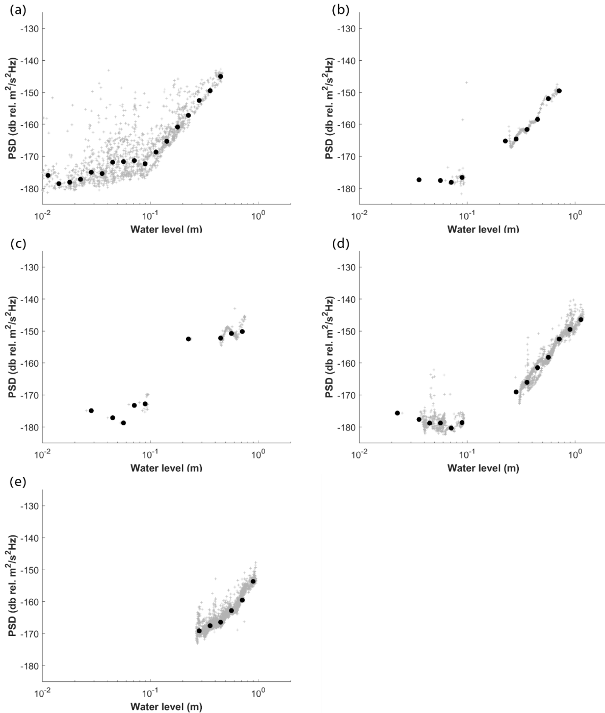
Figure 8. PSD against water depth during event A1, using the 35-60 Hz frequency band(a); and Y 1-4, respectively using the 40–65, 60–85, 50–75, and 30–55 Hz frequency bands (b-e). Data points (grey crosses) are logarithmically binned (black circles) by water depth, with an interval of 2 dB relative to water level. PSD data for the water depth range of 0.10–0.25 m is not shown in (b-e), as it corresponds to the very slow recession phase of this flow event, and no comparable rapid rise gyro data exist for this range.
