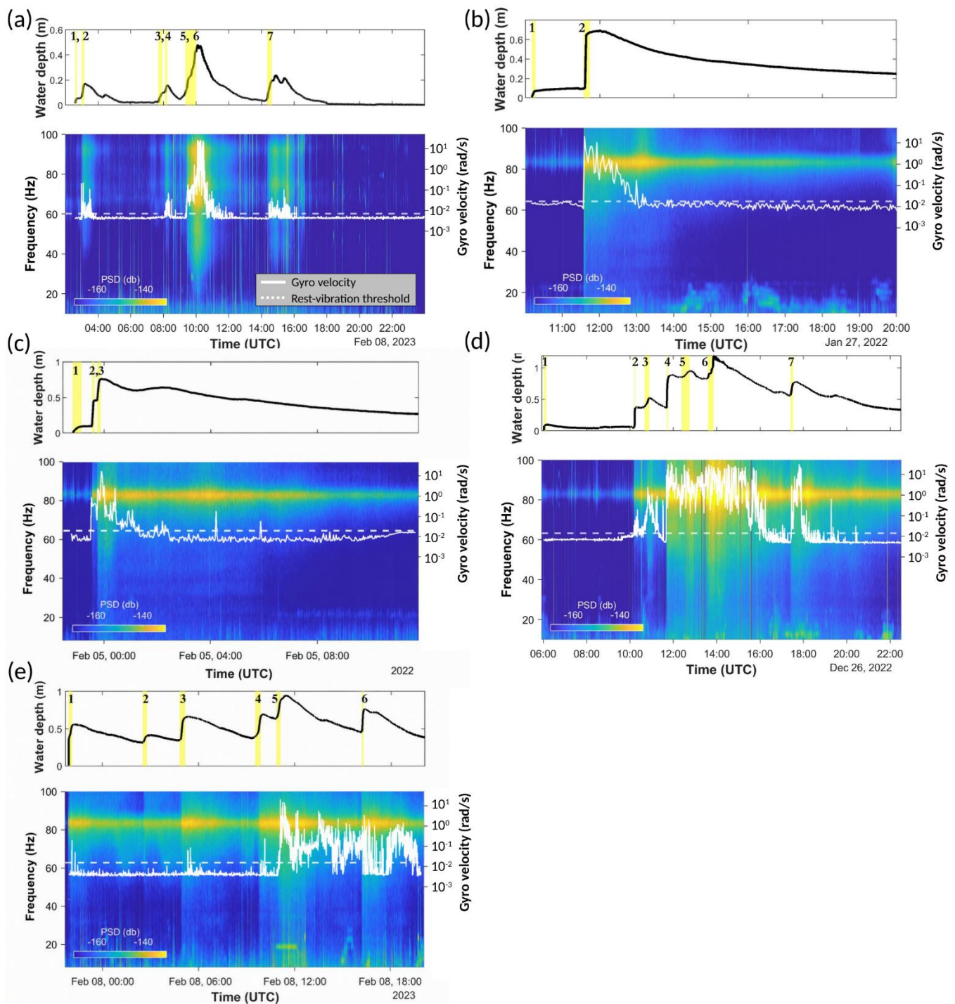
190 Figure 2. Comprehensive data from the A1 (a) and the Y1-4 (b-e) flow events. The upper panels display water stage hydrographs, with yellow-shaded areas indicating intervals of rapid increase of stage. The lower panels present the spectrograms (left y-axis) alongside the gyro velocities of the smarttracks (right y-axis). The smarttrack data are represented by a solid white line, with the rest-to-vibration threshold indicated by a dashed white line.
