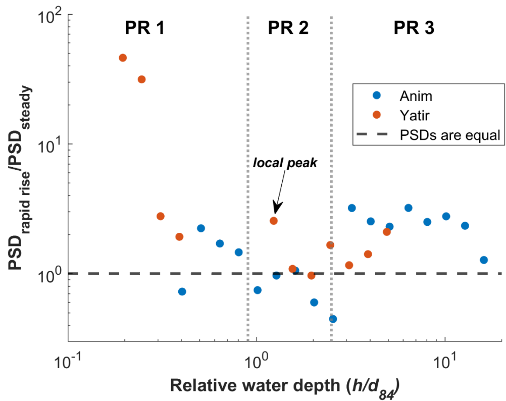
335 Figure 10. PSD ratio against relative water depth ( h/d_{84} ) for the single-monitored Nahal Anim event A1 (blue circles) and for Nahal Yatir, events Y1- Y 4 (red circles). Dashed vertical lines indicate the transitions between stages.
