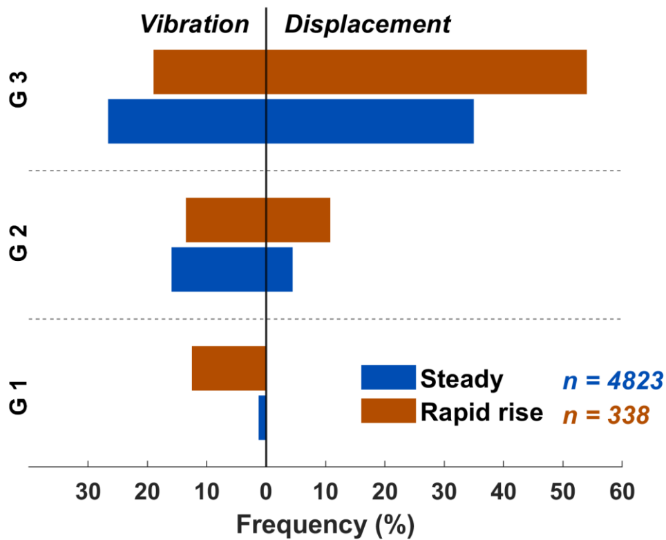
Figure 6. Distribution of smartrock motion during rapid stage-rise and quasi -steady flow conditions in Nahal Yatir. Motion is categorized-classified by motion mode (vibration, left; displacement, right) and into-vibration (left) and displacement (right) according across to the three defined gyro-based stages (G1-3). Frequencies represent the proportion of measurements within in each combination category relative to the total number of measurements, shown separately for rapid stage-rise (red) and steady flow (blue) conditions.
