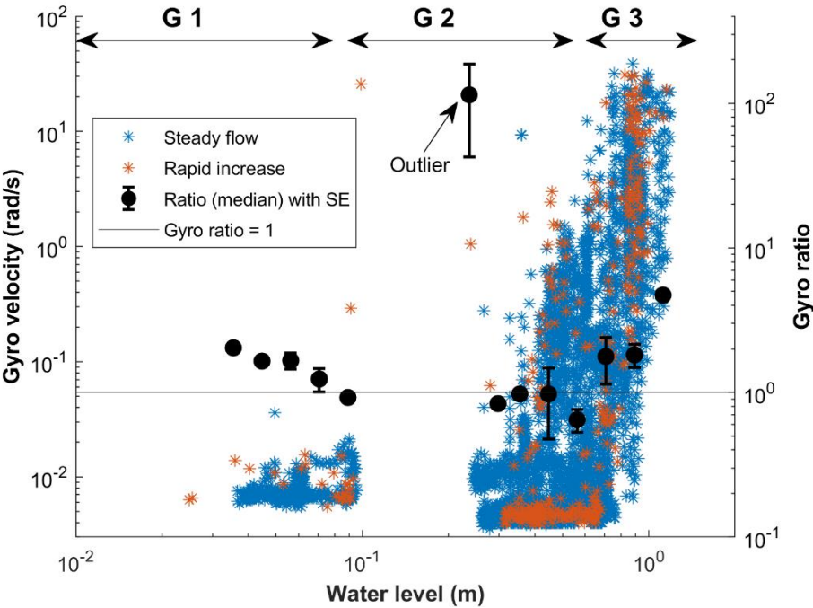
Figure 5. Gyro velocity (left ordinate) and gyro velocity ratio (right ordinate) against water level from Nahal Yatir (events Y1-4 ). The ratio points represent the median gyro velocity between rapid increase of stage and steady flow conditions, calculated for each water level interval. Based on the ratio points the data is categorized into three distinct gyro-based stages ( G1-3 ; black arrows). The horizontal line represents a gyro velocity ratio of 1, indicating equal median velocities during rapid rise and steady flow conditions. Gyro data for the water depth range of 0.0810-0.25 m is not shown, as this range corresponds to the very slow recession phase, where no comparable rapid stage rise gyro data exists.
