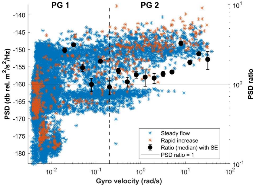
345 Figure 11. The variation of PSD (left ordinate) and PSD ratio (right ordinate) with gyro velocity for Y1–4. The right ordinate represents the ratio of median PSD values between rapid increase of stage and steady flow conditions for each water level interval. Dashed line indicates transition between two stages PSD-gyro stages (PG1 and PG2) . The horizontal line indicates a ratio of 1, denoting identical seismic energy for a given gyro velocity during rapid rise and steady flow conditions. The seismic frequencies used here are those described in Sect. 3.3.
