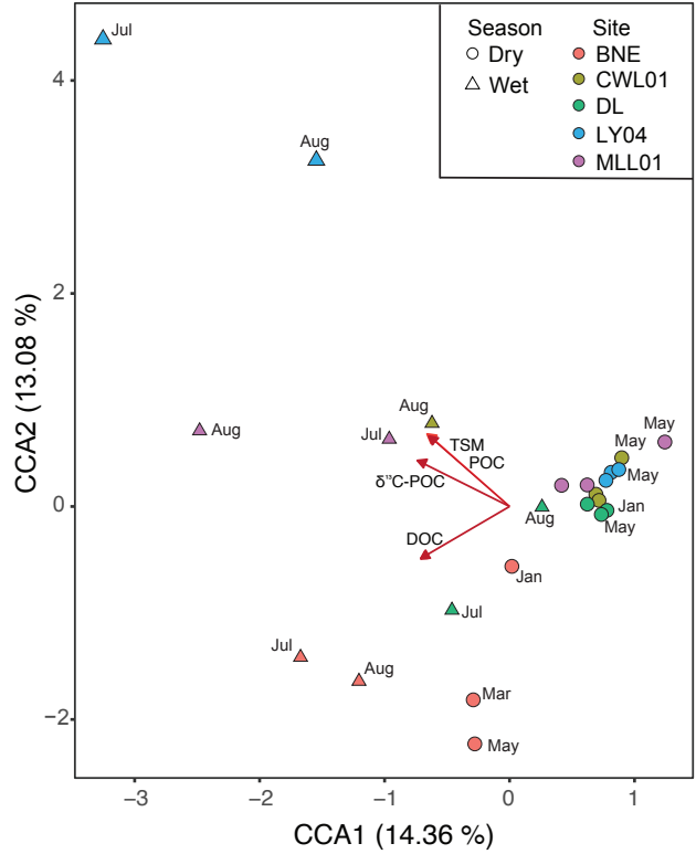
424 Figure 5. Canonical correspondence analysis (CCA) ordination of microbial community composition of 16S rRNA gene 425 amplicons (ASV proportion). Significant environmental vectors (envfit, 9999 permutations, p < 0.05 ) are shown as solid arrows: 426 TSM ( r^2 = 0.94 , p = 0.006 ), POC ( r^2 = 0.96 , p = 0.007 ), DOC ( r^2 = 0.62 , p = 0.011 ), and \delta^{13}\text{C} -POC ( r^2 = 0.65 , p = 0.035 ). Symbols 427 indicate site (color) and season (circle = dry, triangle = wet).
