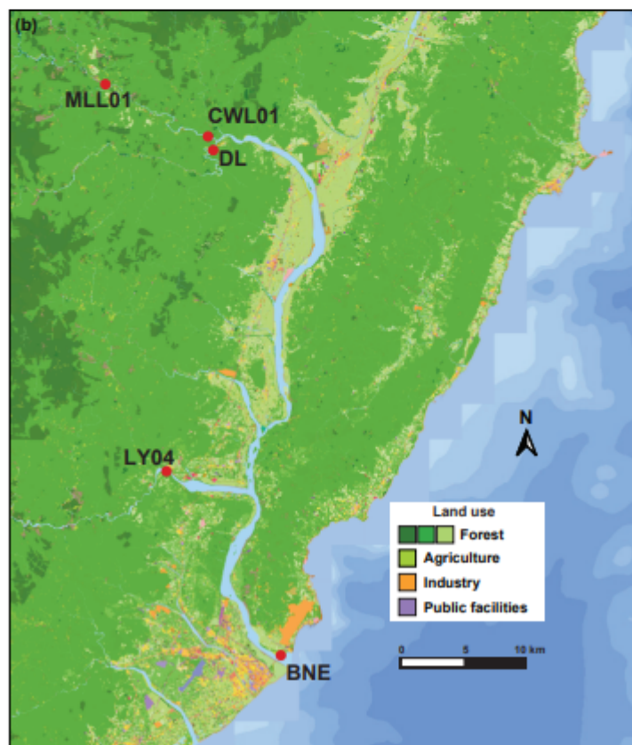
Figure 1: (a) Topographic map of the Beinan River catchment (eastern Taiwan) with sampling sites marked in red. (b) Land use and land cover of the lower Beinan catchment, adopted from the National Land Use Investigation dataset (National Land Surveying and Mapping Center, Ministry of the Interior, Taiwan).
