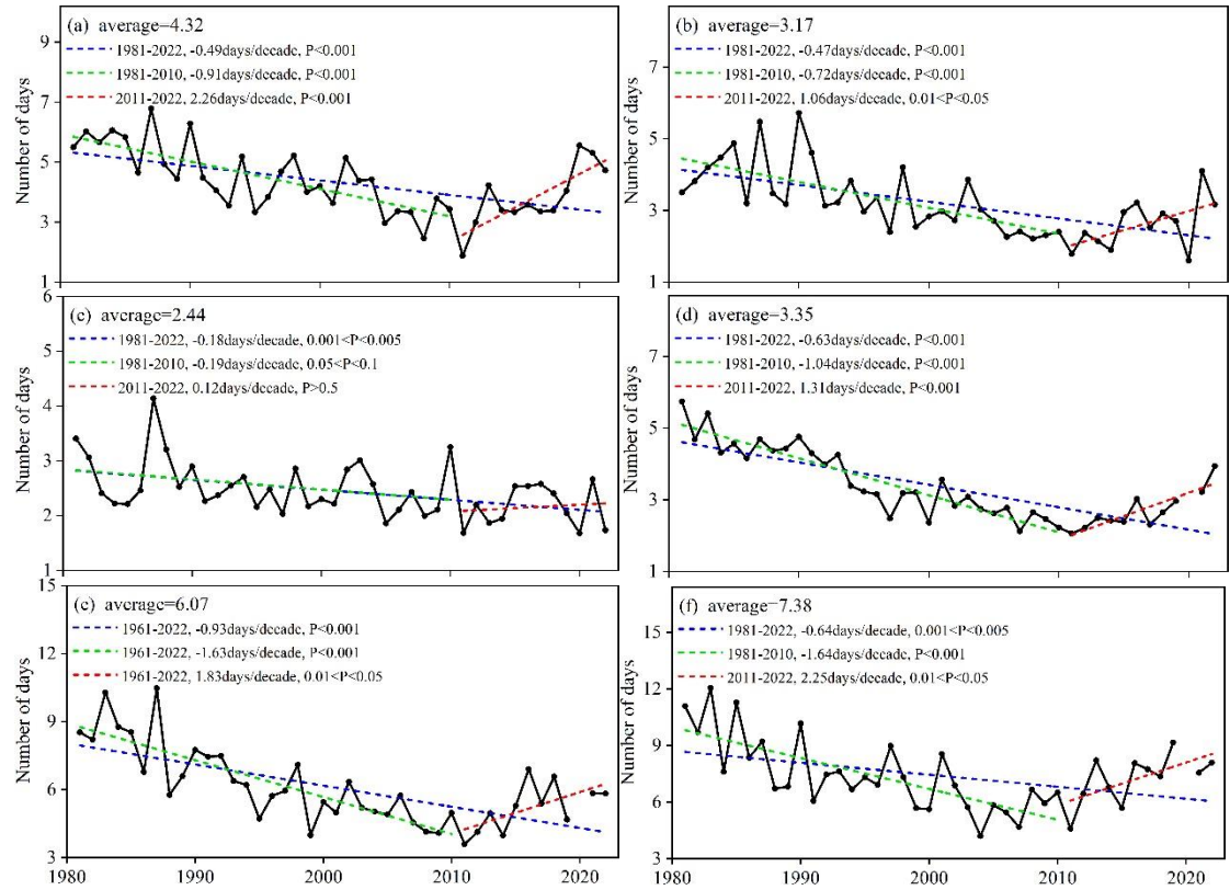
Figure S1. Inter-annual changes of regional CWPDs frequencies (W85/P85) during 1981–2022. (a: NEC; b: NC; c: NWC; d: SWC; e: YR; f: SC)
