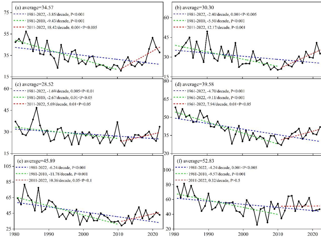
Figure S2. Inter-annual changes of regional CWPd intensities (W85∩P85) during 1981–2022. (a: NEC; b: NC; c: NWC; d: SWC; e: YR; f: SC)
