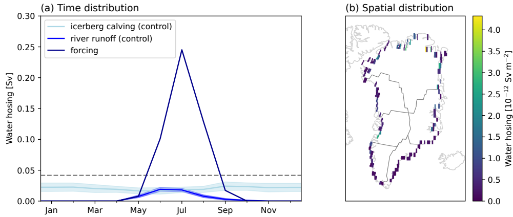
Figure B1. (a) Total monthly freshwater forcing time distribution, monthly climatologies of river runoff and monthly climatologies of iceberg calving fluxes and (b) May-September annual averaged freshwater forcing runoff spatial distribution. Values Forcing values are those given to the model as an input. The dashed lines line in (a) indicate indicates the annual average and of the average over forcing. The shadow areas in (a) represent the five months standard deviation of forcing monthly river runoff and iceberg calving fluxes. The grey lines in (b) indicate the separation between the six sub-drainage basins.
