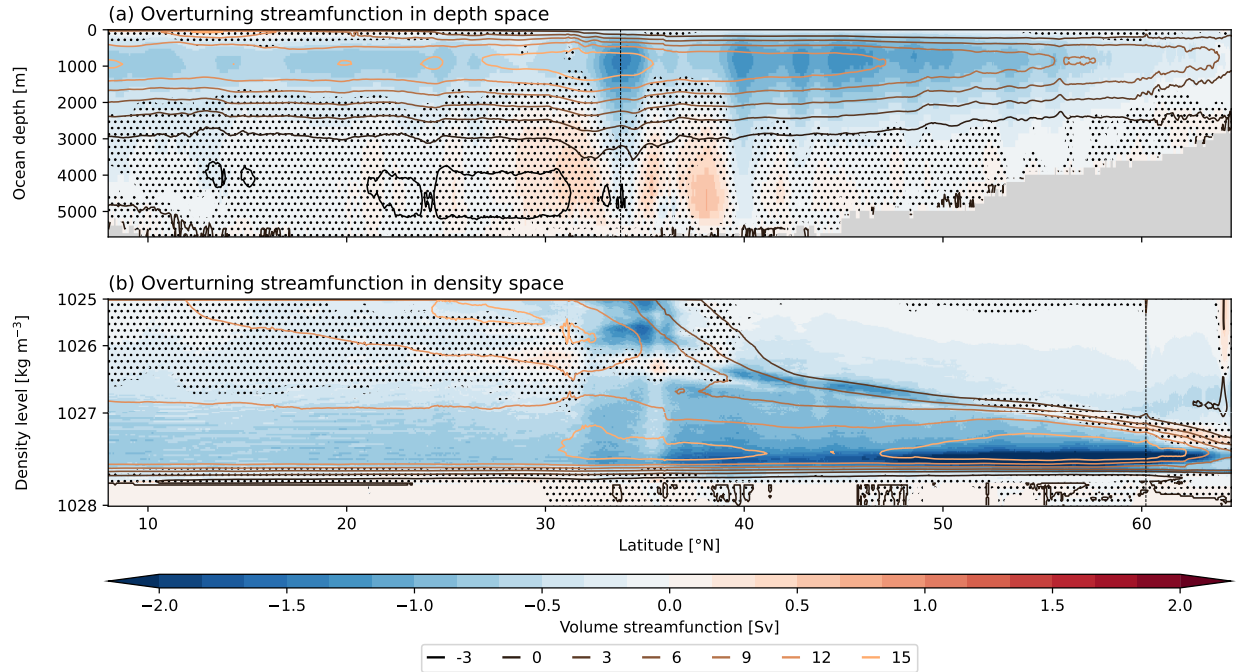
Figure 3. Response to the hosing in the last 10 simulated years (i.e. years 12 to 21 since after the hosing is started) for the overturning streamfunction in (a) depth space and (b) density space; filled coloured contours represent the ensemble-mean anomalies of the hosing with respect to the reference control and the contour lines the climatology of the control. Non-significant values as identified by the bootstrap methodology are masked with dots to improve the visibility over the significant areas. Vertical dashed lines mark the latitude where the maximum difference happens; 33.78° N in depth space and 60.21° N in density space.
