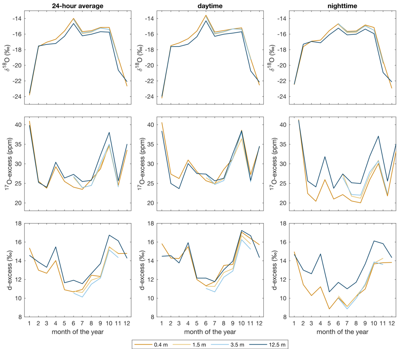
Figure B5: Monthly average of \delta^{18}\text{O} , ^{17}\text{O} -excess and d-excess of atmospheric water vapor at different heights above ground level (agl) in 2021 for daily, daytime and night-time conditions. Atmospheric water vapor at 1.5 and 3.5 m agl was monitored continuously only from June to November 2021, in relation to the oak forest growing season. Therefore, for these heights no isotopic data is available from January to May and December 2021.
