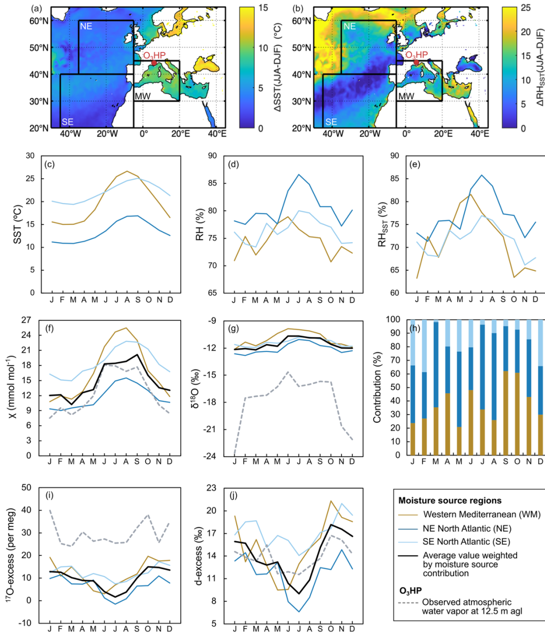
Figure 6: Seasonal and monthly variation in the isotopic composition of atmospheric water vapor measured at \text{O}_3\text{HP} compared with climate parameters and isotopic composition of atmospheric water vapor at the three main oceanic moisture sources. (a)-(b) Spatial variability of the difference between summer (JJA) and winter (DJF) sea surface temperature (SST) and relative humidity normalized to SST ( \text{RH}_{\text{SST}} ) in 2021. Data derived from ERA5 Reanalysis (Hersbach et al., 2020). The red circle indicates the location of the study site. (c)-(e) Monthly average SST, relative humidity above the ocean (RH) and \text{RH}_{\text{SST}} obtained from the ERA5 reanalysis dataset (Hersbach et al., 2020) for 2021. (f)-(j) Monthly average of atmospheric water mixing ratio ( \gamma ), relative contribution of the three moisture sources obtained from Lagrangian moisture source diagnostic (Sect. 3.6), \delta^{18}\text{O}_v , d -excess _v and ^{17}\text{O} -excess _v measured at \text{O}_3\text{HP} at 12.5 m agl (dashed line) and estimated above the three main oceanic moisture sources (solid lines). See Sect. 2.5 for more details on how the isotopic composition of water vapor over each moisture source is estimated.
