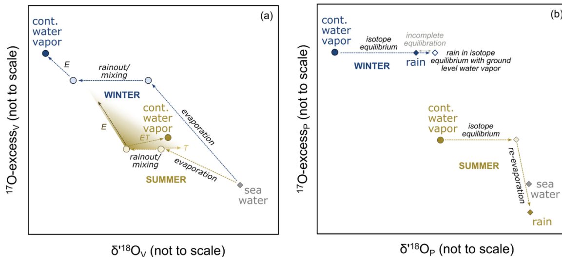
445 Figure 7: Synthesis of the effect of ocean evaporation, rainout, air mass mixing, continental moisture recycling (ET) resulting from evaporation (E) and plant transpiration (T), and post formation precipitation processes in winter (blue) and summer (yellow) on the triple oxygen isotopic composition of (a) atmospheric water vapor and (b) precipitation (see Sect. 4 for further details).
