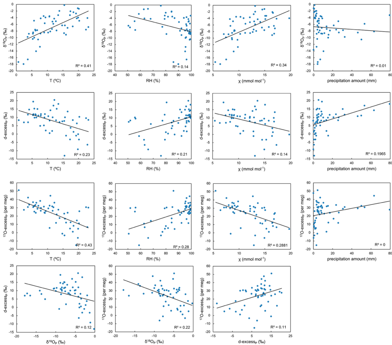
Figure B9: Correlations observed between event-based \delta^{18}\text{O} , d-excess and ^{17}\text{O} -excess of precipitation and relative humidity (RH), atmospheric temperature ( T_{\text{air}} ), the atmospheric water mixing ratio ( \chi ) and precipitation amount.
