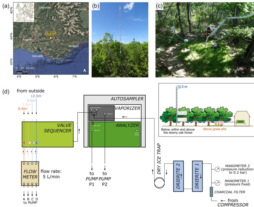
210 Figure 1: (a) Location of the study site O 2 HP . (Map: Google ©2026, Data: SIO, NOAA, U.S. Navy, NGA, GEBCO, Image: Landsat / Copernicus). (b) Mast installed within the downy oak forest canopy, equipped with intake lines for continuous atmospheric water vapor isotopic sampling. (Photo: C. Voigt). (c) Grass plot in the forest understory instrumented with micro-climate and atmospheric isotopic measurement systems (Photo: A. Alexandre). (d) Schematic illustration of the experimental setup. The solenoid valve behind the vaporizer 215 allowed switching between the valve sequencer used for atmospheric water vapor measurements and the dry air stream provided by the combination of compressed air, drierite columns and the dry ice trap used for weekly calibrations. See text for detailed description.
