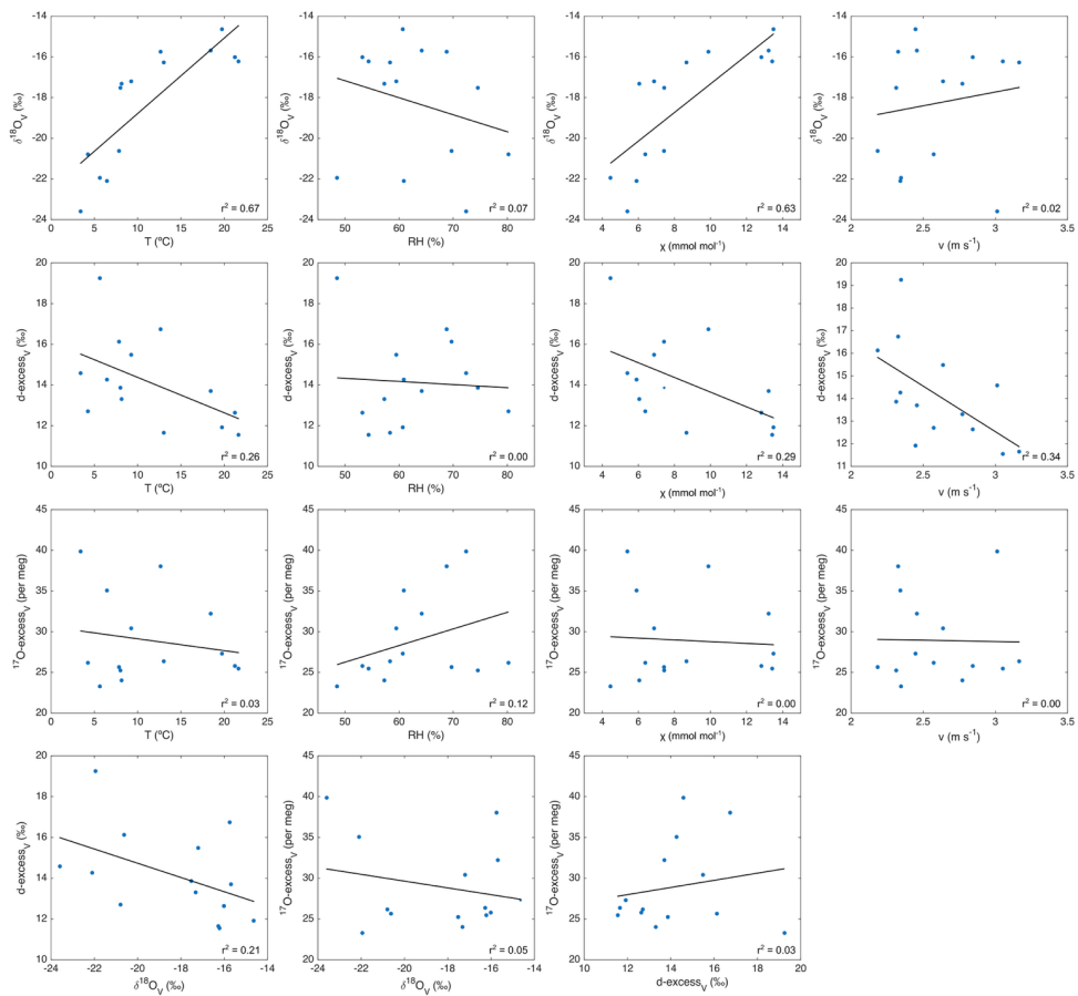
Figure B8: Correlations observed between monthly average \delta^{18}O , d-excess and ^{17}O -excess of atmospheric water vapor measured at 12.5 m agl and relative humidity (RH), atmospheric temperature ( T_{air} ), the atmospheric water mixing ratio ( \gamma ) and wind speed ( v ) at 10 m agl.
