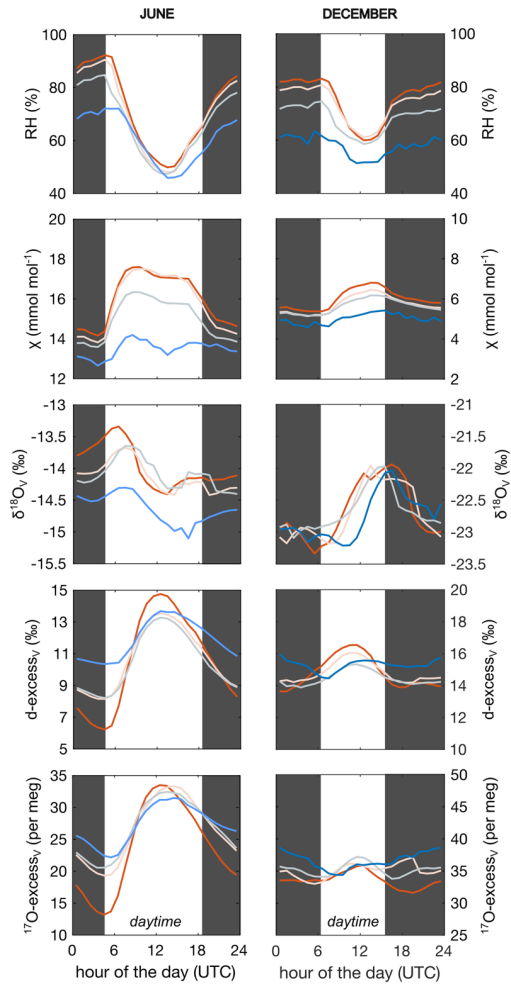
Figure 4: Monthly average daily cycle of relative humidity (RH), atmospheric water mixing ratio ( q ) and \delta^{18}\text{O}_v , d-excess v and ^{17}\text{O} -excess v of atmospheric water vapor at different measurements heights: above the grass plot (0.4 m agl; red), and below (1.5 m agl; pale), within (3.5 m agl; grey) and above (12.5 m agl, blue) the oak forest canopy. The left panels show monthly averages for June 2021, while the right panels show monthly averages for December 2021. For December, only the period from 01 to 25 December is included due to the lack of isotopic
