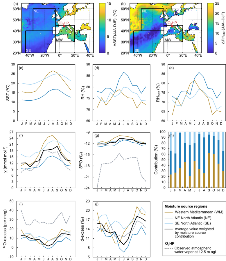
690 Figure 6: Seasonal and monthly variation in the isotopic composition of atmospheric water vapor measured at O 3 HP compared with climate parameters and isotopic composition of atmospheric water vapor at the three main oceanic moisture sources. (a)-(b) Spatial variability of the difference between summer (JJA) and winter (DJF) sea surface temperature (SST) and relative humidity normalized to SST (RH SST ) in 2021. Data derived from ERA5 Reanalysis (Hersbach et al., 2020). The red circle indicates the location of the study site. (c)-(e) Monthly average SST, relative humidity above the ocean (RH) and RH SST obtained from the ERA5 reanalysis dataset (Hersbach et al., 2020) for 2021. (f)-(j) Monthly average of atmospheric water mixing ratio ( \gamma ), relative contribution of the three moisture sources obtained from Lagrangian moisture source diagnostic (Sect. 3.6), \delta^{18}\text{O} , d-excess and ^{17}\text{O} -excess measured at O 3 HP at 12.5 m agl (dashed line) and estimated above the three main oceanic moisture sources (solid lines). See Sect. 2.5 for more details on how the isotopic composition of water vapor over each moisture source is estimated.
