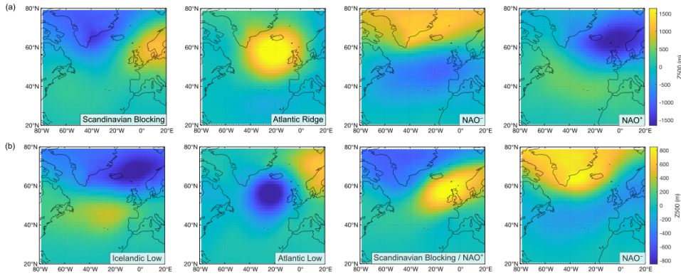
495 Figure C5: Centroids of (a) the four wintertime and (b) the four summertime weather regimes obtained from daily anomalous geopotential 500 height at the 500-hPa altitude ( Z_{500} , colour) from the European Centre for the Medium-Range Weather Forecasts (ECMWF) ERA5 reanalysis over 1989–2022. In winter, the Atlantic Ridge regime is associated with a high-pressure system over the Atlantic Ocean, driving strong northwesterly winds (Mistral) and resulting in cool, dry conditions in the Mediterranean region (Vautard, 1990). The NAO– regime 505 emerges when the Icelandic low shifts southward, displacing the Atlantic jet stream to lower latitudes and inducing southerly winds that bring warmer, wetter conditions to the Mediterranean (Cassou et al., 2004). In contrast, the NAO+ regime is characterized by a strong pressure gradient between the Icelandic Low and the Azores High, promoting westerly to northwesterly winds and generally dry conditions in the Mediterranean (Cassou et al., 2004). The Scandinavian Blocking regime involves a persistent anticyclone over the Scandinavian Peninsula, preventing low pressure systems reaching Europe and leads to north-easterly winds across the western Mediterranean. In summer, the Blocking/NAO+ regime resembles a blocking-like pattern, with a high-pressure anomaly over Scandinavia and the North Sea. The Atlantic Low is dominated by a low-pressure system over the North Atlantic, accompanied by weaker positive anomalies extending toward 510 Scandinavia, facilitating the advection of warm air masses from northern Africa and the Mediterranean basin (Cassou et al., 2005). The summer NAO– regime is characterized by a low-pressure anomaly over the British Isles and a strong high-pressure anomaly over Greenland, while the Icelandic Low regime displays a dipole pattern with a low-pressure anomaly between Iceland and Scandinavia and a weak high- pressure anomaly over the North Atlantic.
