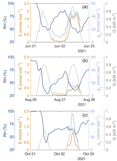
445 Figure B4: Diurnal evolution of transpiration ( E ) and stomatal conductance ( g_s ) of individual oak leaves in the sun-crown of the forest canopy in different stages of the oak forest growing season: (a) early stage, (b) dry stage, (c) last stage. The diurnal cycle of global solar radiation ( G , grey curve) and relative humidity (RH) are shown for comparison.
