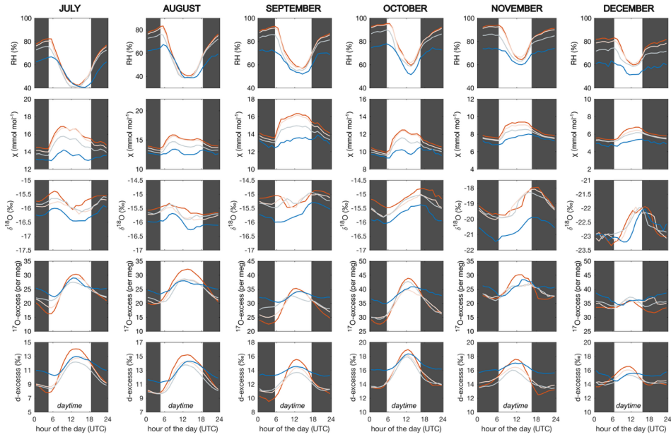
460 Figure B7: Same as Figure B6, but for July to December 2021.
