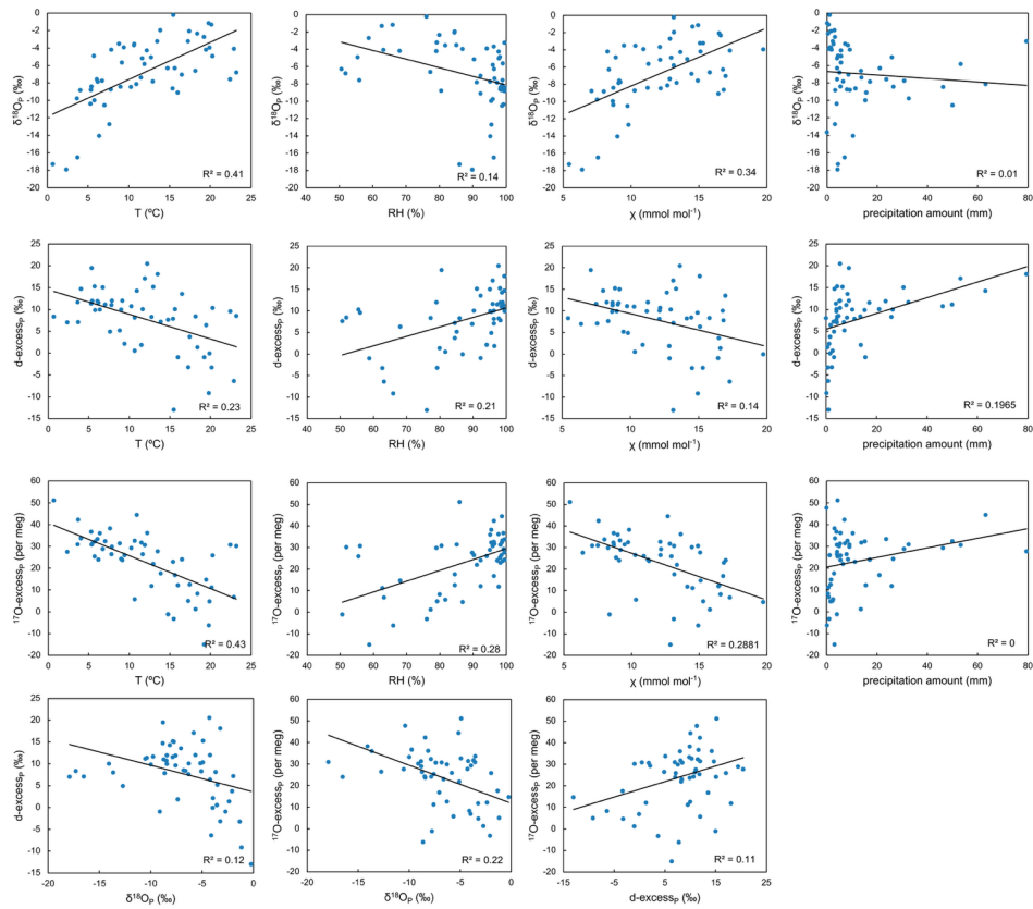
465 Figure B9: Correlations observed between event-based \delta^{18}O , d-excess and ^{17}O -excess of precipitation and relative humidity (RH), atmospheric temperature ( T_{air} ), the atmospheric water mixing ratio ( \gamma ) and precipitation amount.
