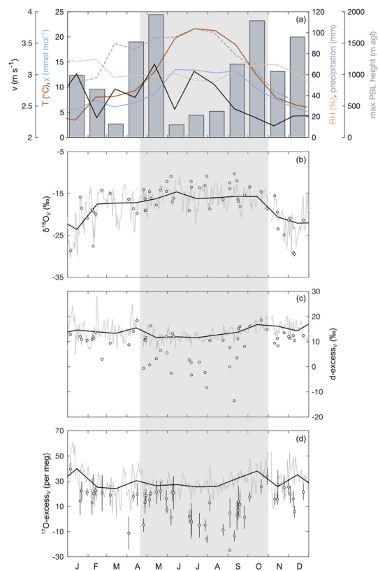
465 Figure 2: Time series of meteorological data and the isotopic composition of atmospheric water vapor measured at 12.5 m agl and estimated from isotopic equilibrium with precipitation in 2021. (a) Monthly precipitation amount and monthly average temperature ( T_{\text{air}} ), atmospheric water mixing ratio ( z ), wind speed ( v ), and relative humidity (RH) measured at 10 m agl. The grey dashed line shows the monthly average maximum planetary boundary layer height for the 0.25^\circ \times 0.25^\circ grid field covering the study site (Guo et al., 2022). (b)–(d) Solid lines represent daily (grey) and monthly (black) average isotopic composition of atmospheric water vapor measured at 12.5 m agl. Circles show the isotopic composition of water vapor estimated from isotopic equilibrium with event-based precipitation samples using T_{\text{air}} observed at 10 m agl. Note that the error bars for \delta^{18}\text{O} and d-excess are smaller than symbol size. The grey shaded area marks the oak forest growing season. 470
