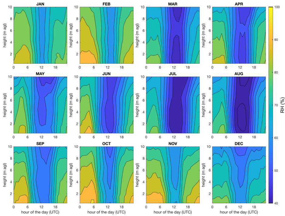
Figure B2: Monthly average variability of atmospheric relative humidity in the near-surface atmosphere over the day. Relative humidity measurements at 0.4 m, 1.5 m, 1.9 m, 4.4 m, 6.15 m and 10 m agl were obtained from the O 3 HP database (Reiter et al., 2015). Data were linearly interpolated between measurement heights, and the hourly means were computed for each month.
