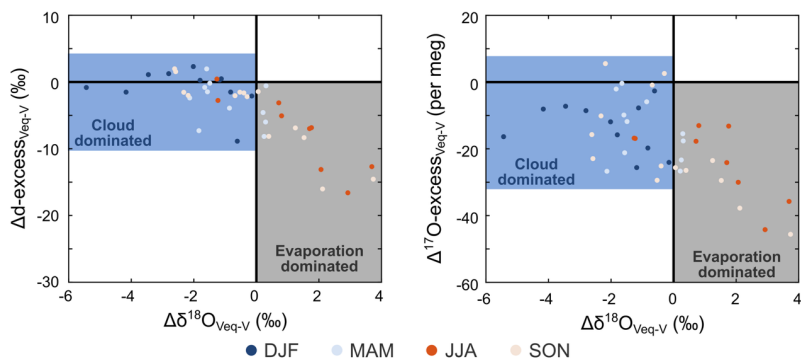
595 Figure 5: Isotopic difference ( \Delta ) between water vapor estimated from isotopic equilibrium with precipitation ( \text{V}_{\text{eq}} ) and amount-weighted atmospheric water vapor measured at 12.5 m above ground level ( \text{V} ) for each precipitation event in 2021. Data is coloured according to season. The blue-shaded area indicates samples for which the equilibration between precipitation and near-surface atmospheric water vapor is likely incomplete. Precipitation samples that correspond to data falling within the grey-shaded area are likely affected by re-evaporation during fall through the air column.
