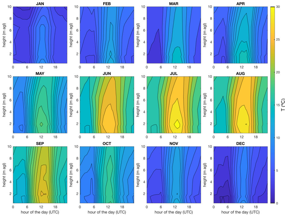
Figure B1: Monthly average variability of atmospheric temperature in the near-surface atmosphere over the day. Temperature measurements at 0.4 m, 1.5 m, 1.9 m, 4.4 m, 6.15 m and 10 m agl were obtained from the O 3 HP database (Reiter et al., 2015). Data were linearly interpolated between measurement heights, and the hourly means were computed for each month.
