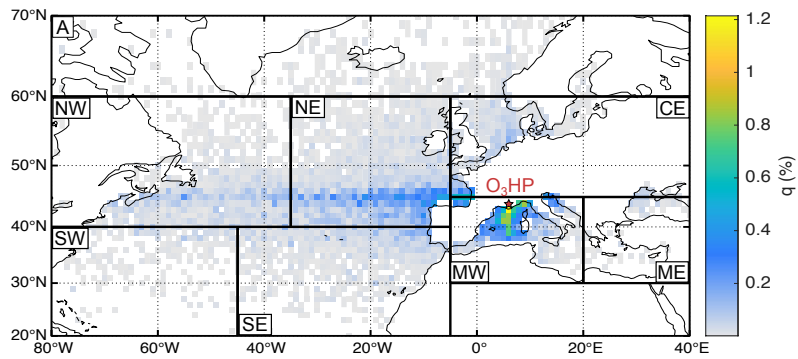
470 Figure C1: Annual mean oceanic moisture source contributions to atmospheric water vapor at O 3 HP. Shading: Relative contribution of evaporation from respective grid cell to the final specific humidity of each trajectory.
