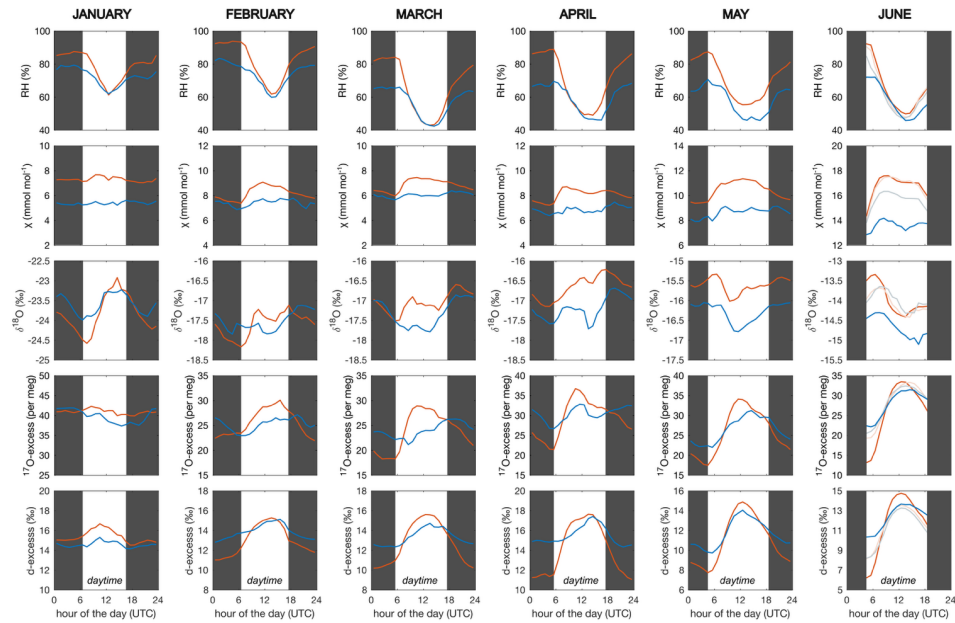
Figure B6: Monthly average diurnal cycle of relative humidity (RH), atmospheric water mixing ratio ( x ) and \delta^{18}\text{O} , d-excess and ^{17}\text{O} -excess of atmospheric water vapor at different measurements heights above the grass plot (red) and below (pale), within (grey) and above (blue) the oak forest canopy for January to June 2021. The grey shaded areas indicate the night-time periods.
