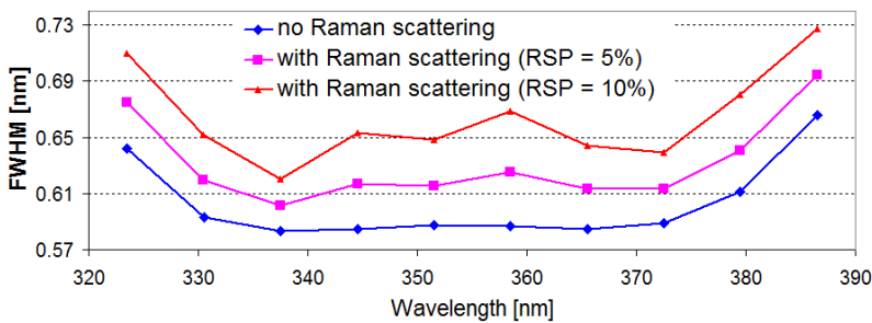
Fig. 6 a) Convolved high-resolution high-resolution solar spectrum without and with the contribution of rotational Raman scattering (RSP of 10%). b) FWHM derived from KFs (without intensity offset) for spectra with different contributions of Raman scattering.
