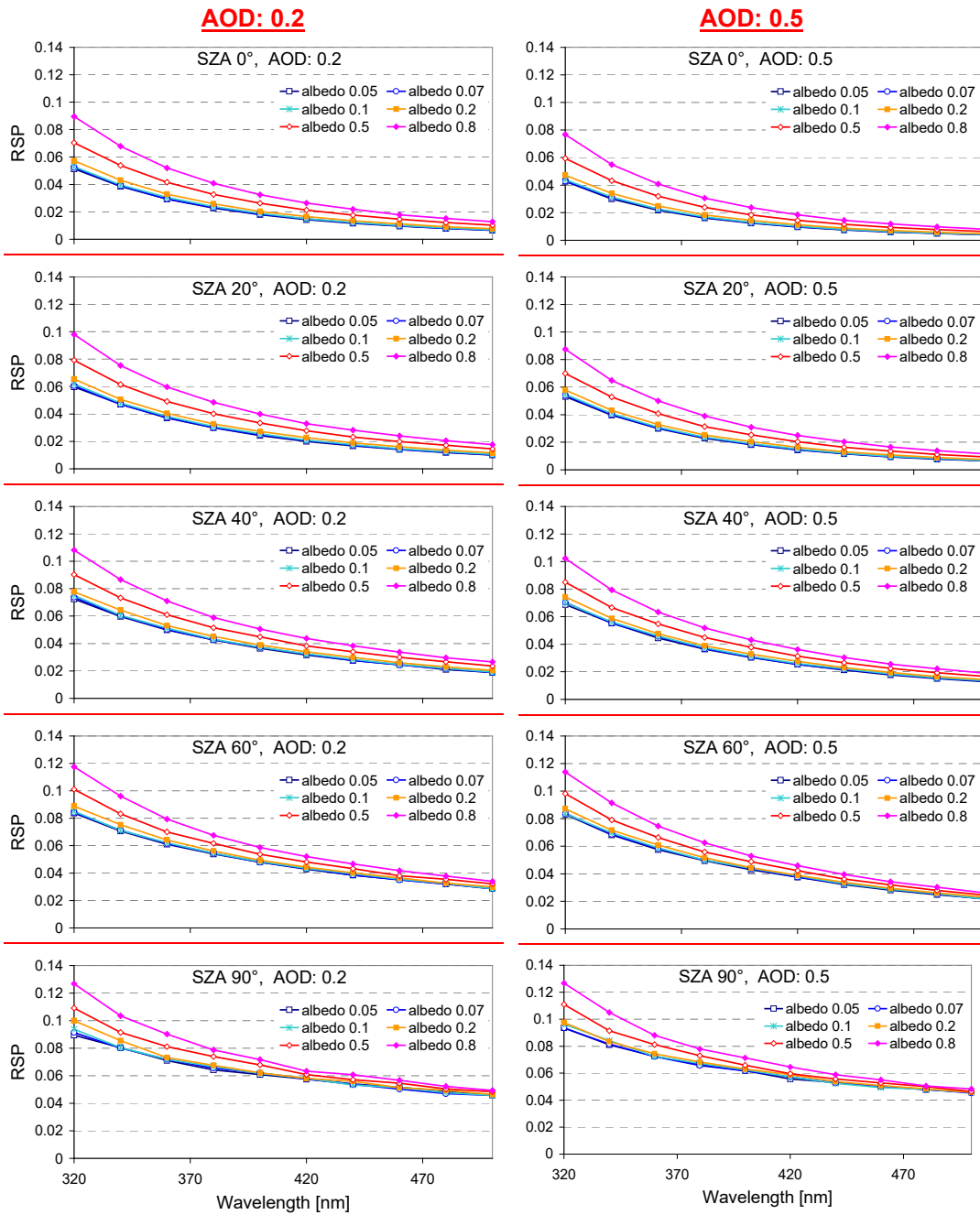
Fig. A6 Dependence of the RSP on wavelength for different surface albedos, SZA and aerosol loads derived from radiative transfer simulations with the radiative transfer model MCARTIM (Deutschmann et al., 2011). The aerosol profile is assumed as box-profile from the surface to 1 km. Single scattering albedo and asymmetry parameter are set to 0.95 and 0.68, respectively.
