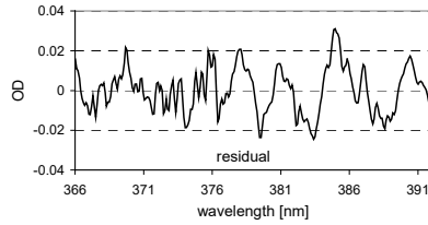
915 Fig. A8-A11 Same as Fig. 11, but for the fit ranges 334.5 – 360.5 nm and 366 – 392 nm.
