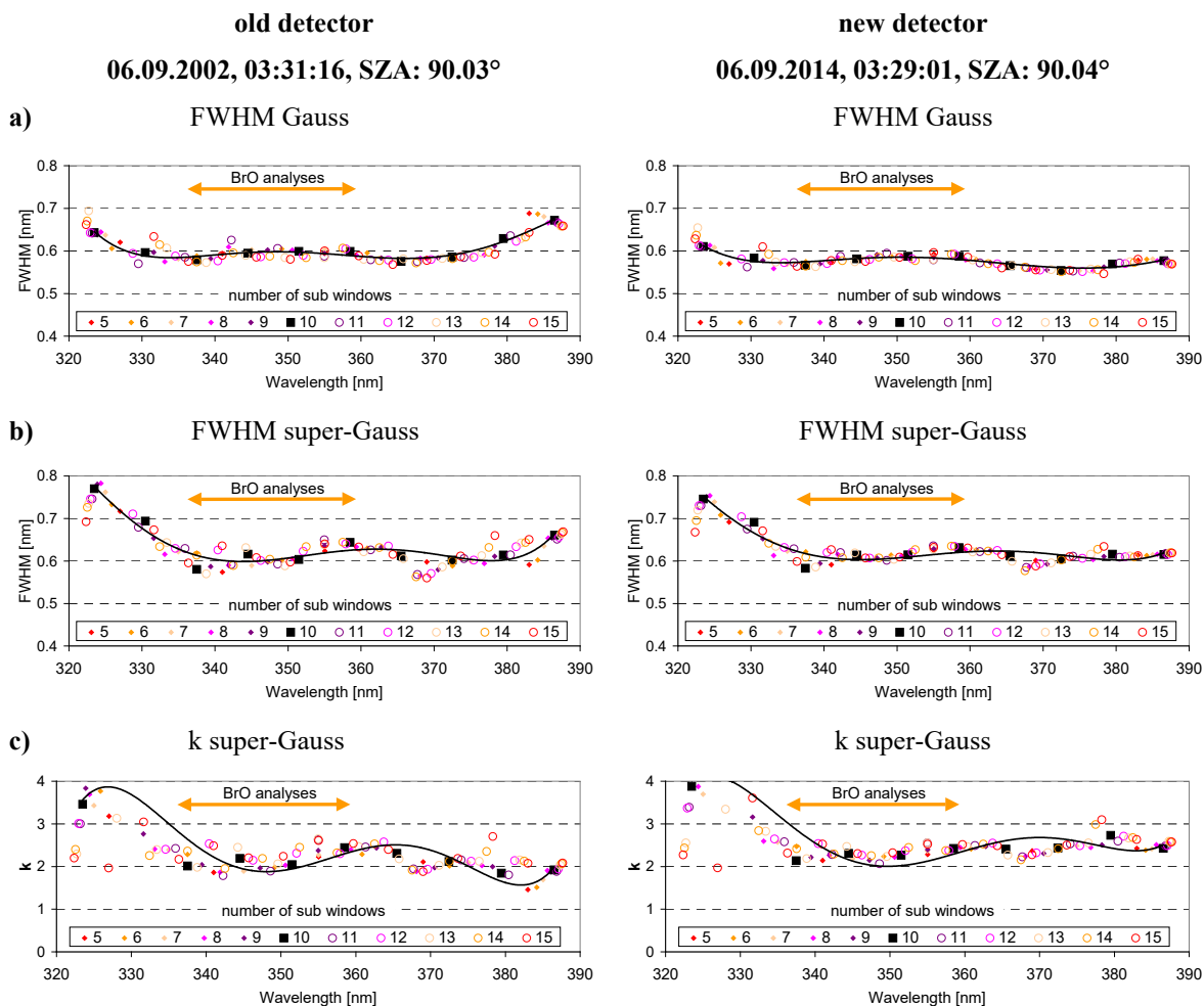
150 Fig. 2 Results of the KF for two selected zenith-sky zenith-sky spectra taken at a SZA of about 90^\circ , one from the old detector (left) and one for the new detector (right). The FWHM was either derived assuming a Gaussian (a) or super-Gaussian (b)
