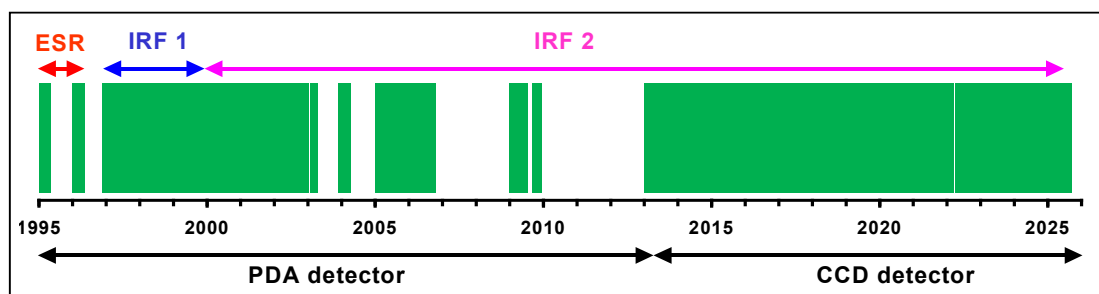
Fig. 1 a) Map with the two locations of the instrument (© google maps); b) timeline of the zenith DOAS measurements. ERS-ESR and IRF 1/2 indicate measurements at ESRANGE and the Swedish Institute for of space-Space physics-Physics near Kiruna, respectively. IRF 1 represents the period between Dec'96 and Oct'99 when the instrument was installed in a small hut on the roof of the institute; after Oct'99 (IRF 2), the instrument was operated in a room inside the institute. Between December 1996 and
