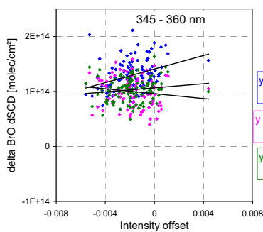
Fig. A10 Correlation plots of the deviations of the BrO dSCDs from those of the standard analyses if the free fitting of a spectral shift, intensity offset, or both is deactivated versus the spectral shift (right) or intensity offset (left) derived from the standard analyses.
