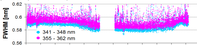
d) FWHM (with offset)
