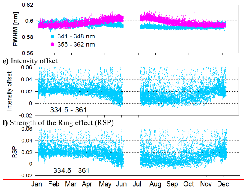
Fig. 4 Seasonal variation (2014 – 2023) of a) the snow depth (data obtained from the Swedish Meteorological and Hydrological Institute, https://www.smhi.se/data , last accessed 17 November 2025). A snow depth of zero indicates a snow-free surface; b) measured radiance (counts per second) for measurements with SZA between 79.5° and 80.5° (red) and 89.5° and 90.5° (blue); c) FWHM derived from a KF without intensity offset; d) FWHM derived from a KF with intensity offset; e,f) intensity offset and RSP derived from an analysis with a pre-convolved high-resolution solar spectrum used as Fraunhofer reference spectrum (see section Sect. 4 ).
