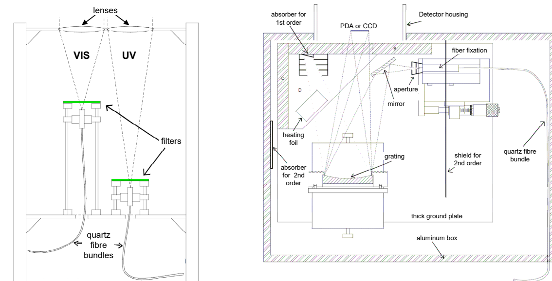
Fig. A1 left ) Entrance optics including telescope lenses, optical filters (UG5 for the UV spectrometer) and quartz fibre bundles. right ) set-up of the UV spectrometer (adapted from Otten, 1997).
