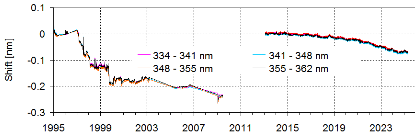
b) intensity offset derived from Gaussian parameterisation
