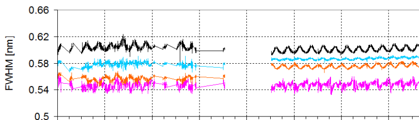
c) Gaussian parameterisation, with Ring spectrum
