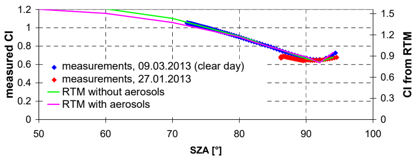
955 Fig. A9-A12 SZA dependence of the colour index (ratio of radiances at 330 nm and 380 nm) for measurements with the old (a) and new (b) detector. The blue dots represent measurements on a clear day, which can be directly compared to the radiative transfer simulations. The red dots represent measurements on a day which was affected by clouds (27 January 2013). The measured CI for this day are almost the same as for the clear day. The radiative transfer simulations were performed for two scenarios: either for an atmosphere with or without aerosols (for more details see text).
