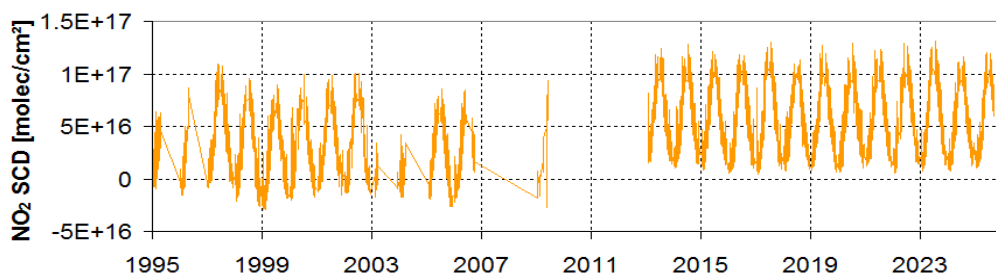
445 Fig. 9 Retrieved intensity offset, RSP and the SCDs of O 3 and NO 2 from the DOAS analysis with convolved sun spectra. Results for daily measurements (SZA = 90°±0.5°) and for three different spectral ranges.
