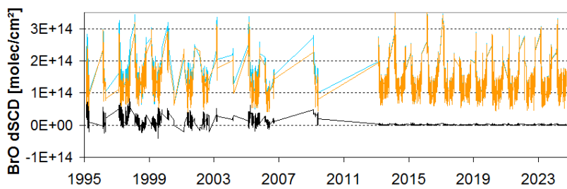
c) BrO dSCD, 345 – 360 nm
