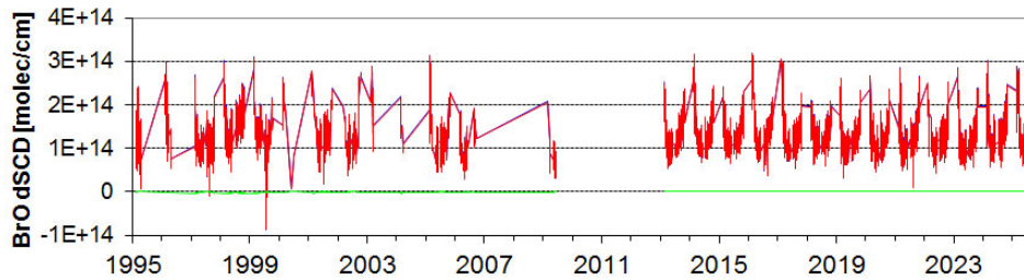
Fig. A5-A7 Time series of BrO dSCDs ( 90^\circ - 80^\circ SZA) obtained for different fit windows and ISFRISRF parameterisations (red: Gauss; blue: super-Gauss). The green lines represent the differences. For both parameterisations, almost identical results are found.
