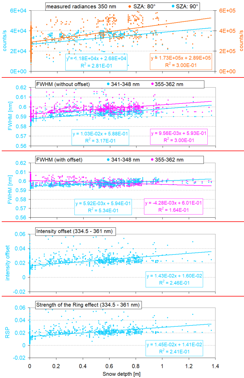
Fig. A4 Correlation plots of the quantities shown in Fig. 4 (b to f) versus the snow depth (Fig. 4a)
