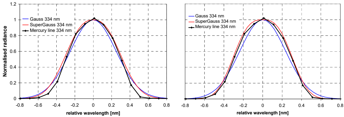
345 Fig. 7 Measured slit function (black, Mercury line at 334 nm, measurement from 03 September 2002) and ISRF-ISRF derived from KFs with Gaussian and super-Gaussian parameterisations to an original (a) and (b) Raman-corrected measured zenith skyzenith-sky spectrum from 06 September 2002, 03:31 UTC (SZA: 90.028°). The Mercury lines in both plots are the same.
