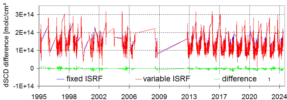
Fig. A7-A9 Time series of BrO dSCDs ( 90^\circ - 80^\circ SZA) for different fit windows and ISRFs (fixed or variable). The green lines represent the differences between both analyses (results with variable ISRF minus results with fixed ISRF).
