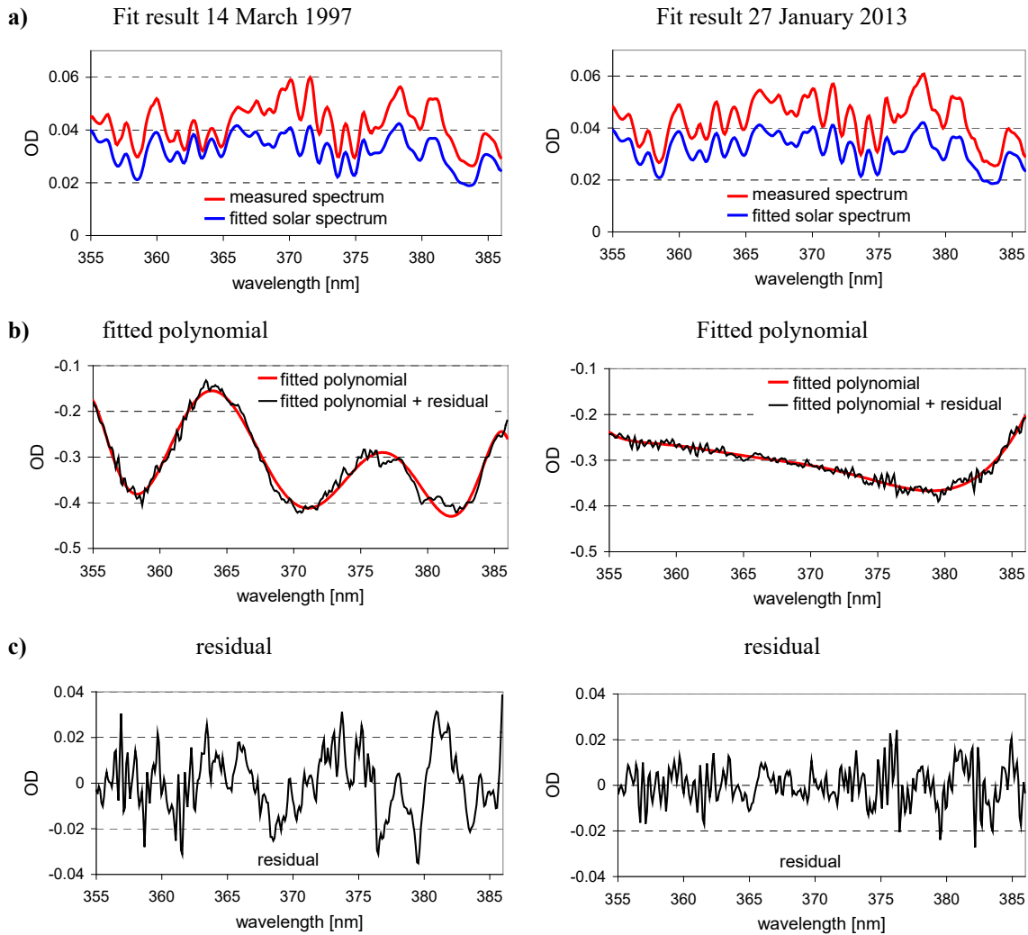
505 Fig. 11 Fit results for selected spectra of the old (14 March 1997, 05:10 UTC, SZA: 90.2°) and new (27 January 2013, 13:15 UTC, SZA: 90.13°) detector using a convolved high-resolution sun spectrum as FRS. Results for the other spectral ranges (334.5 – 360.5 nm and 366 – 392 nm) are shown in Fig. A7-A11 in the appendixAppendix .
