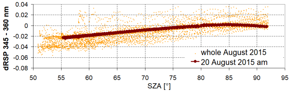
d) FWHM derived from KF (without intensity offset)
