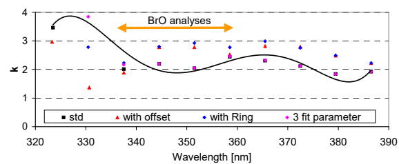
Fig. A2 Same as Fig. 2, but including also a Ring spectrum or an intensity offset or for a freely fitted third fit parameter of the super-Gaussian parameterisation.
