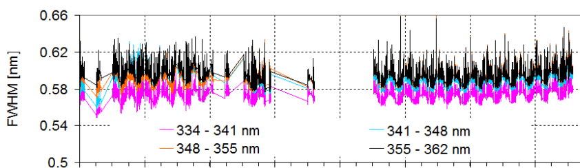
b) Gaussian parameterisation, with intensity offset
