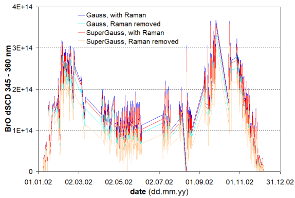
885 Fig. A6-A8 Retrieved BrO dSCDs (90° - 80° SZA) for the year 2002 using reference spectra created with different ISRF (see text).
