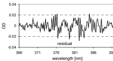
915 Fig. A8-A11 Same as Fig. 11, but for the fit ranges 334.5 – 360.5 nm and 366 – 392 nm.
