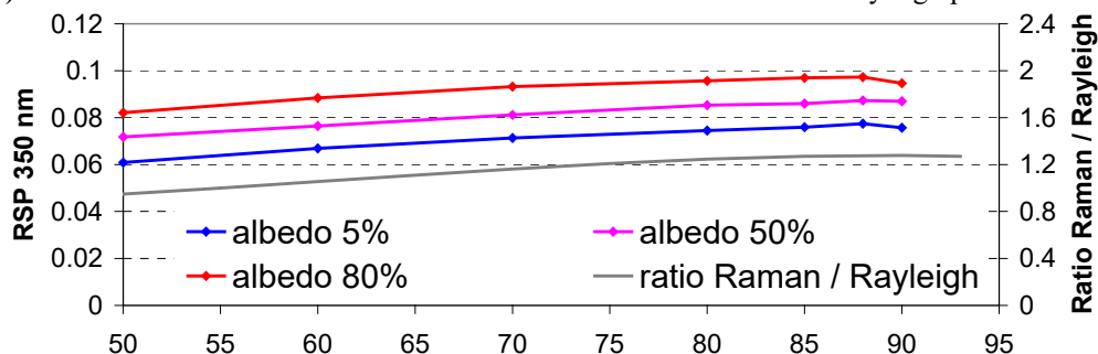
b) Measured d RSP for April 2015 (high surface albedo)
