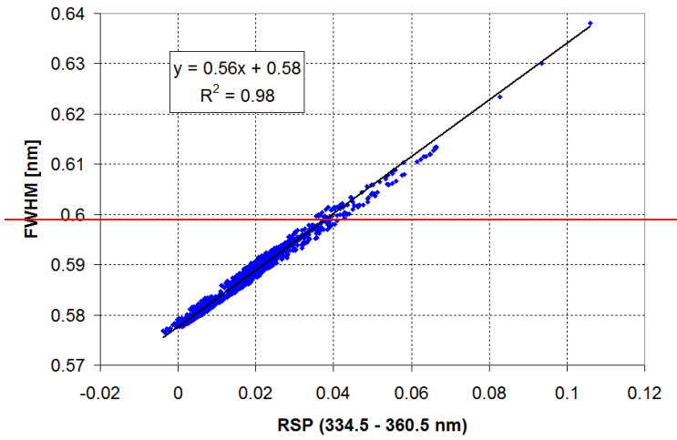
Fig. A3 FWHM derived from a KF (341—348 nm) with a Gaussian parameterisation and without intensity offset plotted versus the strength of the Ring effect (expressed as RSP) derived from a DOAS analysis with a preconvolved solar spectrum, see Sect. 4). Measurements for SZA around 90° ( \pm 0.5^\circ ) in 2015. Similar results are found for other combinations of fit ranges used for the determination of the strength of the Ring effect and for the determination of the FWHM.
