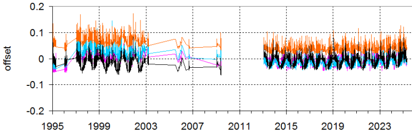
c) Raman scattering pobability (RSP) derived from Gaussian parameterisation
