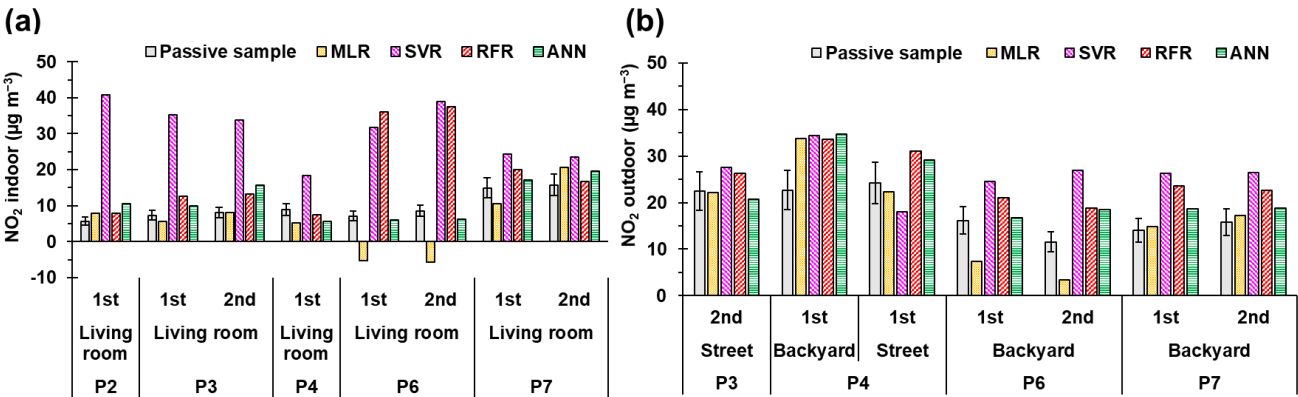
Figure 9. Comparison of the \text{NO}_2 calibration models with the concentration measured by the diffusion tubes (two-week period) for (a) indoor and (b) outdoor sensors. Models (in different colours) were trained with data averaged every 10 min. Error bars indicate the expanded uncertainty of the diffusion tubes (18.4 %).
