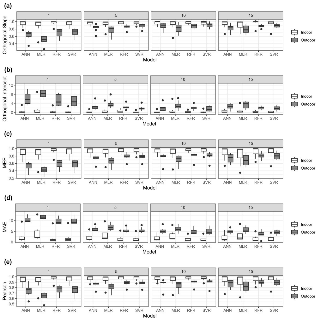
510 Figure 7. Boxplots of various performance evaluation metrics: (a) orthogonal slope, (b) orthogonal intercept (in ppb), (c) model efficiency (MEF), (d) MAE (in ppb) and (e) Pearson correlation coefficient, for different tested models (ANN, MLR, RFR and SVR) for the different time aggregations (1, 5, 10 and 15 min) applied to the testing data for indoor and outdoor NO 2 sensors.
