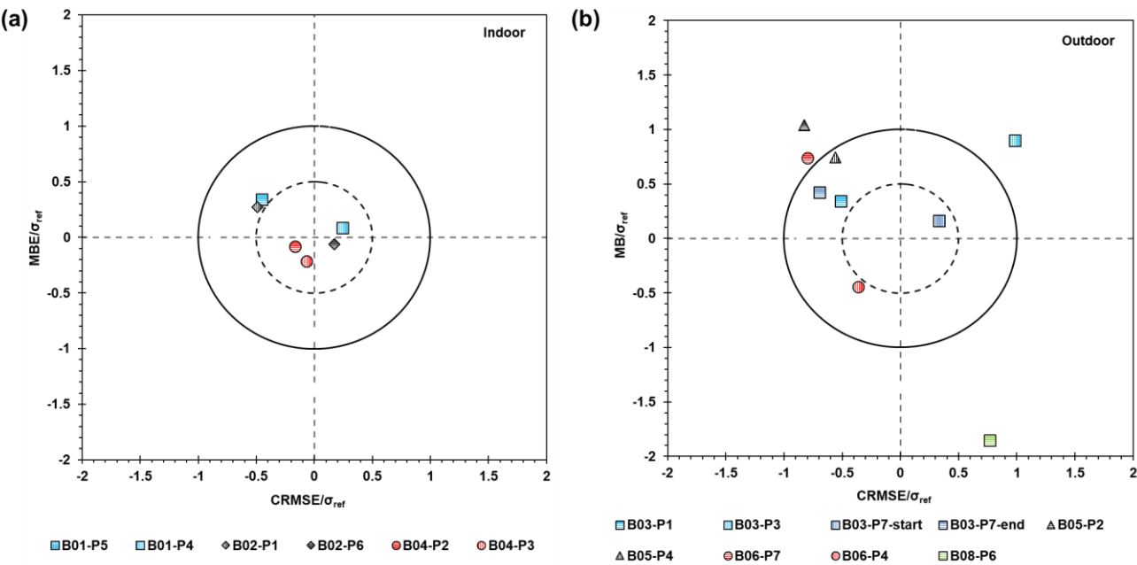
Figure 5. Target diagrams for (a) indoor and (b) outdoor PM 2.5 sensors. The coloured symbols are different AQSSs which were later deployed in the house of different patients (B0X-PX) and therefore some AQSSs were through more than one calibration phase. B03 was calibrated before the deployment in the house of patient 7 (B03-P7-start) and after the deployment (B03-P7-end).
