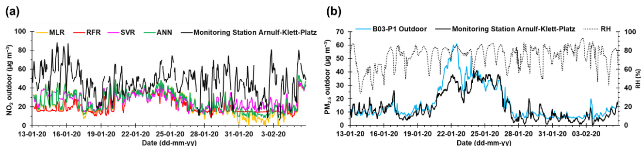
Figure 10. Time series of hourly outdoor (a) \text{NO}_2 calculated using the four tested calibration models (in different colours MLR, RFR, SVR and ANN) and (b) \text{PM}_{2.5} concentrations calculated using the ULR calibration model during deployment in the house of patient P1 as well as the RH. The data of the RI is shown with a solid black line in both graphs.
