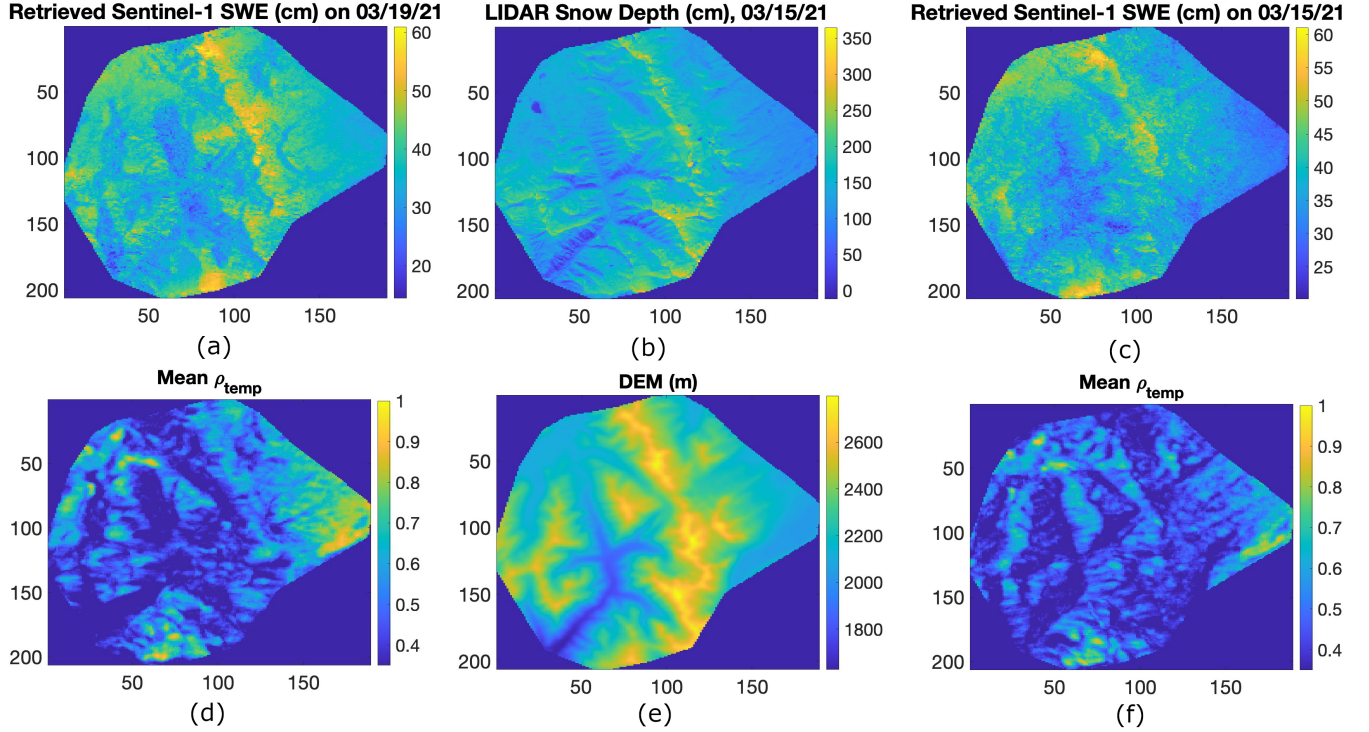
Figure 5. Total retrieved SWE using 6-day repeat Sentinel-1 time series data for (a) 6 am and (c) 6 pm acquisitions, accumulated from December 1 to the date closest to the LIDAR acquisition over Banner Summit. (b) LIDAR-derived total snow depth on 03/15/2021. Mean Sentinel-1 temporal coherence for (d) 6 am and (f) 6 pm acquisitions. (e) Digital elevation model (DEM) of the Banner Summit study area.
