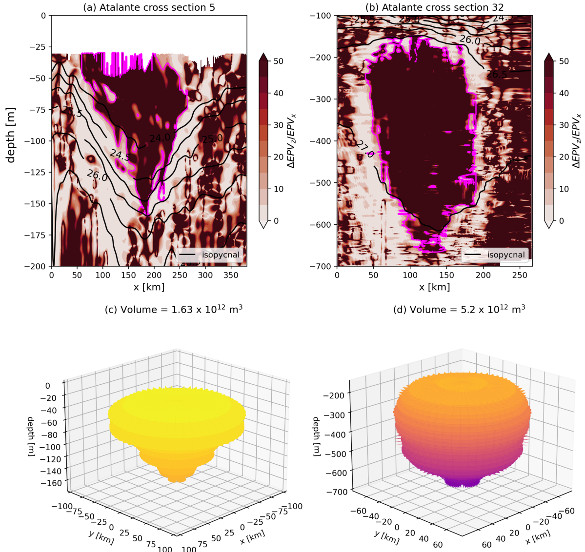
Figure 9. Boundaries of NBC_{surf}1 and NBC_{sub}1 are shown in magenta in a and b, respectively, with \Delta EPV_z/EPV_x as the background field. c-d) Three-dimensional reconstructions using the methodology outlined in Section 3.2, with volume values indicated. Isopycnal surfaces are plotted as dark lines.
