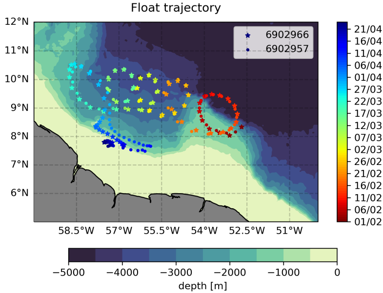
Figure 12. Trajectories of Argo floats N°6902966 and 6902957 within the core of NBC_{sub2} over time, illustrating the material coherence of the eddy. Both floats follow a similar looping pattern until exiting the core of the eddy around April 1. Regional bathymetry is shaded (ETOPO2; Smith and Sandwell (1997)).
