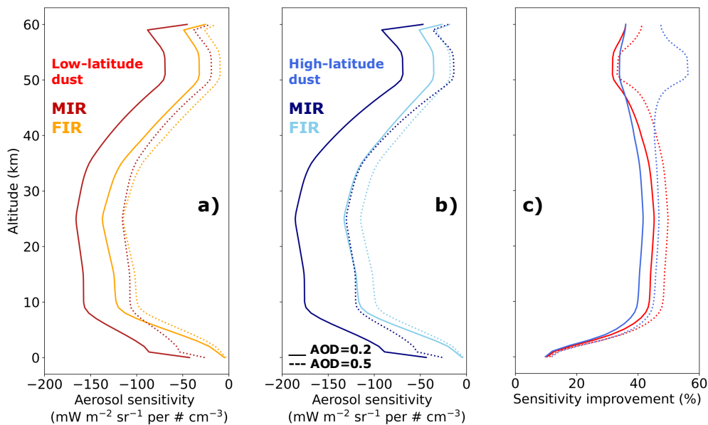
280 Figure 6: Aerosol sensitivity integrated in the sensitive FIR (300-667 \text{cm}^{-1} ) and MIR (800-1200 \text{cm}^{-1} ) spectral regions, for a low-latitude (LMLD2, panel a) and a high-latitude (HLD1, panel b) dust sample. The FIR sensitivity is represented by yellow (panel a) and light blue (panel b), and the MIR sensitivity is represented by red (panel a) and dark blue (panel b) curves. In both panels a and b, scenarios with AOD=0.2 and 0.5 are represented as solid and dotted lines, respectively. The sensitivity improvement for the four scenarios is in panel c: red and blue curves are for low- and high-latitude dust, solid and dotted lines for AOD=0.2 and 0.5 respectively. All scenarios are for a dust layer peaking at 5 km altitude and for a polar background atmosphere.
