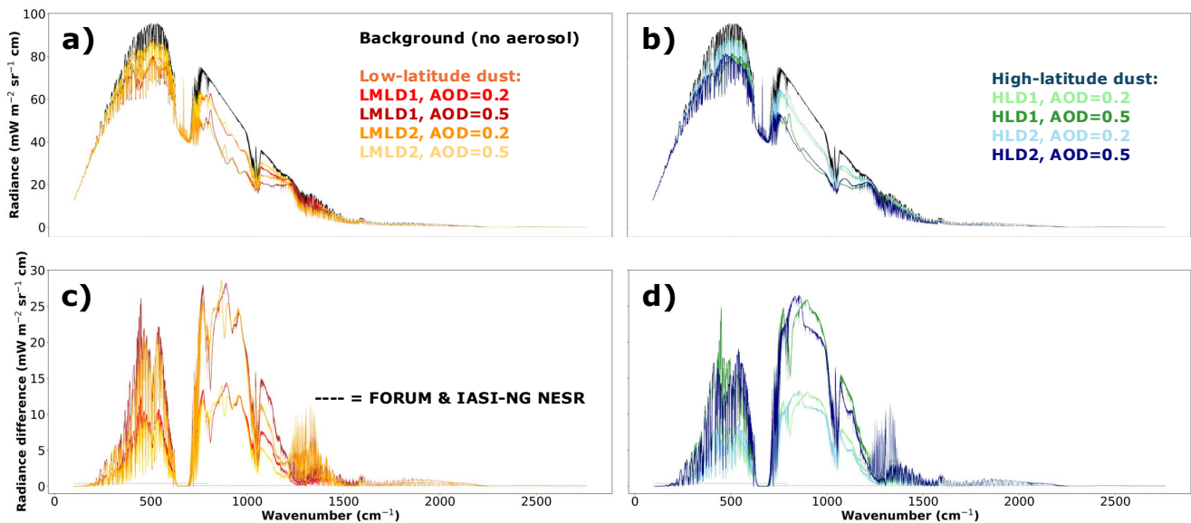
215 Figure 3: Merged FORUM and IASI-NG PO spectra for low- (a, curves in red and yellow shades) and high-latitude dust (b curves in green and blue shades), with different FIR AOD values (see Tab. 1). The aerosol source regions, for both low- and high-latitudes dust samples (see Fig. 2) are indicated in the panels. A background spectrum, i.e. with the same configuration but without any dust layer, is shown as a black curve in panels a and b, as a baseline reference. Spectral signatures of the different dust layers, i.e. the difference of the background and the dust-laden FORUM and IASI-NG PO are shown in panels c and d. The FORUM and IASI-NG average noise equivalent spectral radiance (NESR) is shown in panels c and d.
