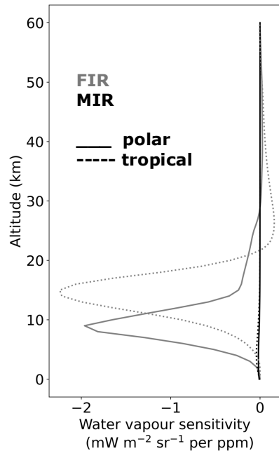
325 Figure 7: Water vapour sensitivity integrated in the full FIR (grey lines) and MIR (black lines) spectral regions, for a polar (solid lines) and a tropical background atmospheres.
