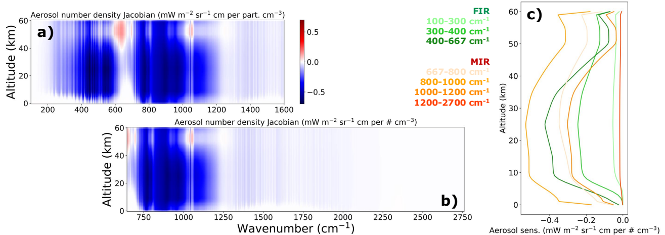
Figure 5: FORUM (a) and IASI-NG (b) Jacobians K(v, z) with respect to the aerosol number density, for the case of Australia dust sample, with a FIR AOD=0.2, a vertical profile peaking at 5 km altitude, in a polar atmosphere. Average aerosol sensitivity, quantified through the average Jacobians at different FIR (curves in green shades) and MIR sub-regions (curves in yellow-red shades) (c). Specific spectral intervals of these sub-regions are listed in the figure, with colours corresponding to those of the curves in panel c. The spectral aerosol sensitivity is estimated using FORUM Jacobians, for the FIR, and IASI-NG Jacobians, for the MIR.
