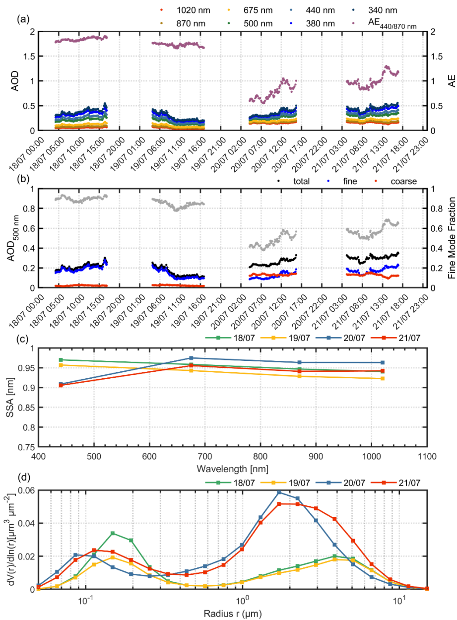
Figure 7. Time-series of values of the (a) AOD for various wavelengths (340 - 1020 nm) and AE at 440/870 nm (b) AOD at 500 nm along with the FMF (c) SSA wavelength dependence and (d) Particle volume size distribution obtained by the NTUA CIMEL sun-sky-lunar photometer for the period 18- 21 July 2023.
