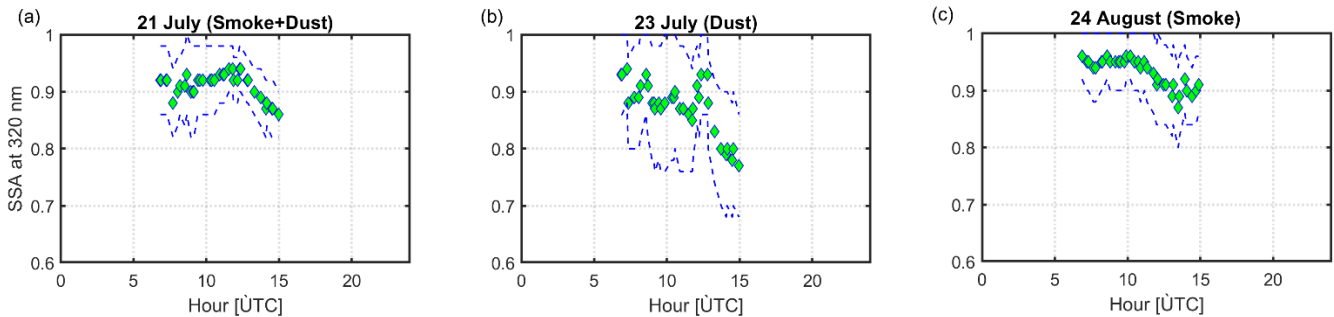
Figure 14. SSA at 320 nm for three representative cases: (a) 21 July (smoke + dust), (b) 23 July (dust), and (c) 24 August (smoke). The dotted blue lines represent the SSA values for irradiances that are within \pm 5\% around the measured values.
