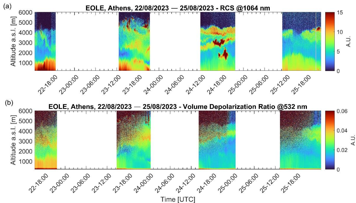
Figure 9. Spatio-temporal evolution of the (a) range-corrected lidar signal (RCS) at 1064 nm and (b) volume depolarization ratio at 532 nm for the period 22-25 August 2023.
