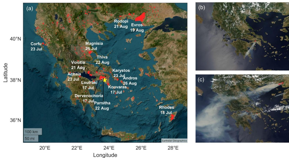
Figure 2. (a) Map of Greece illustrating wildfires detected by Aqua MODIS NASA Satellite imagery from 17 July to 31 August 2023 and satellite image showing wildfires over Greece (b) afternoon 18 July 2023 and (c) afternoon 22 August 2023 - data from Aqua MODIS, NASA. 290 Smoke plumes from these fires were transported across the Aegean Sea and Athens, reaching altitudes up to ~6 km. The elevated aerosol layers observed over Athens during this period resulted from both fine-mode biomass burning (BB) particles and coarse-mode Saharan dust intrusions. FLEXPART simulations and MODIS fire detection data provided clear evidence of the origin and evolution of these intrusions. Between 20 and 25 July, air masses arriving over Athens originated from North Africa, including Morocco, Tunisia, and
