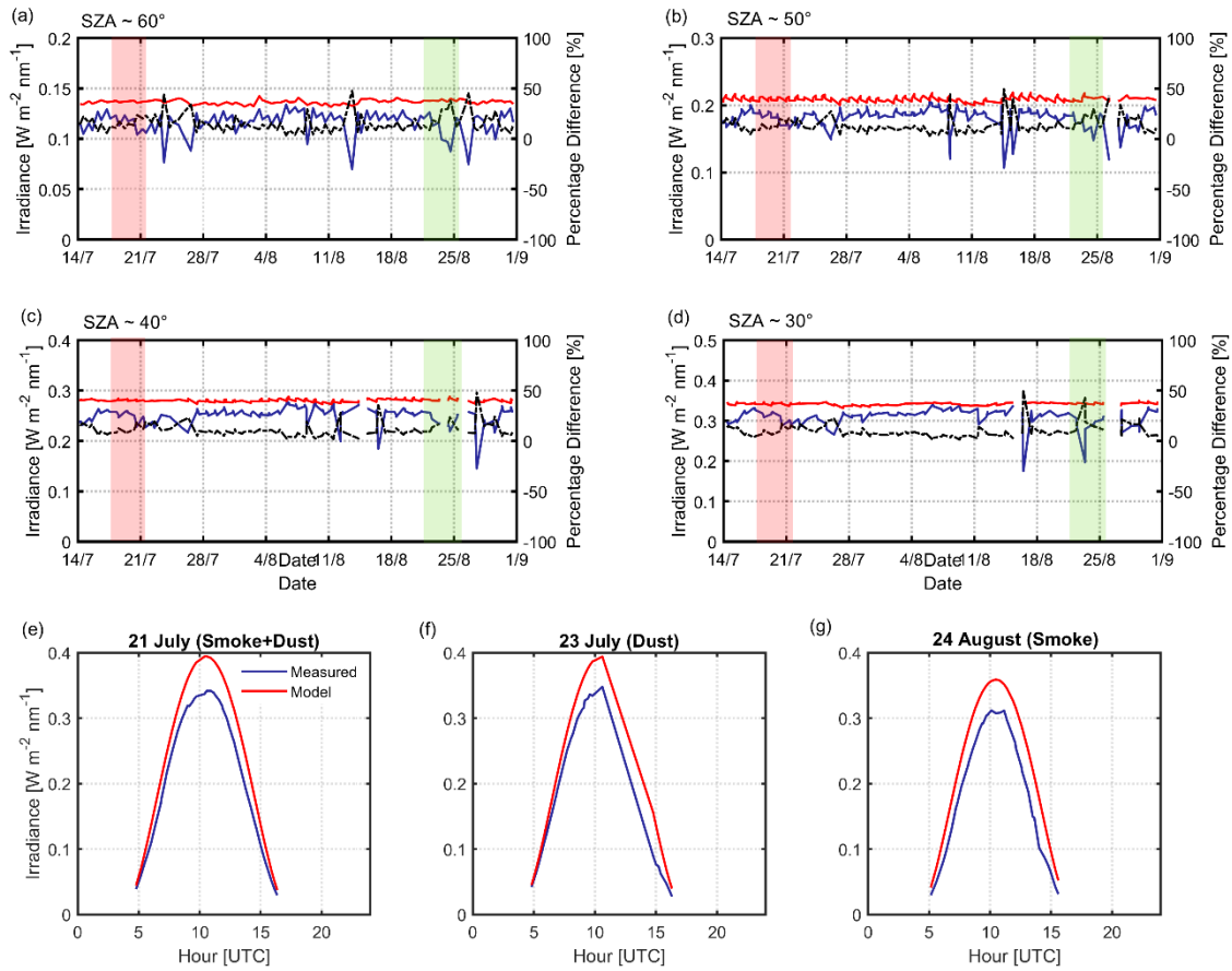
Figure 13. UVB irradiance attenuation at 320 nm for the period 14 July-30 August at SZAs of (a) 60°, (b) 50°, (c) 40°, and (d) 30°, as measured by the Brewer spectroradiometer (blue) and compared with clear-sky simulations from the libRadtran model (red). The percentage difference between observations and model is also shown (black dashed line), as well as the diurnal UVB irradiance at 320 nm for three representative cases: (e) 21 July (smoke + dust), (f) 23 July (dust), and (g) 24 August (smoke), compared to clear-sky values.
