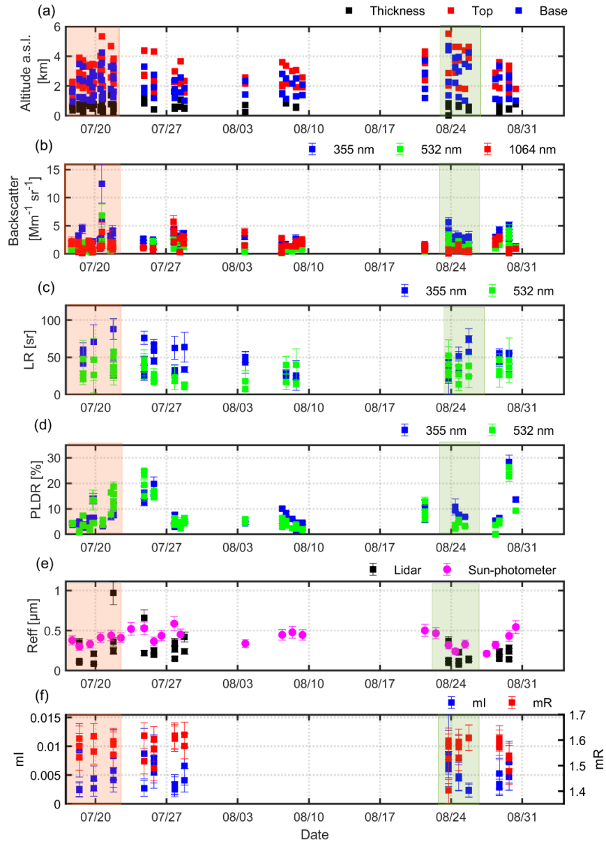
Figure 12. Aerosol geometrical, optical, and microphysical properties retrieved over Athens during the period from 17 July to 30 August 2023: (a) base, top, and thickness off the aerosol layers, (b) backscatter coefficients (355, 532, and 1064 nm), (c) LR (355 and 532 nm), (d) PLDR (355 and 532 nm), (e) Reff, and (f) imaginary (mI) and real (mR) parts of the complex refractive index.
