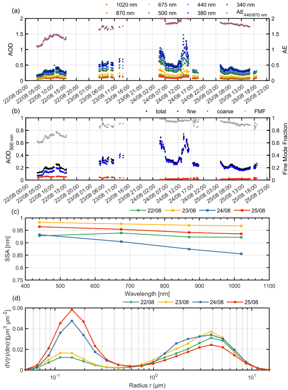
Figure 11. Time-series of values of the (a) AOD for various wavelengths (340 - 1020 nm) and AE at 440/870 nm (b) AOD at 500 nm along with the FMF (c) SSA wavelength dependence and (d) particle volume size distribution obtained by the NTUA CIMEL sun-sky-lunar photometer for the period 22- 25 August 2023.
