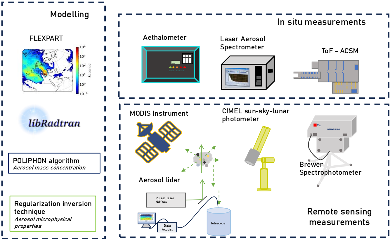
Figure 1. Schematic overview of the instrumentation set-up used in this study. The figure illustrates the integration of multi-platform observations from the NTUA (lidar and photometer), DEM (air quality and aerosol composition), and BRFAA (Brewer spectrophotometer) stations, together with satellite observations (MODIS FIRMS), FLEXPART dispersion modelling, as well as the POLIPHON algorithm and the Regularization inversion technique, highlighting the synergistic use of active and passive remote sensing, in situ data, and modelling tools.
