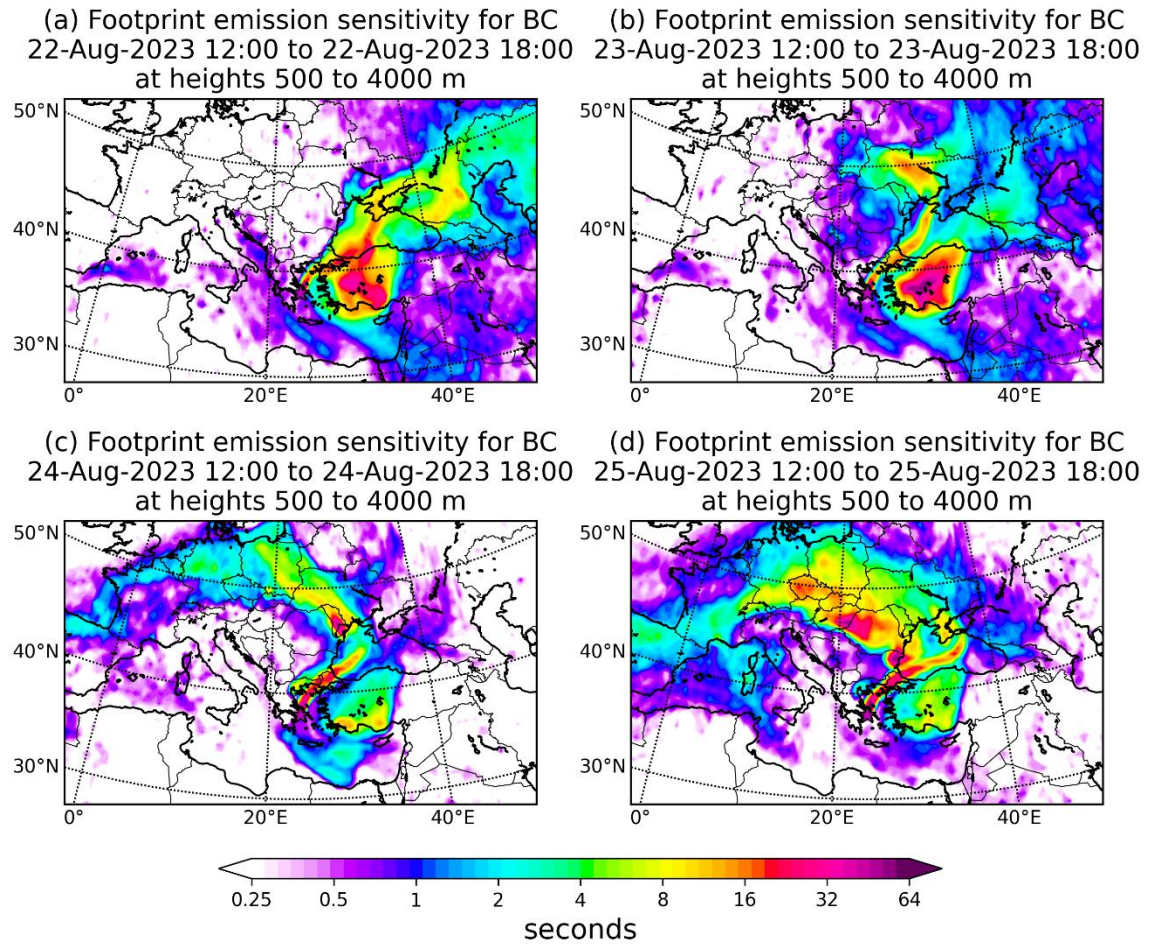
Figure 8. Footprint emission sensitivities for BC obtained using FLEXPART for the air masses arriving over Athens between 0.5 and 4.0 km from 22 to 25 August 2023 (12:00 UTC to 18:00 UTC).
