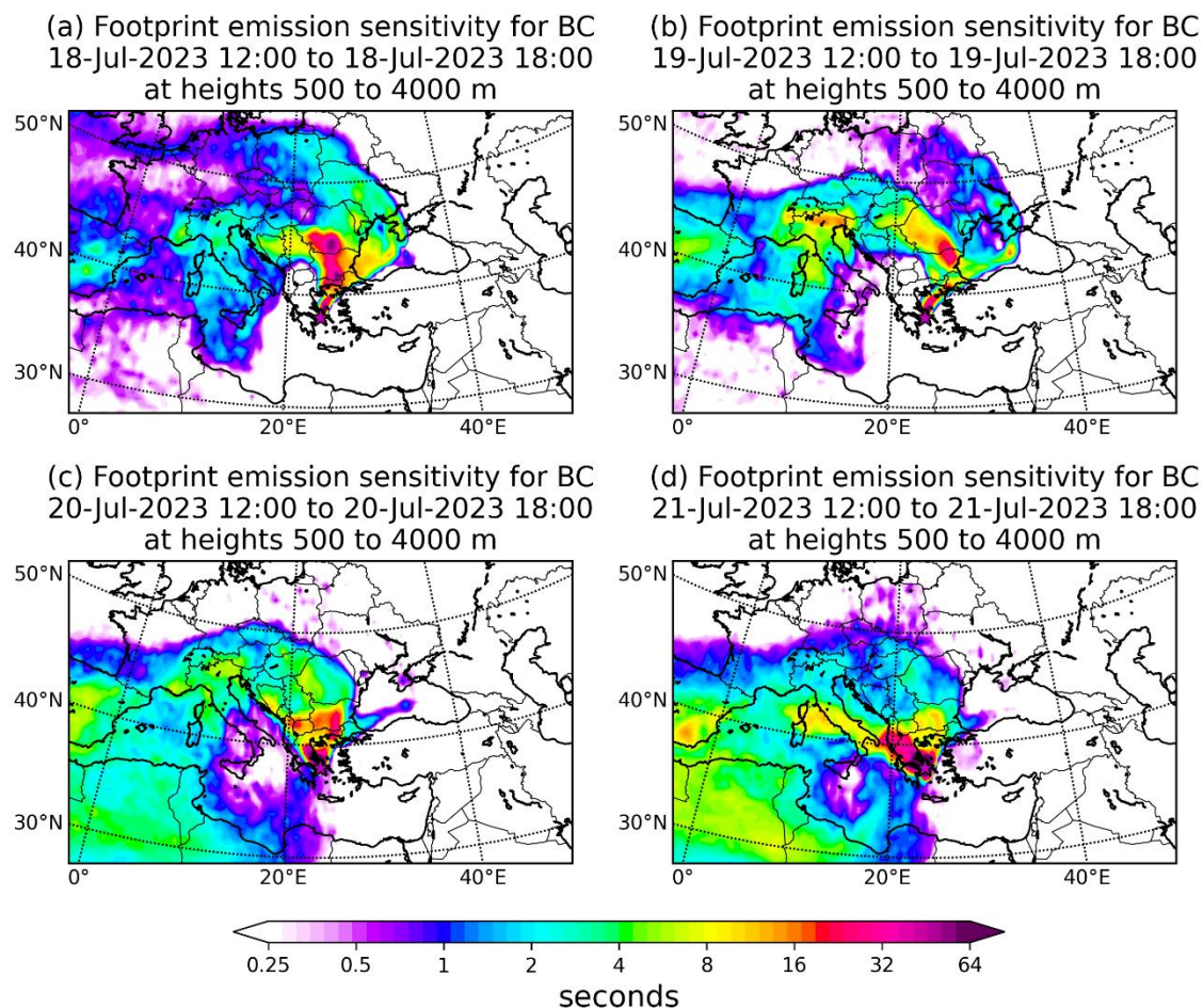
Figure 4. Footprint emission sensitivities for BC calculated using FLEXPART for air masses arriving in Athens between 0.5 and 4.0 km from 18 to 21 July 2023 (12:00 UTC to 18:00 UTC).
