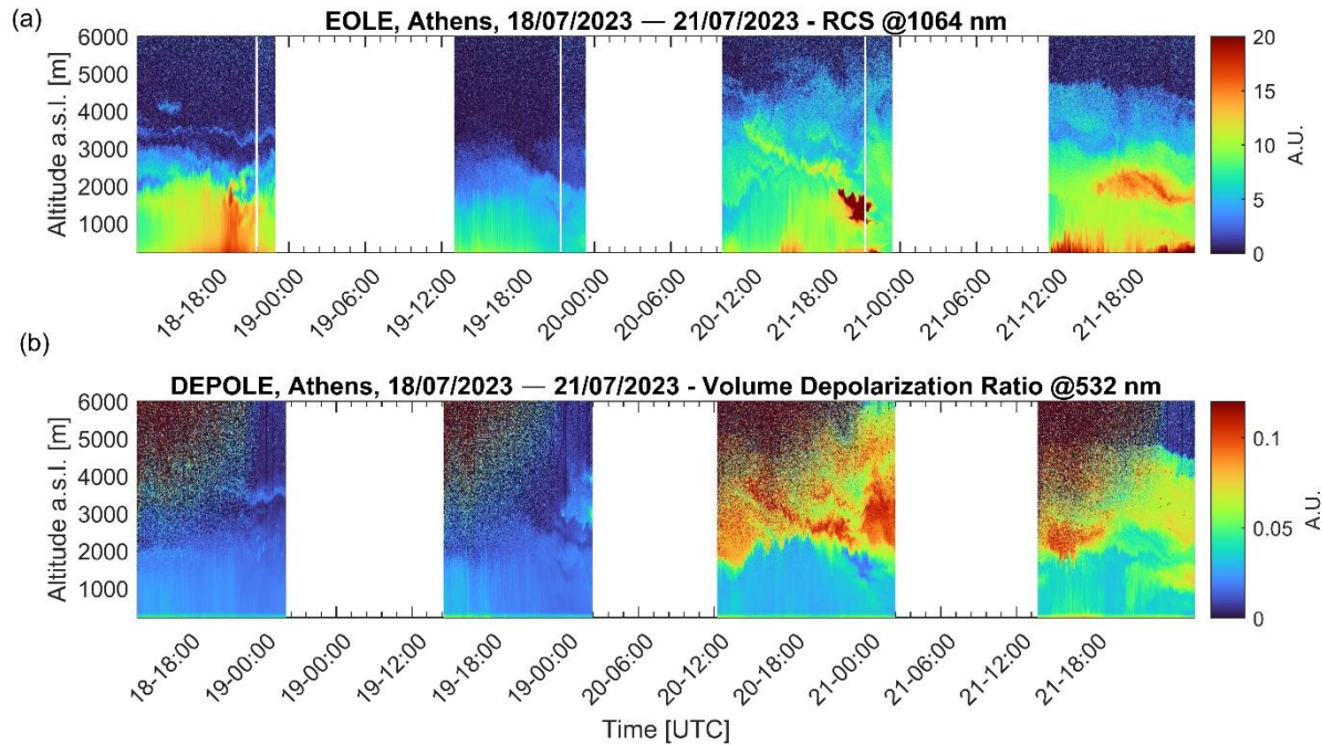
Figure 5. Spatio-temporal evolution of the (a) range-corrected lidar signal (RCS) at 1064 nm and (b) volume depolarization ratio at 532 nm for the period 18-21 July 2023.
