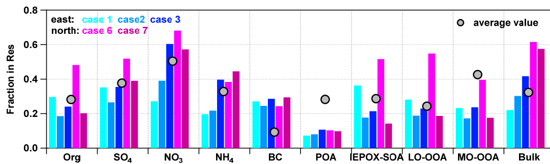
40 Figure S9: Average fraction of chemical components in Res particles during every cloud event in 2023. All cloud events are grouped in colour based on their air masses sources.
