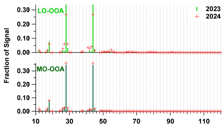
35 Figure S7: Comparison of OA factor spectra (LO-OOA and MO-OOA) resolved in 2023 and 2024.
