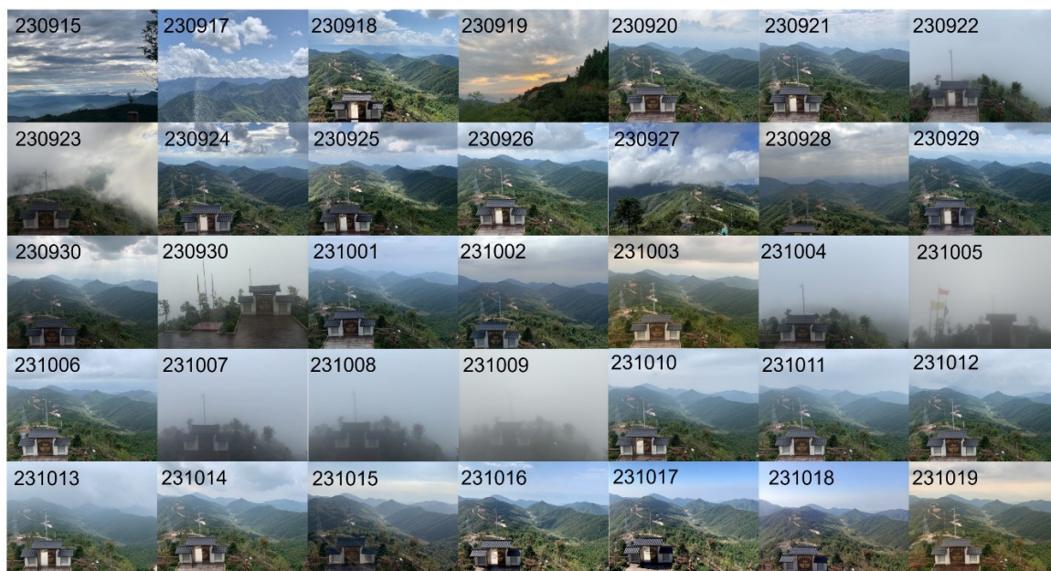
20 Figure S2: Photographic documentation of meteorological conditions during the 2023 field campaign.
