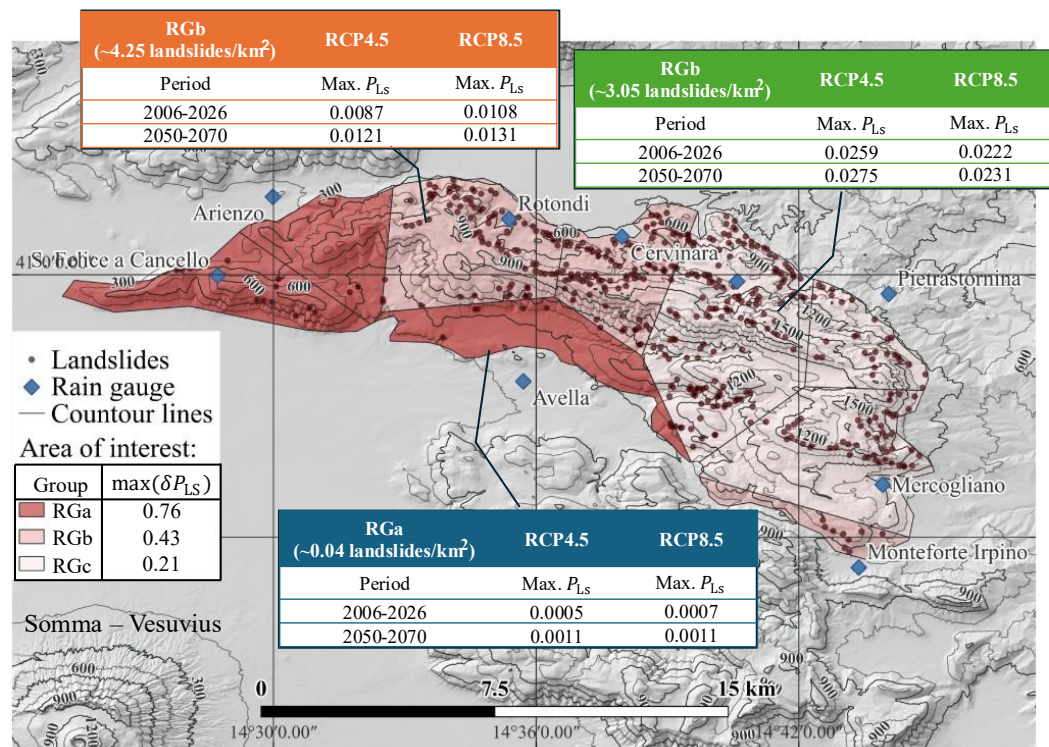
Figure 13. Spatial distribution of the maximum relative change in marginal probability of landslide occurrence ( \Delta P_{LS} ) under the climate change scenarios between 2006-2026 and 2050-2070.
