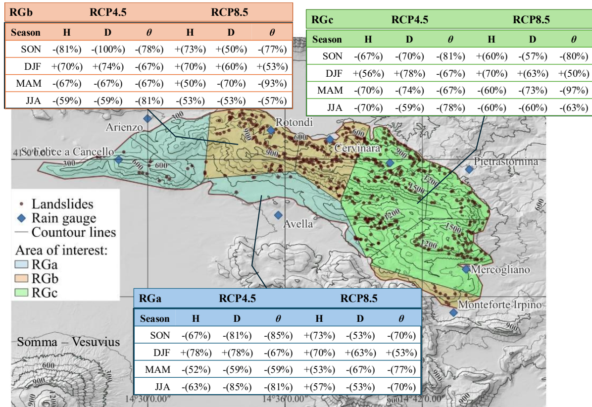
Figure 7. Subregional trend (positive “+” or negative “-”) and percentage of agreement (in brackets) of the ensemble members on rainfall (H), intensity (D) and antecedent volumetric water content (θ), according to RCP4.5 and RCP8.5 climate change scenarios.
