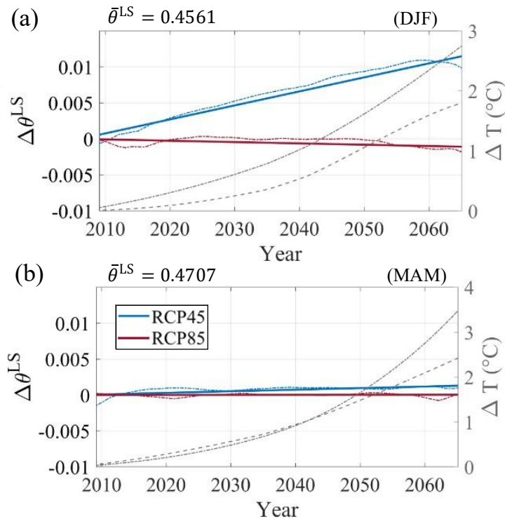
538 539 Figure 12. Anomalies of antecedent volumetric water content ( \Delta\theta^{LS} ) one hour before the onset of triggering rainfall events in DJF 540 (a) and MAM (b).
