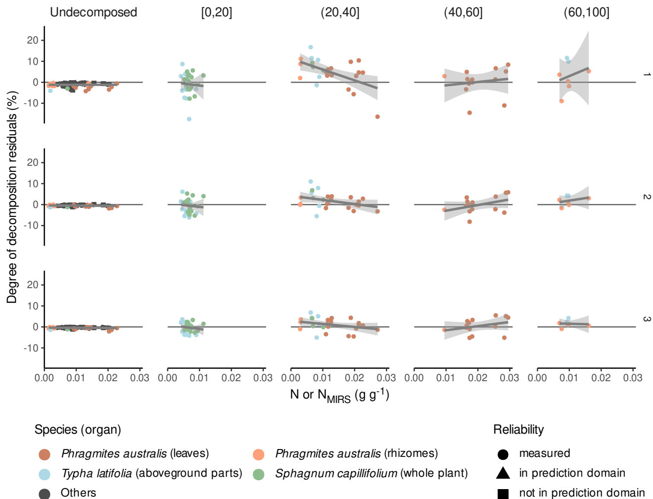
Figure 3. Model residuals (measured \gamma - \gamma_{MIRS} ) versus N or N_{MIRS} for different levels of \gamma (columns) and the three models (rows). Points are averages and lines and shaded areas averages and 95% confidence intervals of regression models fitted to the average residuals. “Reliability” refers to how reliable the N or N_{MIRS} values are. Values of N_{MIRS} are less reliable when they are not in the prediction domain, which is the case only for some of the undecomposed litter samples.
