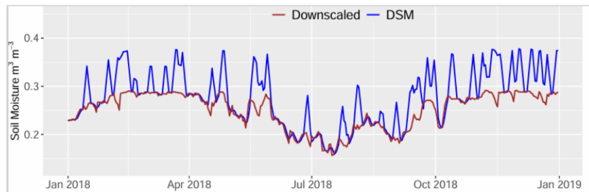
Figure 3: Time series of downscaled (mlhrsm product) and downscaled-bias-corrected soil-moisture (DSM) at the watershed-scale. Data from only one year are shown for clarity.
