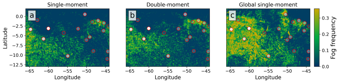
Figure 6. Fog occurrence frequency for (a) the single-moment and (b) double-moment simulations, shown alongside (c) the global single-moment run. Fog occurrence is defined as the fraction of analysed time steps with fog mass mixing ratio exceeding 0.01 \text{ g kg}^{-1} . Overlaid circles (red) represent SYNOP stations, with their filling opacity indicating the normalised observed frequency of fog events (visibility < 1.5 \text{ km} ) during the study period. Higher opacity corresponds to a greater frequency of fog reports.
