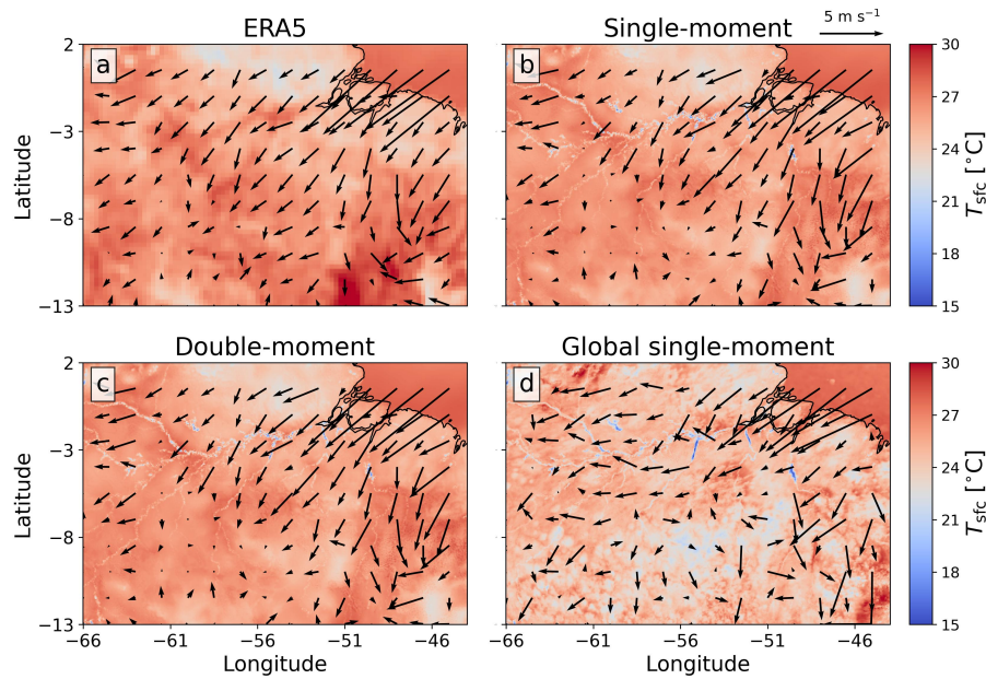
Figure 2. Surface temperature (shading) and wind field (arrows) on 1 February 2020, 00:00 UTC, from (a) the ERA5 reanalysis and (b) the regional single-moment, (c) the regional double-moment, (d) and the global single-moment simulations. The figure illustrates the large-scale differences between the forcing fields used in the regional framework and the freely evolving global simulation.
