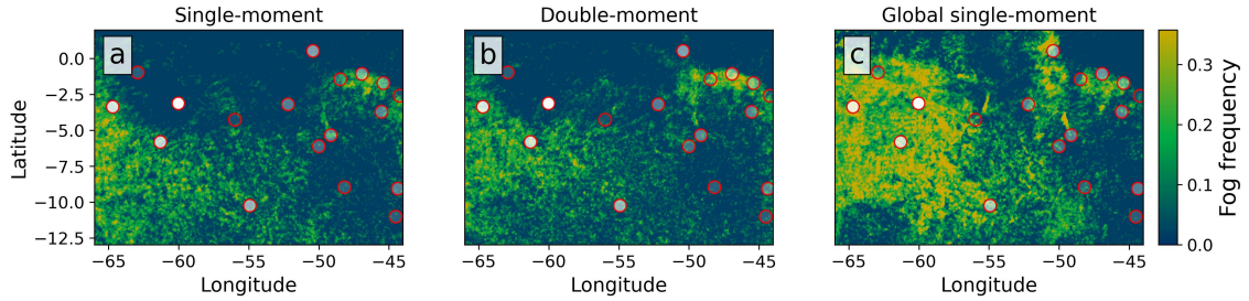
Figure 6. Time-averaged maps of fog mass mixing ratio–Fog occurrence frequency for (a) the single-moment and (b) double-moment simulations, shown alongside (c) the global single-moment run. Fog occurrence is defined as the fraction of analysed time steps with fog mass mixing ratio exceeding 0.01 \text{ g kg}^{-1} . Overlaid circles (red) represent SYNOP stations, with their filling opacity indicating the normalised observed frequency of fog events (visibility < 1.5 \text{ km} ) during the study period. Higher opacity corresponds to a greater frequency of fog reports.
