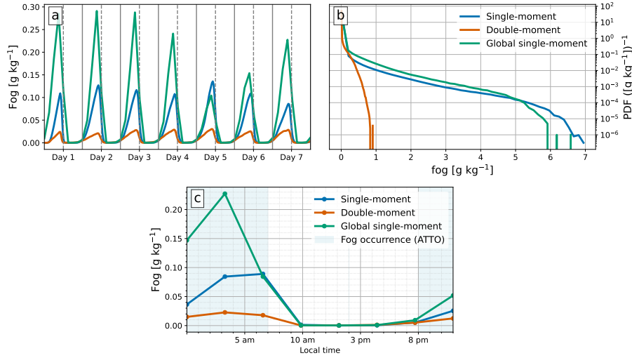
Figure 7. (a) Time-Domain mean time series and, (b) probability density functions, and (c) the mean diurnal cycle of cloud liquid water mixing ratio at the lowest model level (fog) for the regional single-moment (blue) and double-moment (red) simulations, shown alongside the global single-moment run (green). The time series are averaged over In (c), the entire Amazon region blue shading indicates periods when fog was observed by the ATTO ceilometer at least twice during the first week of February between 2022 and experiment duration: 2025.
