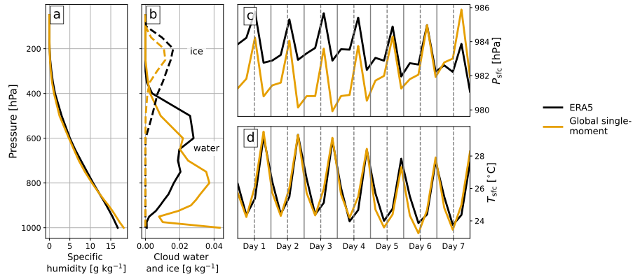
Figure 3. Comparison of the ERA5 lateral boundary conditions forcing applied to both regional simulations (black curves), used to nudge the regional simulations, with corresponding data from the global single-moment simulation (yellow curves) sampled in within the boundary zone. Panels (a) and (b) show the mean vertical profiles of (a) specific humidity and (b) cloud water (solid) and ice (dashed), and panels (c) and (d) show the time series of (c) surface pressure and (d) surface temperature. The figure is intended to characterise differences in the large-scale forcing framework between the regional and global simulations.
