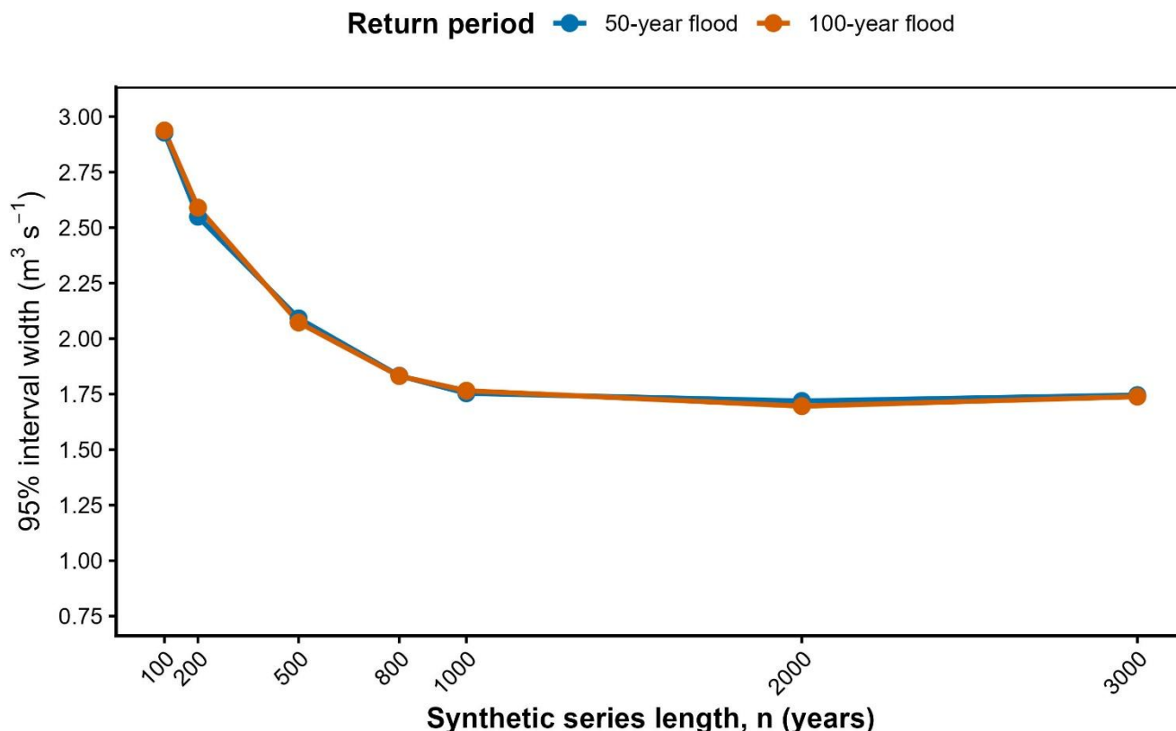
Figure 4. Sensitivity of the UQ-flood 95% interval width to simulated-series length for the 50- and 100-year flood quantiles in the Black River watershed. Interval width is defined as the difference between the 97.5th and 2.5th quantiles across the predictive ensemble.
