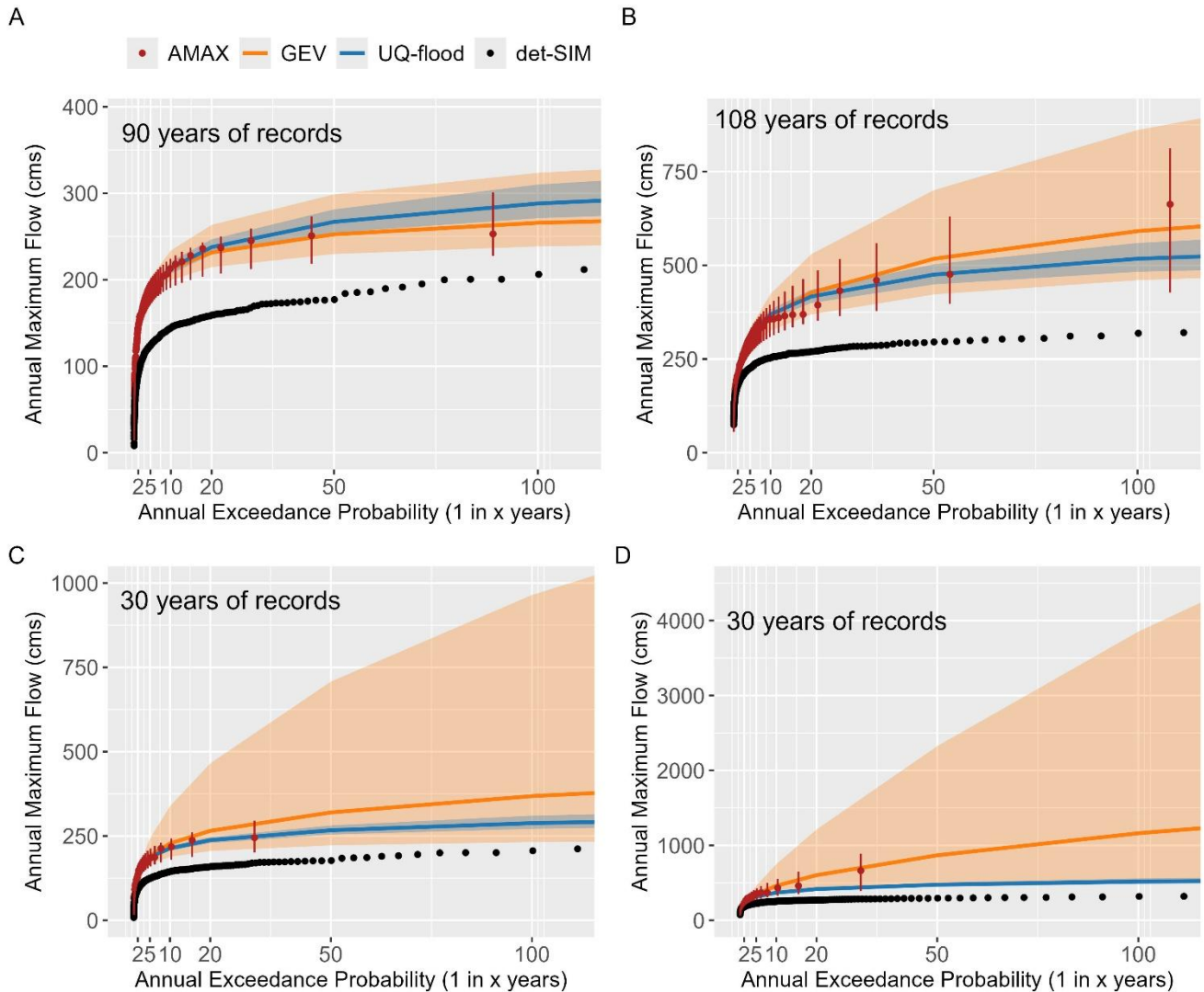
Figure 5: Flood frequency estimates and associated 95% uncertainty intervals for the Moyie River (left panels: A and C) and Lahave River (right panels: B and D) derived using the statistical GEV approach and the UQ-flood framework. The observed annual maximum discharge (AMAX; red) distribution, shown with confidence intervals for discharge quantiles, and the deterministic simulation output (without error model) (det-SIM; black points) are included for reference. The top panel shows GEV results using long-term records (108 years); the bottom panel uses short records (30 years). The UQ-flood framework uses only the 30-year record in both cases
