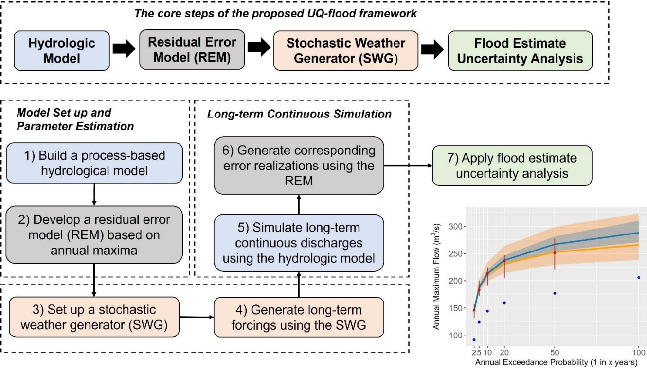
Figure 42: Conceptual diagram of the proposed UQ-flood (Residual Error Model - Flood Frequency Analysis) framework.
