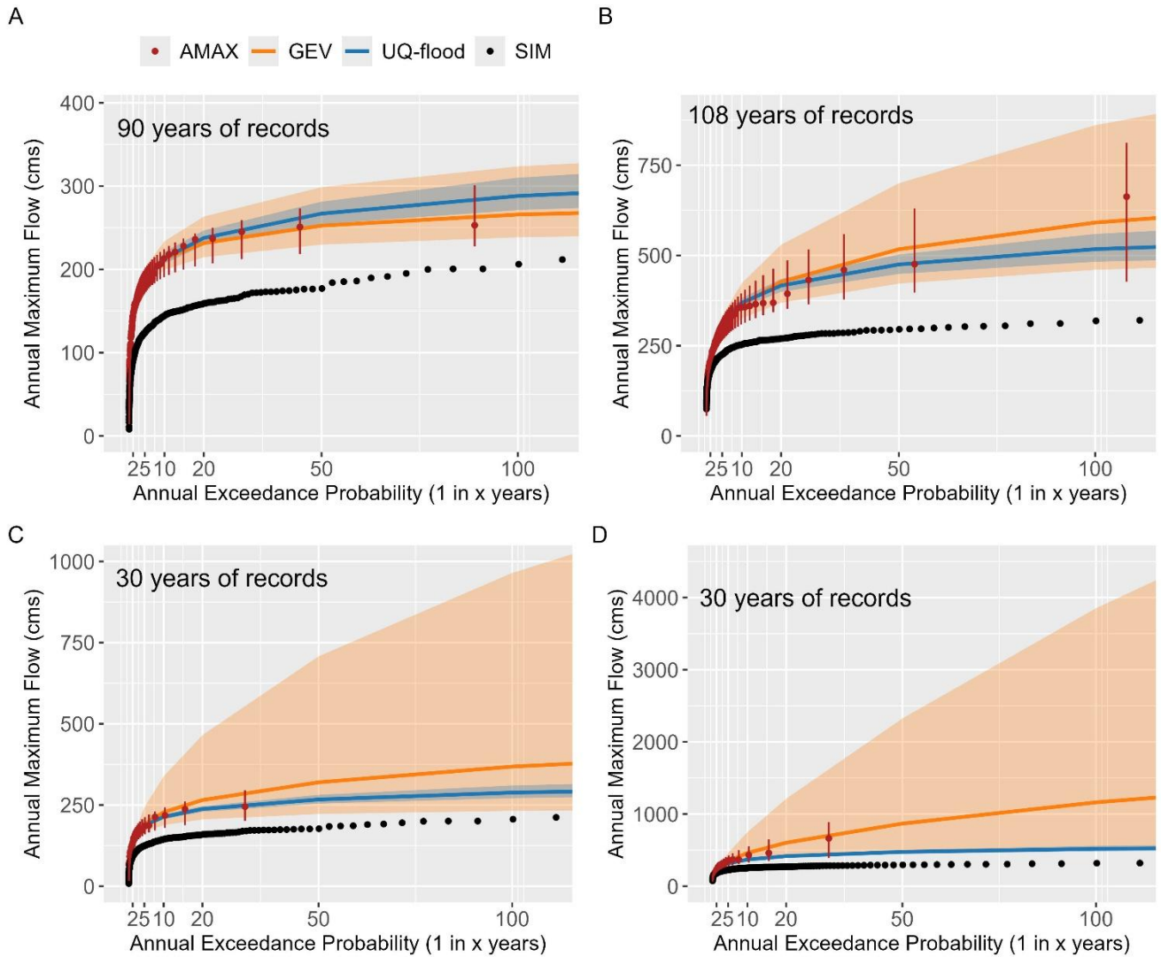
Figure 34: Flood frequency estimates and associated 95% uncertainty intervals for the Movie River (left panels: A and C) and Lahave River (right panels: B and D) derived using the statistical GEV approach and the UQ-flood framework. The observed annual maximum discharge (AMAX; red) distribution, shown with confidence intervals for discharge quantiles, and the deterministic simulation output (SIM; black points) are included for reference. The top panel shows GEV results using long-term records (108 years); the bottom panel uses short records (30 years). The UQ-flood framework uses only the 30-year record in both cases. Flood frequency estimates and 95% uncertainty intervals for the Movie River (left panels: A and C) and Lahave River (right panels: B and D) using a statistical method (GEV) and the UQ-flood framework. AMF_{pp} (red) with plotting position confidence intervals and AMF_{sim} (blue points) are shown for reference. The top panel shows GEV results using long-term records; the bottom panel uses short records (30 years). UQ-flood framework uses only the 30-year record in both cases.
