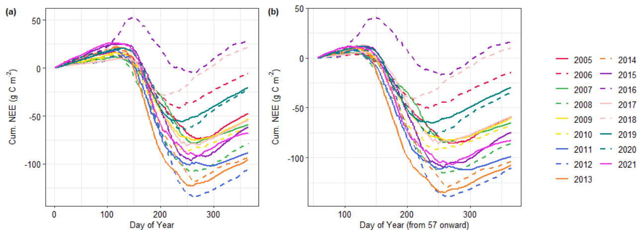
Fig A1. a) Cumulative sums of gap-filled daily sums of net ecosystem exchange of CO 2 (NEE), starting from the day of year( DoY) 1 and b) starting from DoY 57 (B). As 2016 had the highest annual balance, but there was a significant measurement gap in DoY 1-57 in 2016, we calculated the annual sums for all years excluding this period. 2016 remained to have the highest balance, and the relative ranking in the annual balances remained similar. We therefore concluded that the positive balance of 2016 was not a result of the gapfilling period.
