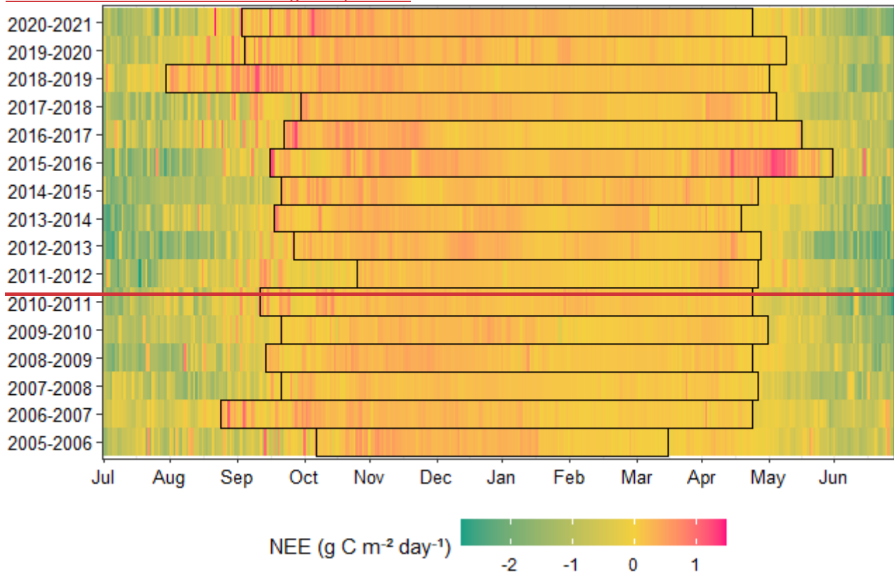
Figure 2. (A) Daily net ecosystem exchange of CO 2 (NEE; g C m -2 day -1 ) in 2005–2021 and the non-growing season (NGS, black rectangular outline) periods centered in the winter. Each row represents one year, beginning in July and ending in June of the following year. Colors indicate daily mean NEE values, where the yellow–green gradient reflects negative values (net carbon sink) and the yellow–pink gradient reflects positive values (net carbon release). Black rectangular outlines mark the NGS periods, defined as the period beginning after the first three consecutive days of positive NEE and ending after the first three consecutive days of negative NEE. On average, the NGS started on September 17th and ended on April 30th.
