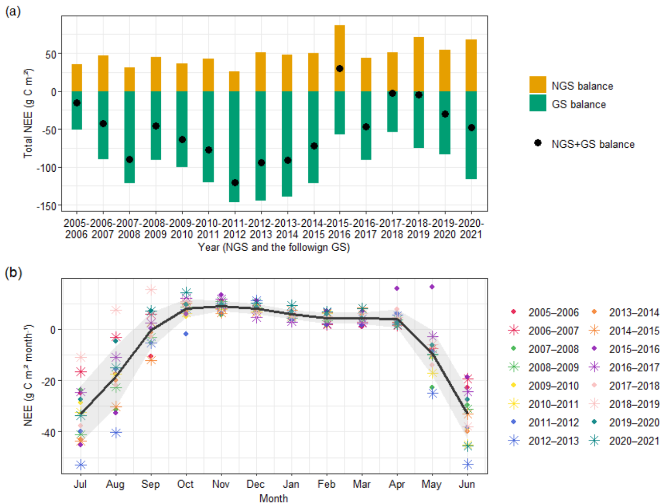
Figure 3. (a) Non-growing season (NGS) and growing season (GS) net ecosystem exchange (NEE) sums of CO 2 for each full NGS and the following GS, with the net balance of the combined period indicated by black points. Negative values indicate a carbon uptake and positive values indicate carbon loss to the atmosphere. We use the terms growing season (GS) and non-growing season (NGS) to refer to periods when the ecosystem acts as a net carbon sink (GS) or a net carbon source (NGS), based on daily NEE values, following the definition for a sink period by Aurela et al. (2004). The start of the NGS is defined as the first of three consecutive days with positive NEE, and the GS begins on the first of three consecutive days with negative NEE. The NGS sum of CO 2 is calculated for the full season, starting in autumn and ending in spring. (b) Monthly NEE sums across the study years, with the mean monthly sums (black line) and standard deviation (shaded area) shown for the period 2005–2021.
