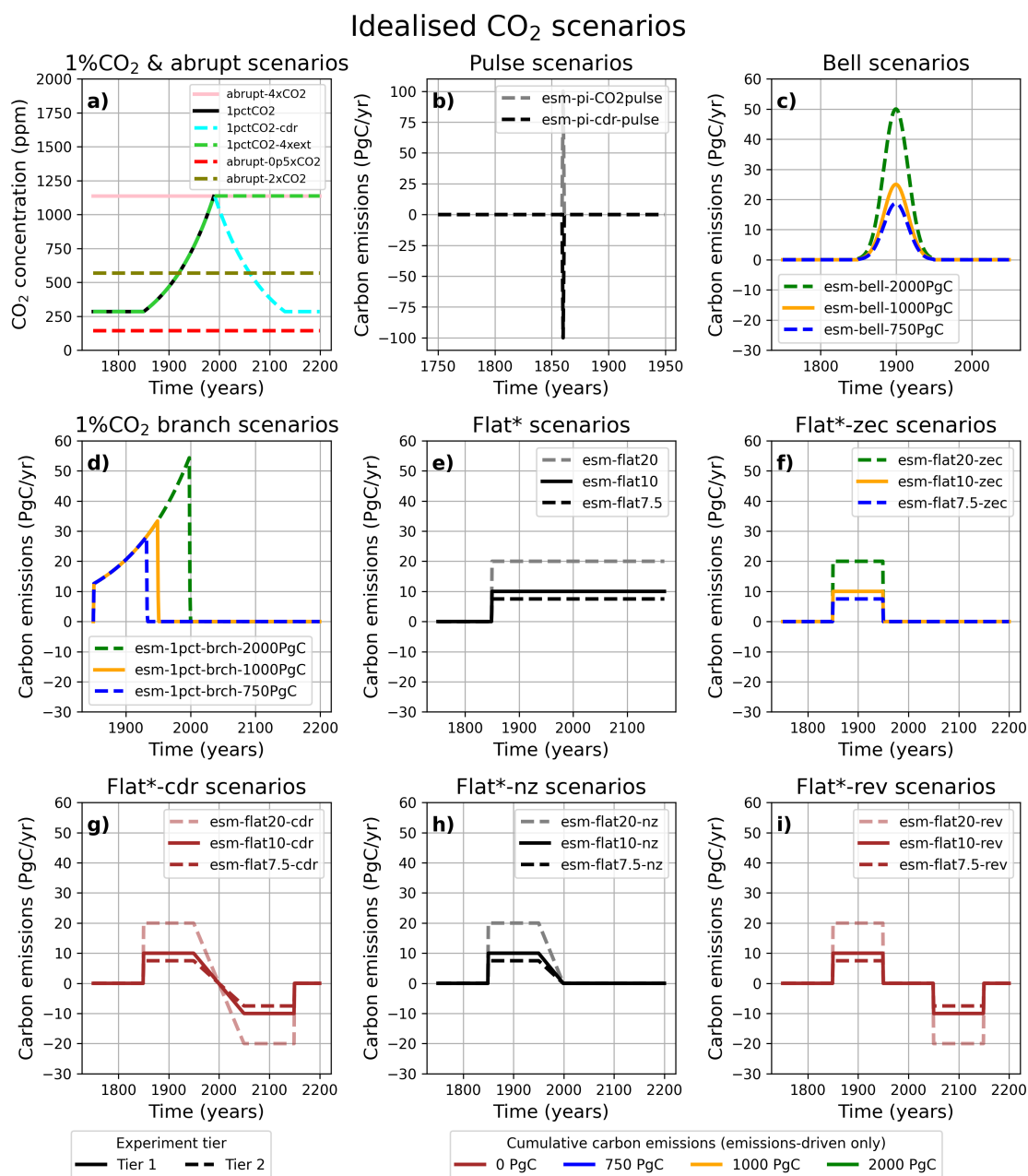
Figure 2. Annual carbon concentrations and emissions as a function of time for the idealized experiments included in RCMIP3. For clarity, flux magnitudes are shown in petagrams of carbon (PgC), although the accompanying dataset provides emissions time series in megatons of CO 2 (MtCO 2 ), consistent with the requested CO 2 emissions variable. Similarly, years in the x -axis are indicative, with the actual requested experiment durations being detailed in Table 1. Line style indicates the experiment tier or running priority (solid for Tier 1 and dashed for Tier 2), while colour (except black) represents the shared cumulative carbon emissions across emissions experiments.
