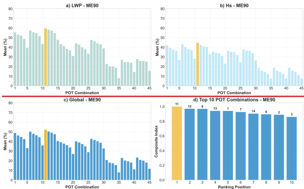
565 Figure 8. Statistical analysis relative to ME90. (a) Mean match of LWP; (b) mean match of wave height. The mean values in (a) and (b) are calculated across all wave conditions and both CV, for each POT combination. (c) Mean match between LWP and wave height; (d) TOP 10 of combinations ranked by the Composite Index (CI), with the combination number indicated above each bar.
