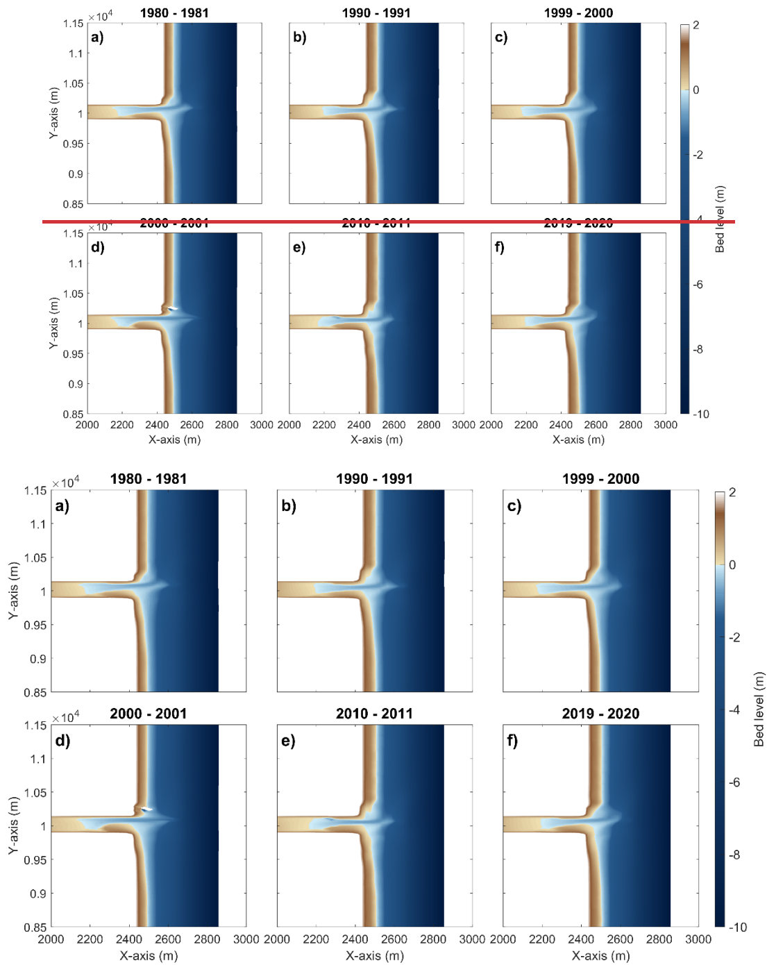
Figure 3. Final bathymetries obtained for each simulation: (a) 1980-81, (b) 1990-91, (c) 1999-2000, (d) 2000-01, (e) 2010-11 and (f) 2019-20
