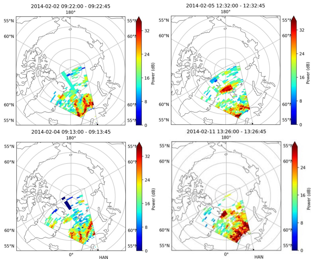
Figure S1. Shows few examples of MSTIDs with different orientations in the Hankasalmi radar FAN plots.
