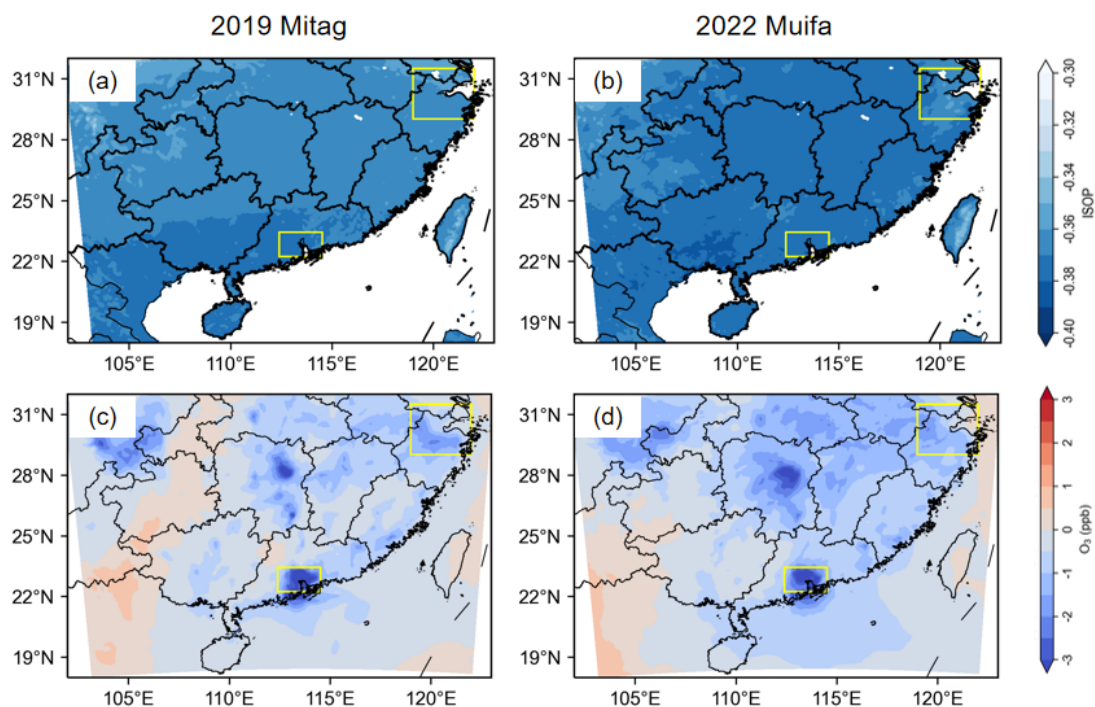
440 Figure 13: Variability rate of ISOP caused by radiation changes during two ozone pollution episodes (a and b). Changes in ozone concentration due to reduced BVOCs emissions resulting from decreased solar radiation (c and d).
