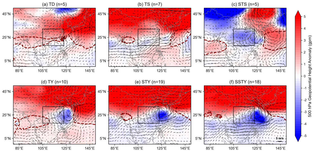
Figure 6: Composites anomalies of 500 hPa geopotential height (color shade) and 850 hPa wind fields (wind arrow) under different intensities of northward TCs within the key subregion relative to the autumn climatology. The dark red dashed lines represent the mean position of the WPSH.
