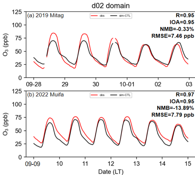
370 Figure 8: Hourly variations and statistical metrics of ozone in observed values (red line) compared to model simulations (black line) for SEC (d02 domain) from two ozone episodes.
