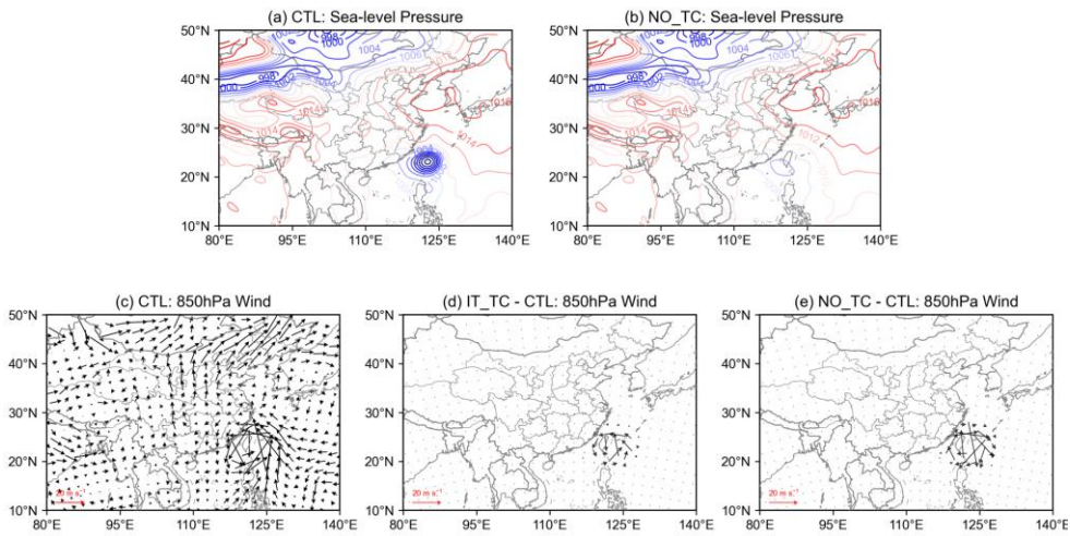
Figure 2: Meteorological fields at 14:00 on 30 September 2019. Sea level pressure field for the CTL (a) and the NO_TC (b). Differences with the CTL (c) in the IT_TC (d) and the NO_TC (e) of the 850 hPa wind field.
