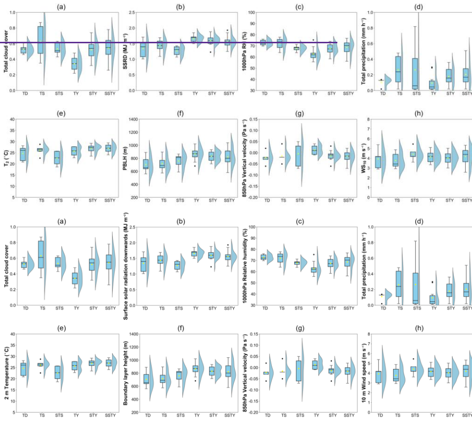
Figure 5: Comparison of meteorological conditions between among different intensities of northward TCs within the key subregion. (a–h) represent total cloud cover, surface solar radiation, 1000 hPa relative humidity, total precipitation, 2 m temperature,
