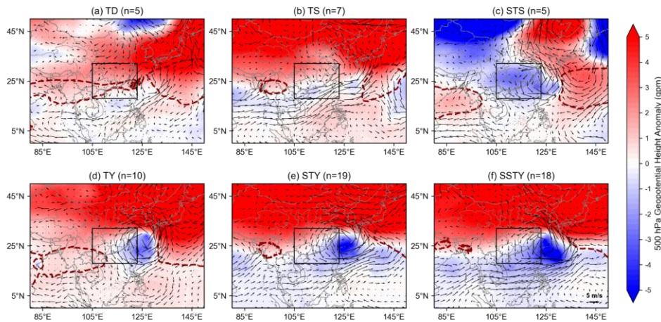
Figure 6: Composites anomalies of 500 hPa geopotential height (color shade) and 850 hPa wind fields (wind arrow) under different intensities of northward TCs within the key subregion relative to the autumn climatology. The dark red dashed lines represents the mean position of the WPSH.
