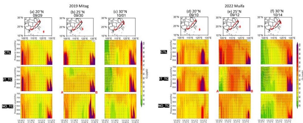
430 Figure 12: Vertical distribution of ozone concentration (contours) and atmospheric circulation (wind vectors) over SEC (along the cross-section marked by the red line in the top-row panels) at 14:00 on the days with similar TC positions during the two episodes.
