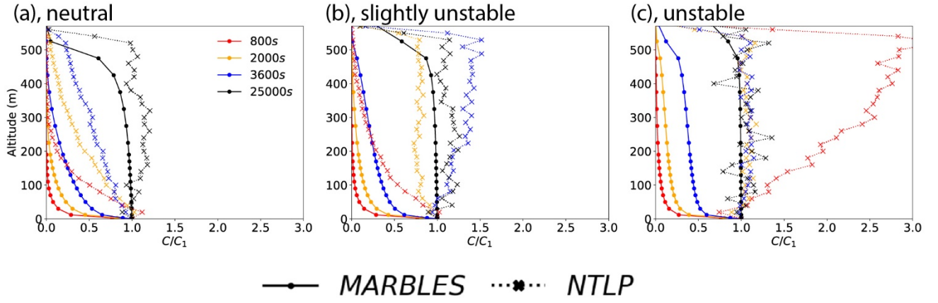
585 Figure 10. Comparison of vertical concentration profiles between Lagrangian NTLP (dotted lines) and 1-D MARBLES (solid lines) for the benchmark cases (a) neutral, (b) slightly unstable, and (c) unstable cases using the turbulent mixing coefficients from the parameterization proposed by Nissanka et al. 2018 (Equation 11) obtained using NTLP input variables. Profiles are normalized by C_1 , the concentration at the first grid point.
