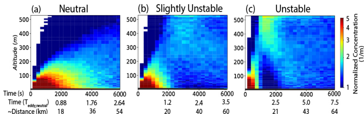
400 Figure 5. Time-height evolution of normalized particle concentration for the three baseline cases: (a) neutral, (b) slightly unstable, and (c) unstable conditions, over 6000 seconds. The bottom axes show time in seconds, corresponding time in eddy turnover times and horizontal transport distance assuming 12 m/s of geostrophic wind speed.
