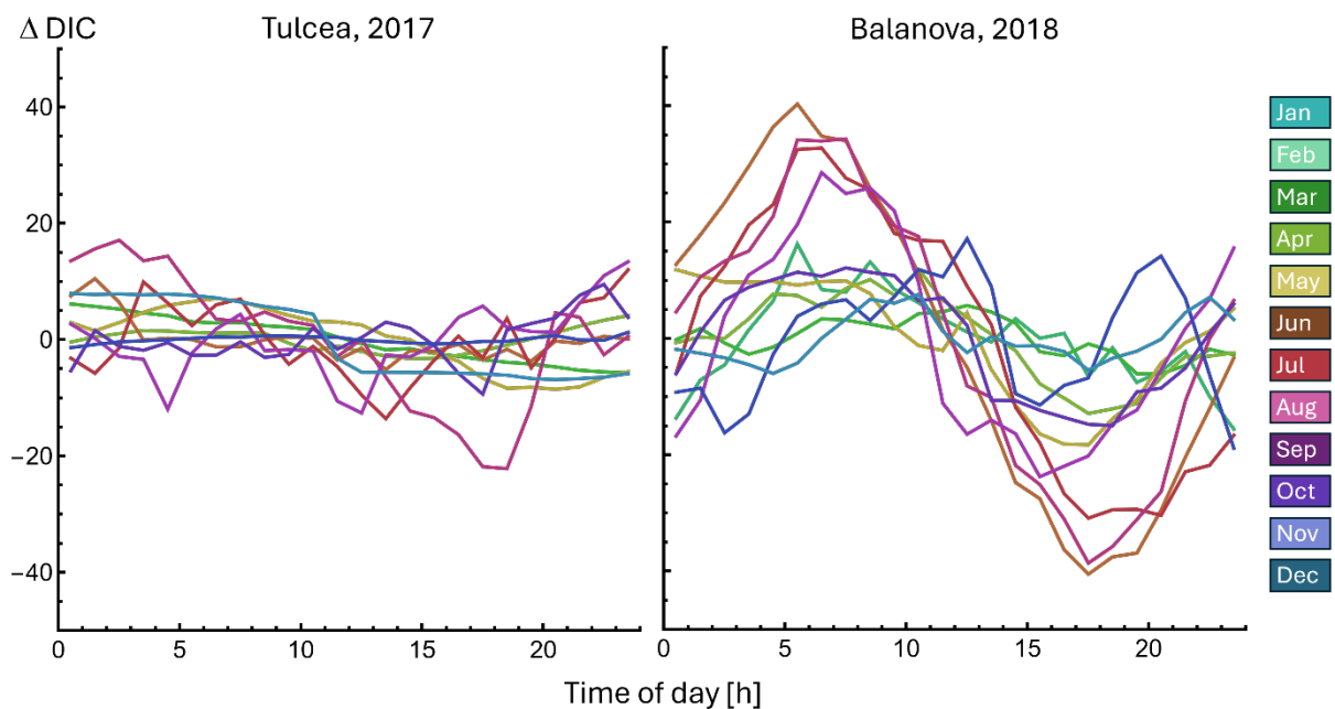
Figure C2 Example of 24-h monthly averages for DIC at Tulcea from March to December 2017 and at Balanova station from February to December 2018. The DIC cycles show stronger random variability compared to the \text{exO}_2 and \text{exCO}_2 cycles in Fig 3. Rapid changes in DIC at monthly timescales are likely and important source of this stochasticity (Fig C1).
