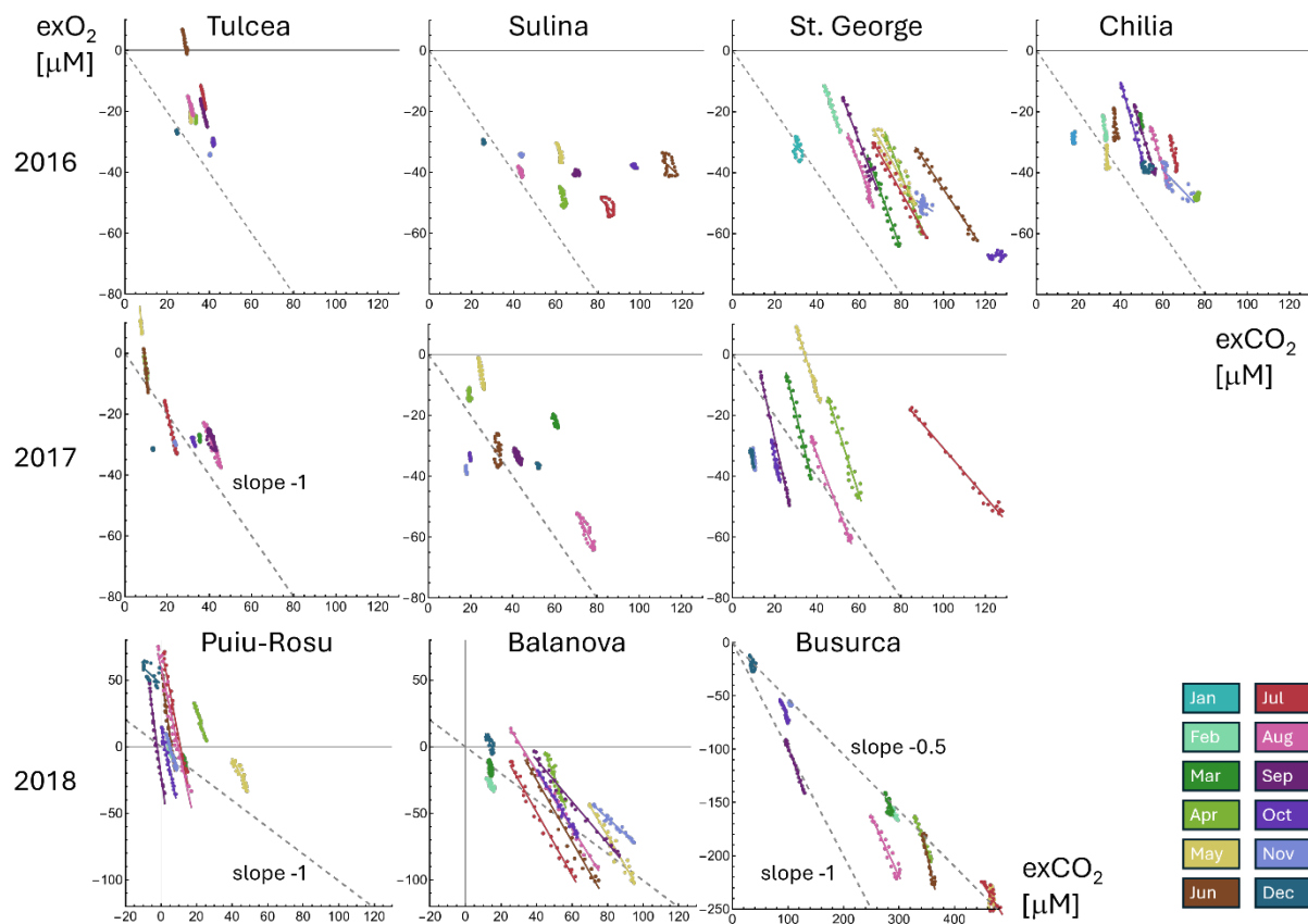
330 Figure 5. Paired exO_2 - exCO_2 plots of mean 24-h cycles. Dots represent monthly averages at one hour resolution and are connected by linear regression lines. Diagonals mark theoretical O_2 - CO_2 stoichiometry of photosynthesis and respiration. Note extended x-y scale at Busurca.
