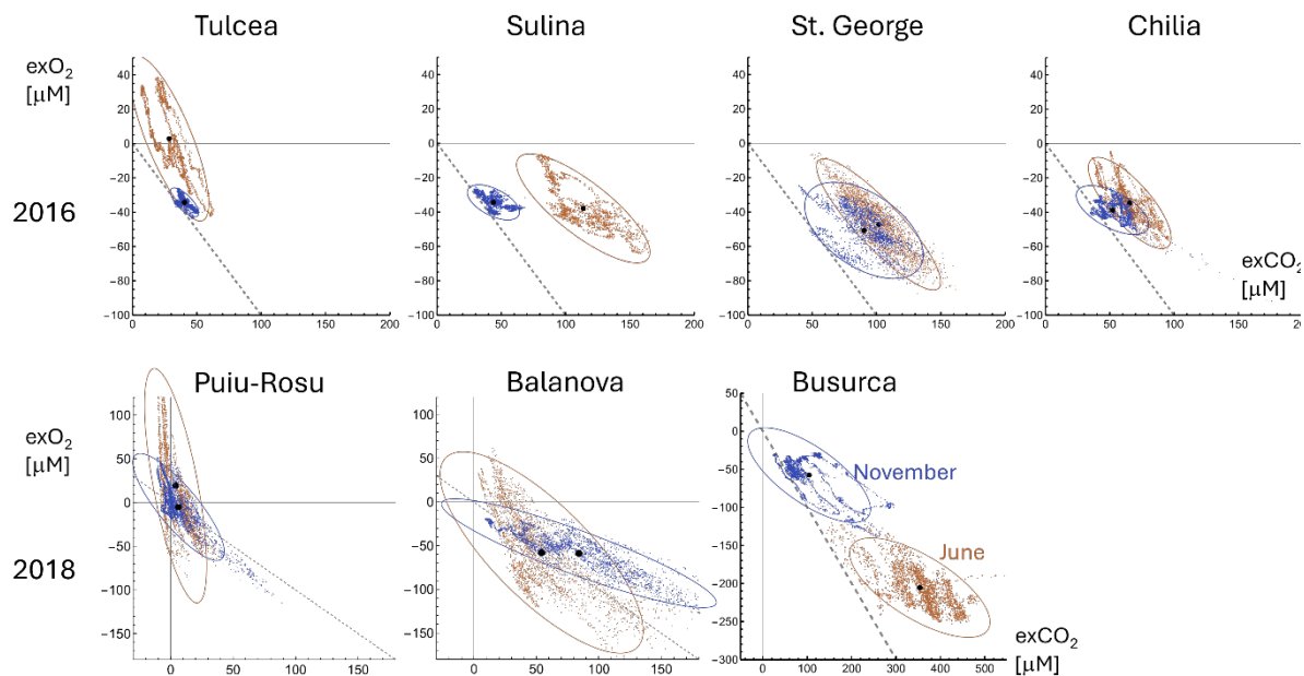
Figure 6. Examples of covariance ellipses for exO_2 - exCO_2 data pairs at 95% confidence level for the Danube River reaches (upper panels) and stations within the delta (lower panels). Diagonal lines represent the theoretical slope of -1 for photosynthesis and respiration. Dots mark the centroids. Expanded axes for Busurca.
