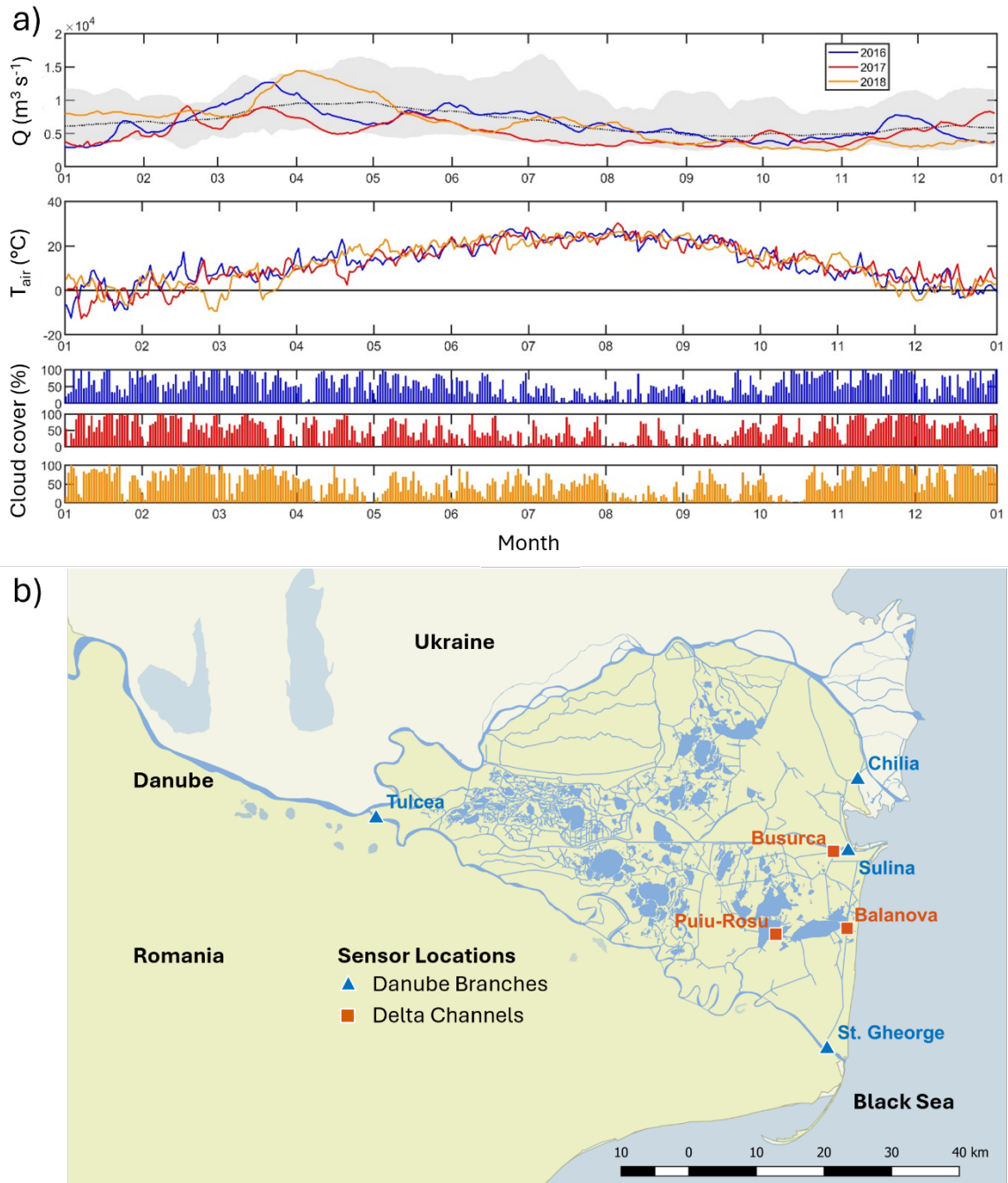
Figure 1a) –Three years of environmental records for the Danube Delta 2016-2018. Top: mean daily discharge of the Danube at Reni, Ukraine, upstream of the Delta (available at https://www.danubehis.org/stations - last access 27. Oct. 2025). Gray area indicates the range of daily discharge for the period 1998-2017. Middle: average daily air temperature; bottom: average daily cloud cover at Tulcea Airport (available at https://rp5.lv/Weather_in_Tulcea_(airport) – last access 27. Oct. 2025). b) Monitoring locations for EXO2 probes in main branches and within the Danube Delta. Map: © OpenStreetMap contributors 2024. Distributed under the Open Data Commons Open Database License (ODbL) v1.0.
