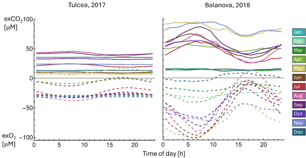
Figure 3. Examples of 24-h monthly averages of \text{exCO}_2 (solid lines) and \text{exO}_2 (dashed lines) at Tulcea from March to December 2017 and at Balanova station from February to December 2018. The averaged daily cycles define characteristic amplitudes and timing of river metabolism for each month. See Fig. C2 for corresponding 24-cycles of DIC.
