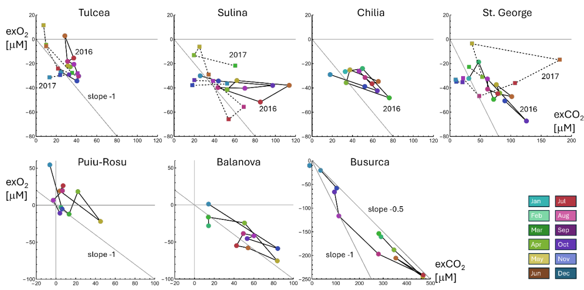
Figure 7. Top: Annual trajectories of monthly centroids at the four Danube River stations in 2016 and 2017. Extended x-axis for St. George. Bottom: Monthly centroids at three stations within the Danube Delta in 2018. Extended x-y axes for Busurca.
