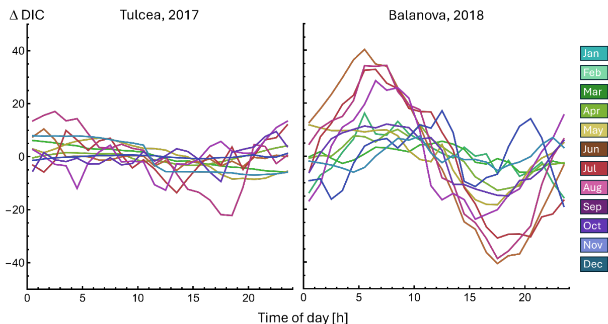
670 Figure C2 Example of 24-h monthly averages for DIC at Tulcea from March to December 2017 and at Balanova station from February to December 2018. The DIC cycles show stronger random variability compared to the \text{exO}_2 and \text{exCO}_2 cycles in Fig 3. Rapid changes in DIC at monthly timescales are likely and important source of this stochasticity (Fig C1).
