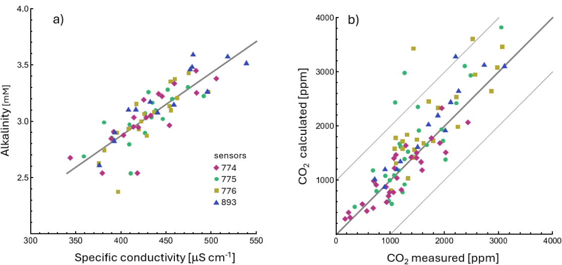
Figure B1 a) Linear regression of alkalinity analyses from water samples versus specific conductivity. The specific conductivity recorded by the EXO2 sensors was correlated with alkalinity measurements obtained from titration analysis of water samples taken at the same time and location. Labels mark the four different EXO-2 probes. Alkalinity [mM] = 0.0057 \times \text{specific conductivity } [\mu\text{S cm}^{-1}] + 0.60 , with a correlation coefficient of R^2 = 0.70 . b). Measured CO 2 data based on the headspace technique compared to dissolved CO 2 calculated from EXO2 data. Alkalinity was estimated by correlation (panel a) and pH plus temperature records were combined to calculate dissolved CO 2 . With few exceptions, the CO 2 estimates compared well with direct CO 2 measurements ( R^2 = 0.82 ). Diagonal marks the 1:1 relationship with lines at \pm 1000 ppm. Symbols represent the same sensors as in panel a).
