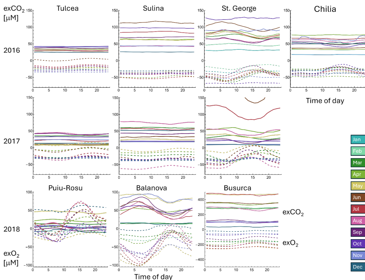
680 Figure D1. Monthly averaged time-of-day plots showing \text{exCO}_2 (solid lines) and \text{exO}_2 (dashed) during 2016 and 2017 at the Danube stations during 2018 at the Delta stations. Extended y-axis for Busurca.
