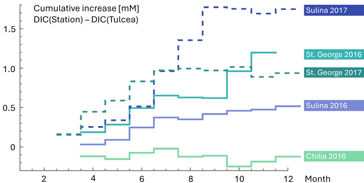
675 Figure C3 Cumulative increase in DIC concentration during seasonal cycles calculated from the difference between the mean monthly DIC at a station and the upstream data at Tulcea.
