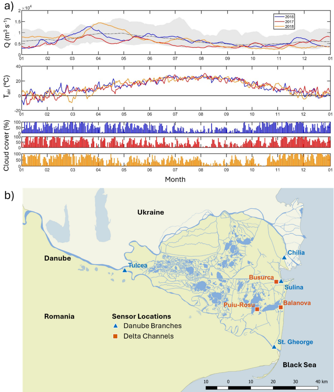
175 Figure 1a) –Three years of environmental records for the Danube Delta 2016-2018. Top: mean daily discharge of the Danube at Reni, Ukraine, upstream of the Delta (available at https://www.danubehis.org/stations - last access 27. Oct. 2025). Gray area indicates the range of daily discharge for the period 1998-2017. Middle: average daily air temperature; bottom: average daily cloud cover at Tulcea Airport (available at https://rp5.lv/Weather_in_Tulcea_(airport) – last access 27. Oct. 2025). b) Monitoring locations for EXO2 probes 180 in main branches and within the Danube Delta. Map: © OpenStreetMap contributors 2024. Distributed under the Open Data Commons Open Database License (ODbL) v1.0.
