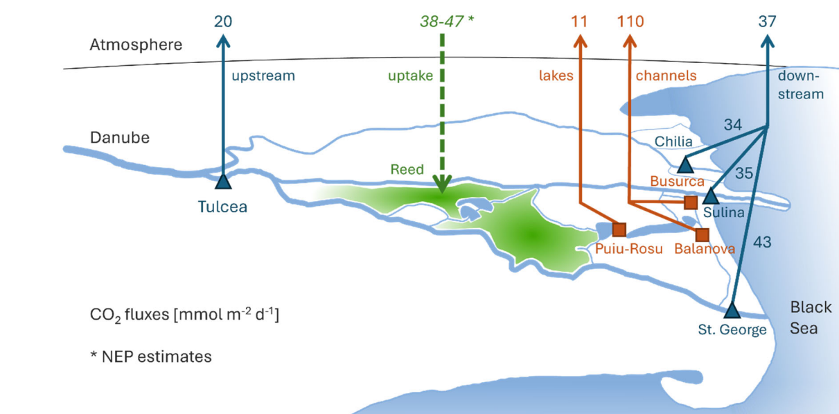
Figure 8. Schematic overview of average CO 2 emission rates in main river reaches upstream and downstream of the Danube Delta for 2016-2017 compared to stations within the delta in 2018 and global median net ecosystem production (NEP) uptake by wetlands from Li et al. (2025) and Lu et al. (2017).
