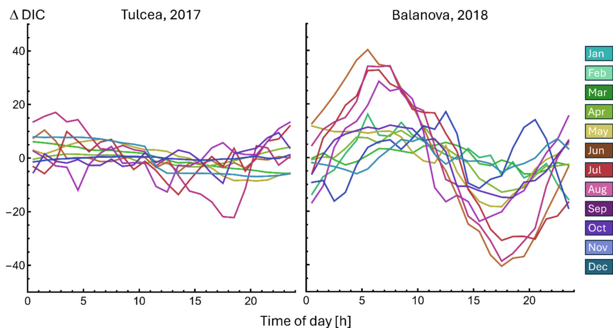
Figure C2 Example of 24-h monthly averages for DIC at Tulcea from March to December 2017 and at Balanova station from February to December 2018. The DIC cycles show stronger random variability compared to the \text{exO}_2 and \text{exCO}_2 cycles in Fig 3. Rapid changes in DIC at monthly timescales are likely and important source of this stochasticity (Fig C1).
