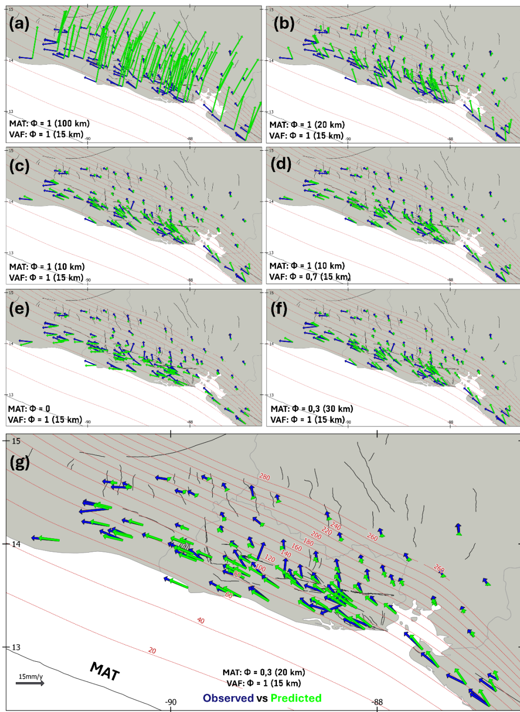
455 Figure 7: Observed horizontal GNSS velocities (blue vectors) vs. predicted horizontal velocities (green vectors) in several forward models with different parameters. Faults are represented as black lines. Red lines show the subduction slab contours (with the depth in km labelled in red).
