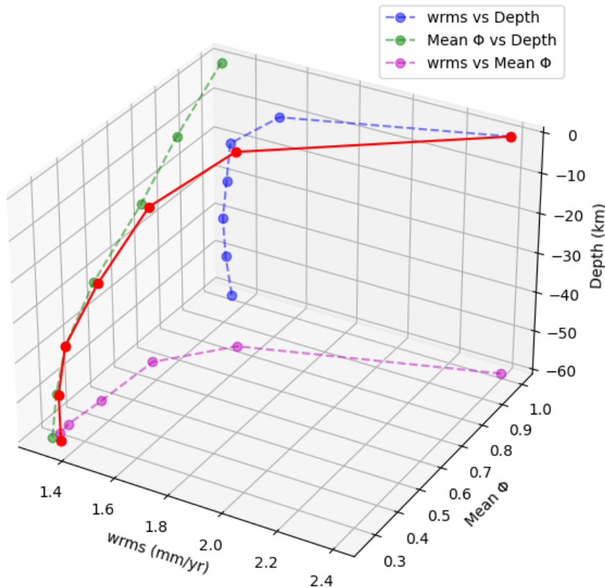
535 Figure 8: Detected trade-offs between several parameters of the model: the maximum depth at which we let the slab to be coupled, the wrms of the geodetic data, and the mean predicted coupling ( \Phi ) in the slab in the model. The red line shows the combined relationship.
