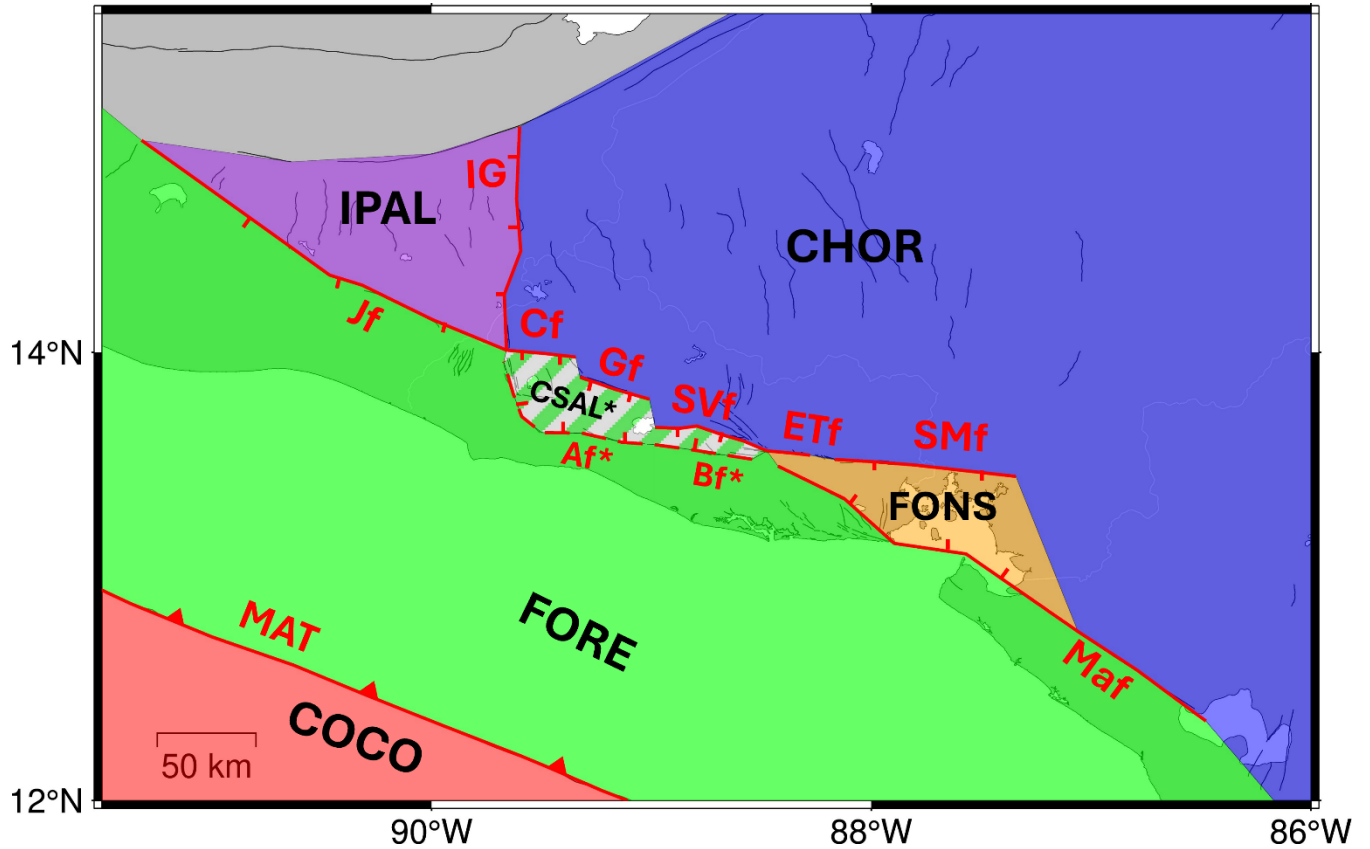
Figure 3: Block geometry defined for the kinematic models. Inverted block limits are shown as red lines (and labelled following faults and structures in Fig. 1). The CSAL block and the Af and Bf faults are marked with an asterisk, indicating that we also present models in which the CSAL block is tied to the FORE block and, consequently, these faults are not inverted.
