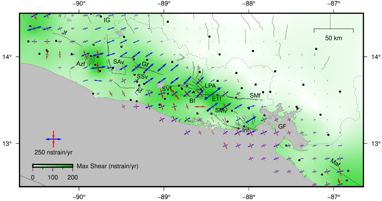
240 Figure 4: Strain rate tensors (crosses) and maximum shear strain rates. Main faults (black lines) are labelled following Fig. 1. The dots represent the location of the GNSS stations used for the strain determination.
