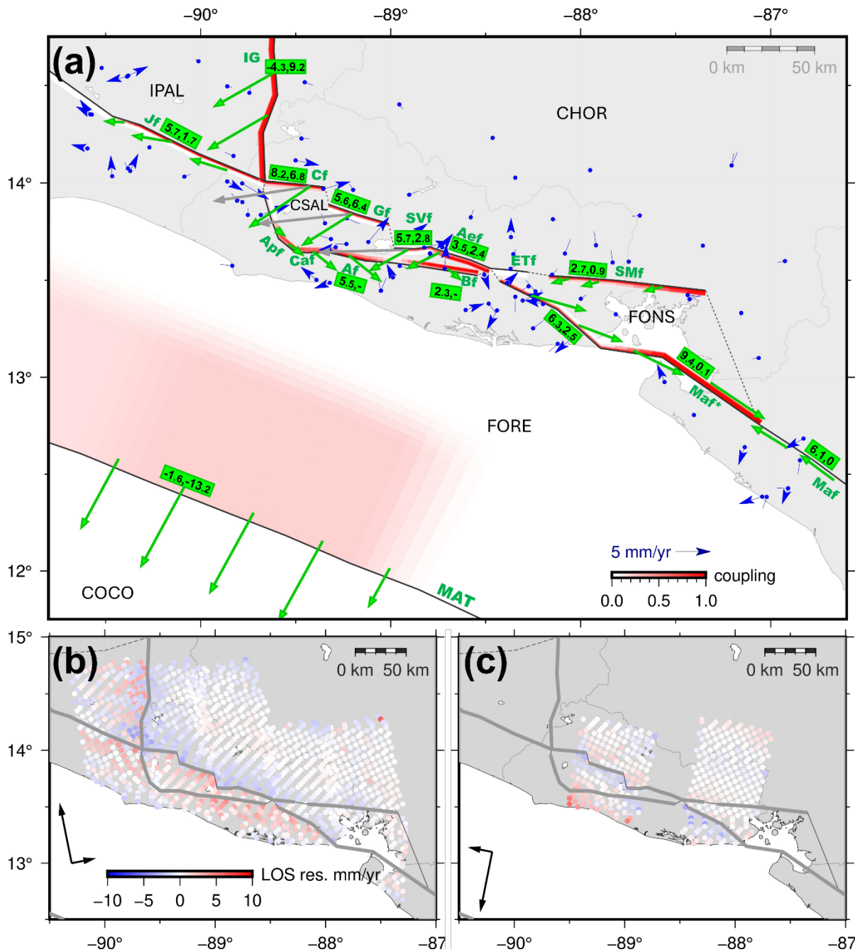
275 Figure 5: Preferred kinematic model results for the ESFZ. A: GNSS residuals (blue vectors) and resulting slip rates for each fault or segment, represented as green arrows (located on the hanging walls and slightly displaced from the center of each segment) and with the fault-parallel and fault-normal slip rates in green rectangles, in mm/yr (negative values for sinistral and reverse slip rates). Faults are represented as planes, coloured by their predicted coupling ratio. The grey dashed lines represent the block boundaries that were not inverted (i.e., they were forced to creep). The blocks are named in black (Fig. 3). We also show the ALOS LOS ascending (subpanel b) and descending (subpanel c) residuals of the model. 280
