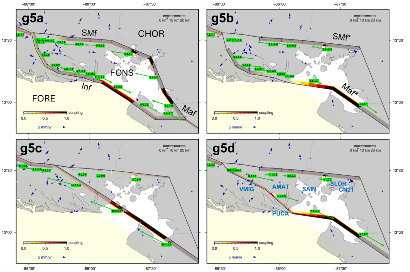
Figure 6: Different geometries tested for the Fonseca block (FONS) in the inversions. Slip rates are shown as green vectors, labelled with their respective slip rates (fault-parallel, fault-orthogonal). Negative values (-) indicate sinistral and reverse slip rates, respectively. The inverted coupling ratio at the nodes and along the faults is also displayed. The residuals (observed minus calculated velocities in the model) of the GNSS horizontal velocities are represented as blue vectors, with some relevant stations labelled in g5d. In g5a, the blocks (in uppercase) and the main faults are labelled, while in g5b, the proposed fault continuations from Portela et al. (2024) are indicated. Model g5a is based on the geometry of Staller (2014), while the rest of the models are original. Note that g5d is not the preferred model of this study, but a previous test.
