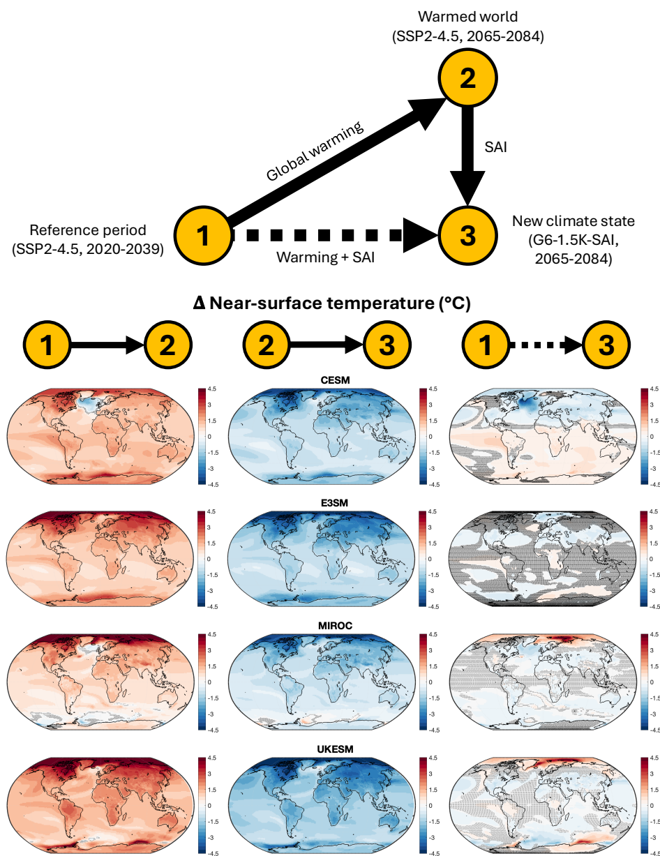
Figure 5. Maps of near-surface air temperature changes (in ^{\circ}\text{C} ) between three different periods: (1) the reference period, 2020-2039 of SSP2-4.5, corresponding to the period over which the GMSAT targets are defined; (2) the warmed world, 2065-2084 of SSP2-4.5, corresponding to the last 20 years of the experimental period; and (3) the new climate state reached under G6-1.5K-SAI in 2065-2084. The left column plots the difference between (1) and (2), representing the changes due to global warming; the middle column plots the difference between (2) and (3), representing the changes due to G6-1.5K-SAI; and the bottom column plots the difference between (1) and (3), representing the combined impacts of warming and G6-1.5K-SAI. Shading represents regions with no statistically significant differences at p = 0.05 according to the two-sample t-test.
