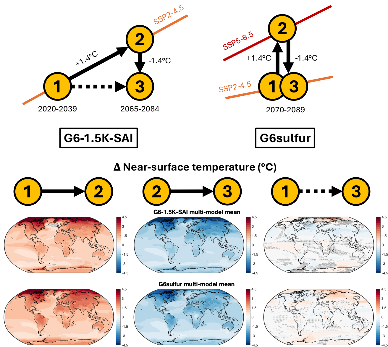
Figure 6. Maps of changes in near-surface air temperature (in °C) as in Fig. 5, for G6-1.5K-SAI and G6sulfur multi-model means. For G6sulfur, all three periods are averages of 2070-2089 data, in which the amount of cooling is approximately the same (1.4°C) as the last 20 years of G6-1.5K-SAI: period 1 is SSP2-4.5, period 2 is SSP5-8.5, and period 3 is G6sulfur. Shading represents areas where models disagree on the sign of the change (fewer than 3 out of 4 for G6-1.5K-SAI, and fewer than 4 out of 6 for G6sulfur).
