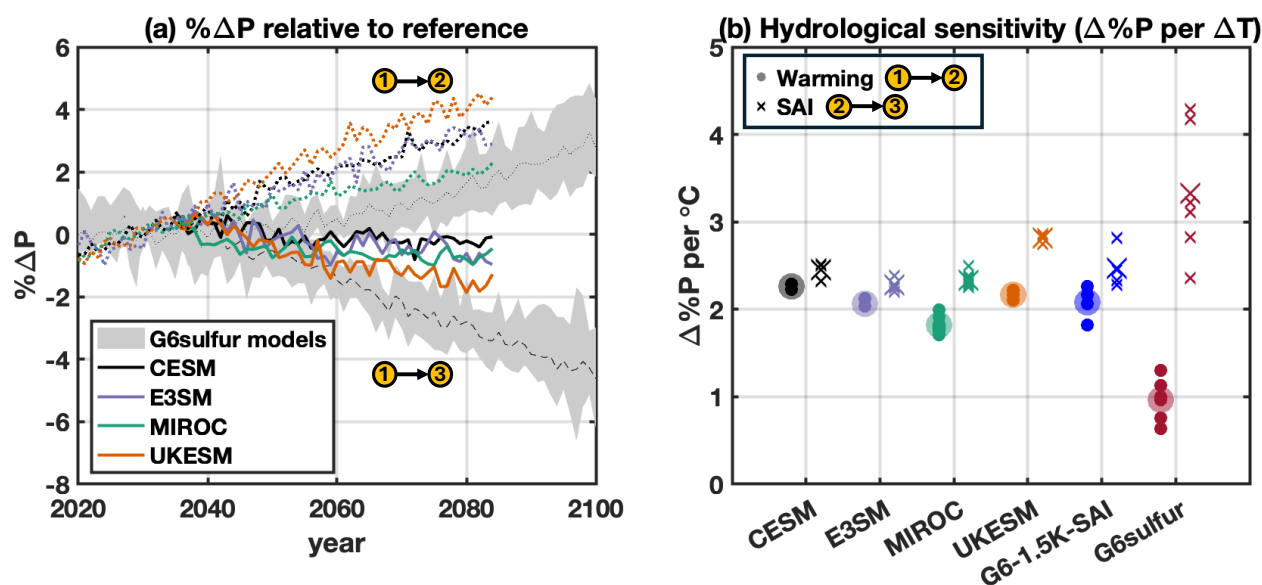
Figure 9. Precipitation (P) changes and hydrological sensitivity for G6-1.5K-SAI- and G6sulfur-participating models. Panel (a) plots changes in global mean precipitation over time, expressed as a % change relative to each model's reference (the SSP2-4.5 2020-2039 mean for G6-1.5K-SAI models, and SSP2-4.5 for G6sulfur models). Colored lines represent ensemble means of G6-1.5K-SAI-participating models, and gray shading denotes the spread of ensemble means of G6sulfur-participating models; dotted lines (values > 0) are for warming scenarios (SSP2-4.5 for G6-1.5K-SAI, and SSP5-8.5 for G6sulfur) and solid/dashed lines (values < 0) are for intervention scenarios (G6-1.5K-SAI and G6sulfur). Panel (b) plots hydrological sensitivity, defined as the % change in global mean precipitation (relative to the reference period) per degree of global mean temperature (T) change; for panel (b), periods 1, 2, and 3 are defined as in Figs. 5-8. Dots indicate warming scenarios (% increase in P per ^{\circ}C of global warming), and x's indicate SAI scenarios (% decrease in P per ^{\circ}C of global warming). For individual G6-1.5K-SAI participating models (left four columns), small symbols denote individual ensemble members, and large symbols denote ensemble means; for multi-model means (right two columns), small symbols denote ensemble means of individual models, and large symbols denote multi-model means.
