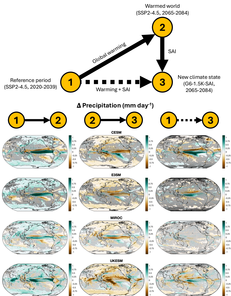
Figure 7. Maps of differences in precipitation (in mm/day) for G6-1.5K-SAI and SSP2-4.5, as in Fig. 5.
