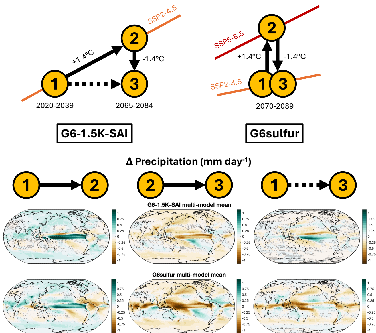
Figure 8. Multi-model mean maps of differences in precipitation (in mm/day) for G6-1.5K-SAI and G6sulfur and their respective warming scenarios, as in Fig. 6.
