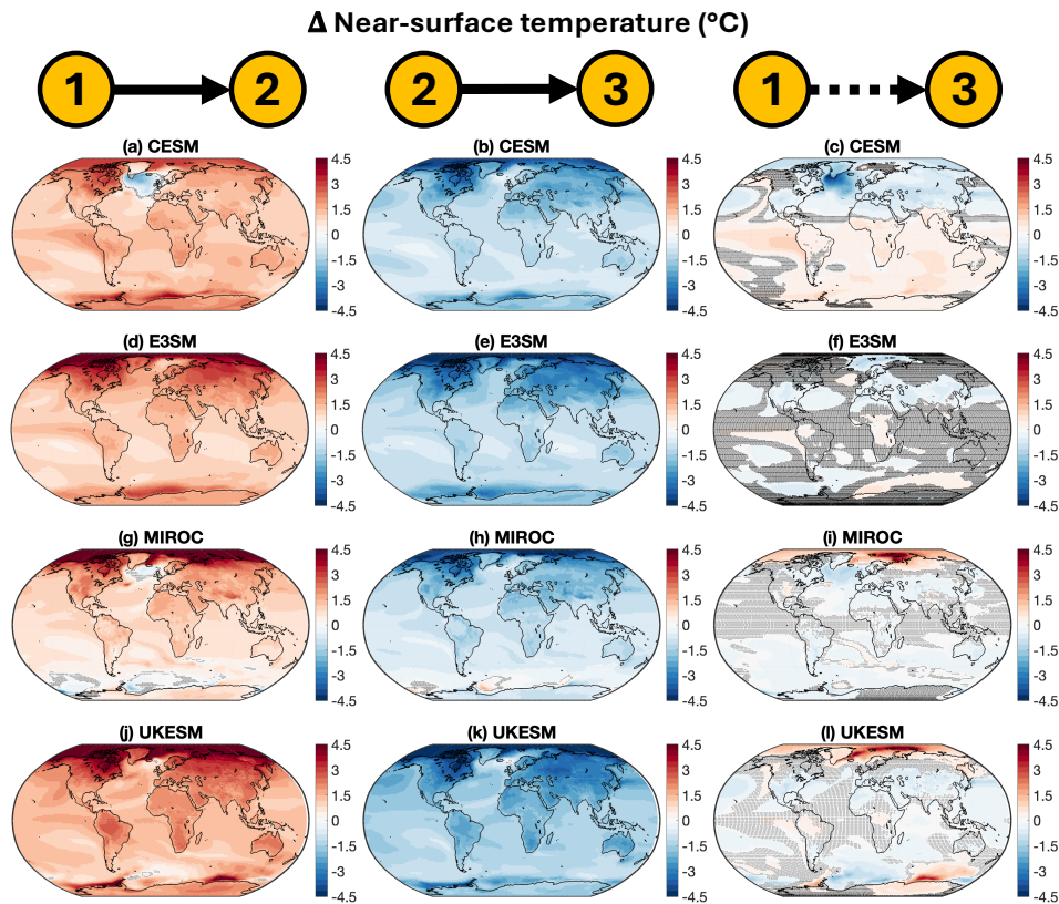
Figure 5. Maps of near-surface air temperature changes (in °C) between three different periods: (1) the reference period, 2020–2039 of SSP2-4.5, corresponding to the period over which the GMSAT targets are defined; (2) the warmed world, 2065–2084 of SSP2-4.5, corresponding to the last 20 years of the experimental period; and (3) the new climate state reached under G6-1.5K-SAI in 2065–2084. The left column plots the difference between (1) and (2), representing the changes due to global warming; the middle column plots the difference between (2) and (3), representing the changes due to G6-1.5K-SAI; and the right column plots the difference between (1) and (3), representing the combined impacts of warming and G6-1.5K-SAI. Shading represents regions with no statistically significant differences at p = 0.05 ; p values are computed for each grid cell, with samples consisting of all individual annual mean data points across all ensemble members from the respective time periods, with samples compared using the two-sample t-test.
