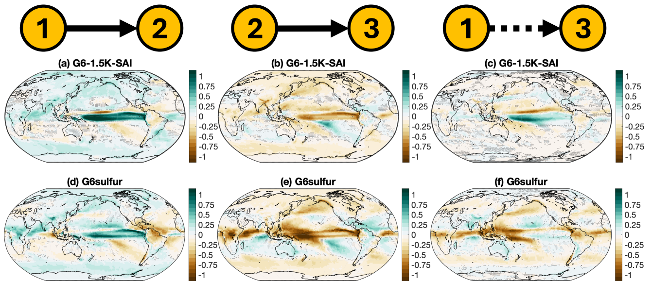
Figure 8. Multi-model mean maps of differences in precipitation (in mm/day) for G6-1.5K-SAI and G6sulfur and their respective warming scenarios, as in Fig. 6.
