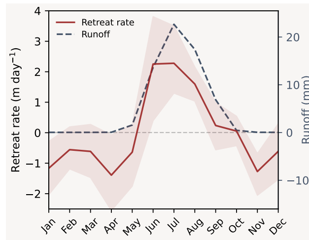
Figure 8. Average monthly retreat rates between 2014 and 2024 (red line with confidence interval as shading), average daily runoff per month (blue stippled line).
