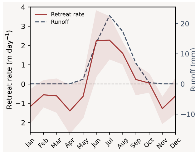
Figure 8. Average The average monthly retreat rates-rate of the marine terminus of Qoogqup Sermia between 2014 and 2024 (red line with confidence interval as shading) and the average daily runoff per month (blue stippled line).
