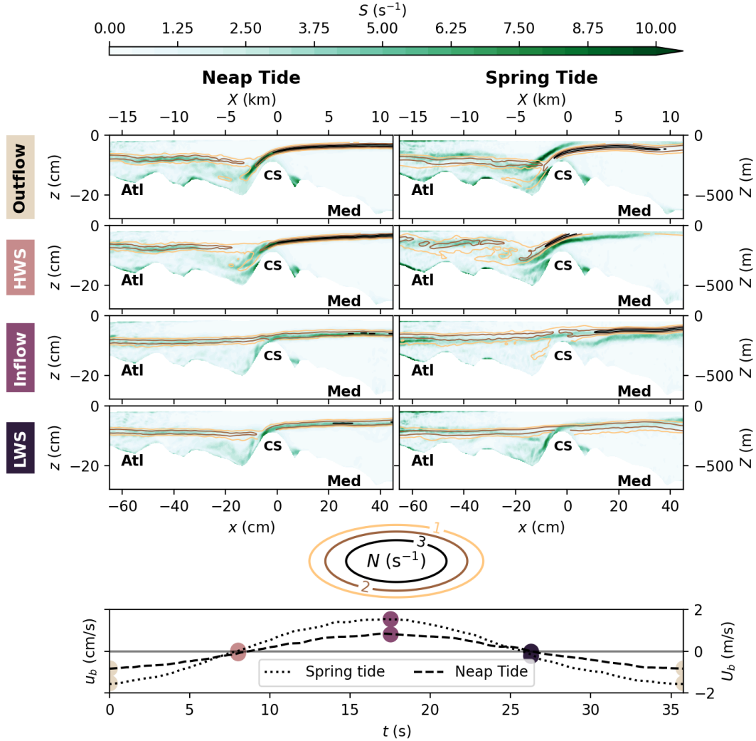
Figure D1. Correlation maps between the vertical velocity shear S (see equation (11) (green colormap) and the Brunt–Väisälä frequency N (colored iso-contours) for maximum outflow, high water slack, maximum inflow and low water slack (from top to bottom, see bottom panel for tidal reference). Neap tide (left panels) and spring tide (right panels). Experimental units (bottom-left), real ocean units (top-right).
