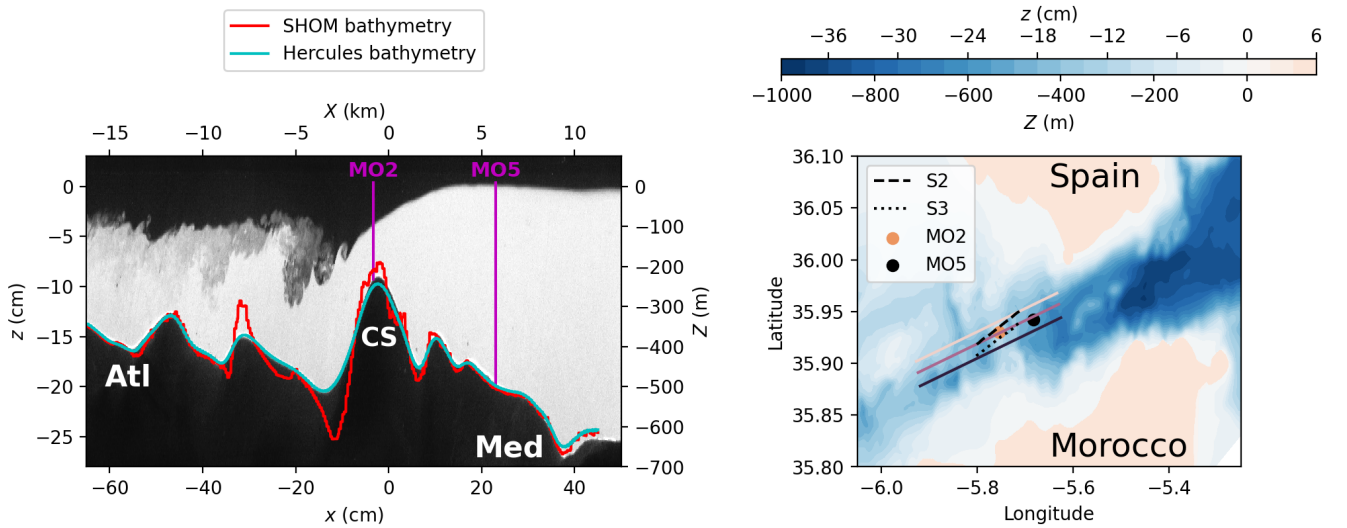
Figure 3. On the left, an instantaneous image of the laser plane during the experiment comparing the real topography (red line), the smoothed topography used in the present experiments (blue line) and the topography after calibration as registered on the camera images (black shadow), for the central transect. Vertical magenta lines gives the position closest to MO2 and MO5 moorings. On the right, sketch of the three transects considered for the PIV/LIF measurements (continuous lines), the middle one passing through the CS summit, and further southern and northern transects. The positions of the moorings MO2 and MO5 of the PROTEVS GIB2020 campaign (Bordoïs and Dumas, 2020) are given as well, along with the transects S2 and S3 (dashed and dotted lines, respectively), that will be used for comparison with the experimental data.
