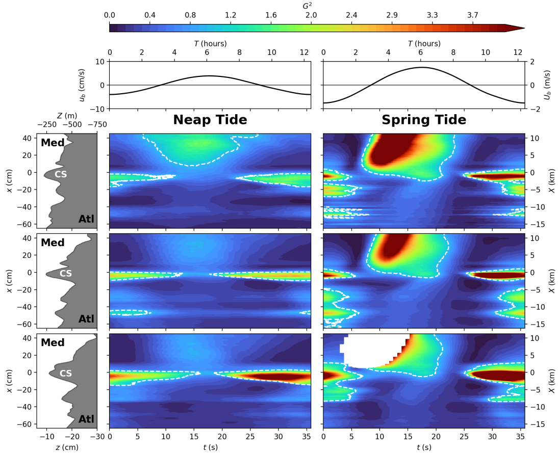
Figure 14. Evolution of the composite Froude number G^2 (cf. equation (10) with the tide for the northern (top panels), the middle (middle panels) and the southern (bottom panels) transects in neap tide (left columns) and spring tide (right column). White dashed lines delimit G^2 = 1 . Experimental units (bottom-left), real ocean units (top-right).
