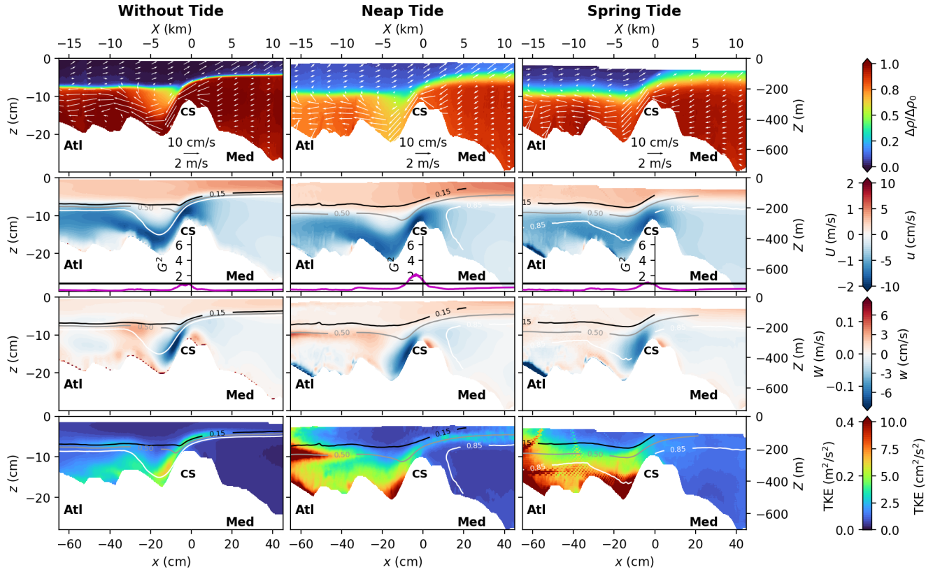
Figure A3. Same as figure A2 but for the southern transect.
