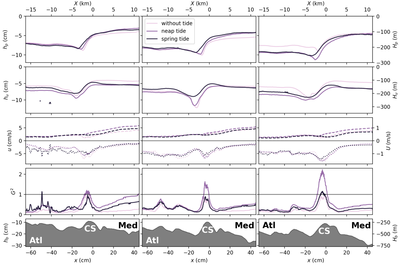
Figure 6. Two-layer time-averaged (over seven tidal cycles) flow characteristics at CS for the planes (from left to right: northern, middle and southern transects) for the three tidal forcing. From top to bottom: pycnocline depth h_p ; surface of maximum vertical gradient of along-strait velocity h_u ; vertically integrated along-strait velocity u for the Mediterranean (dotted lines) and Atlantic (dashed lines) layers; two layer composite Froude number G^2 ; bathymetry. Experimental units (bottom-left), real ocean units (top-right).
