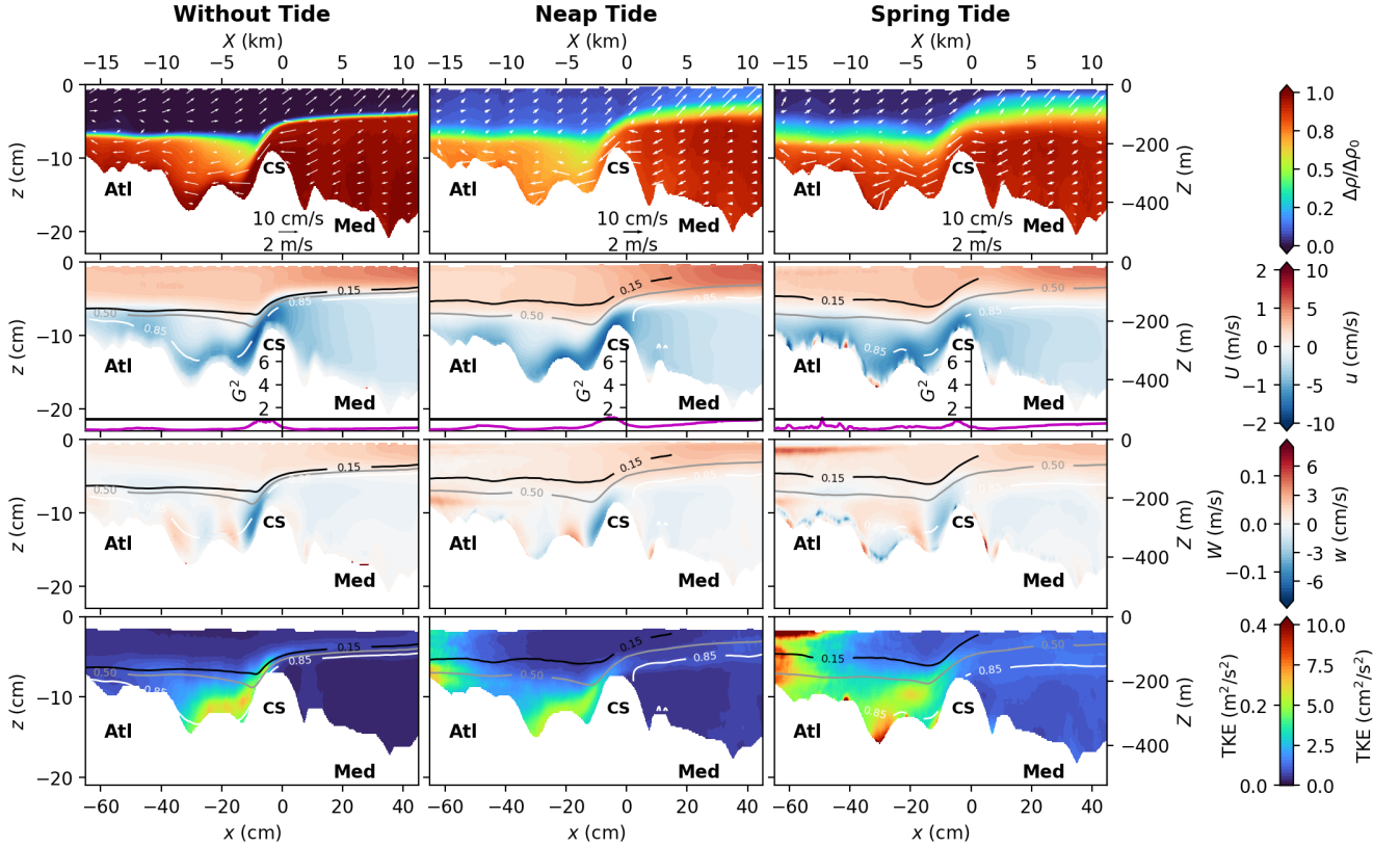
Figure A2. Mean flow characteristics for the northern transect passing north of the CS summit (cf. figure 3b), for the three tidal forcings: without tide, neap tide, and spring tide from left to right. The x axis represents the along-transect coordinate, being positive toward the east. The first row displays the mean density with the averaged velocities (\bar{u}, \bar{w}) (white arrows). The second and third rows panels display the mean horizontal u and vertical w velocities, respectively, superposed with the \Delta\rho/\Delta\rho_0 = 0.15, 0.5 , and 0.85 (black, grey, and white lines respectively). In between, the composite Froude number G^2 is displayed as a purple line. The last row panels display the turbulent kinetic energy TKE = (\overline{u'^2} + \overline{w'^2})/2 . Experimental units (bottom-left), real ocean units (top-right).
