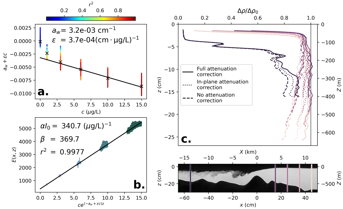
Figure A1. a) Attenuation coefficient as a function of Rhodamine concentration. The colorbar indicates the determined coefficient r^2 of each linear regression used to compute the attenuation coefficient. (b) Light E on the camera sensor against the corrected Rhodamine concentration ce^{-(a_w + \epsilon c)z} . Black lines represent linear interpolations. (c) Effect of the LIF corrections on five vertical density profiles during outflow. Dashed lines represent no correction, dotted lines include correction for absorption along the laser paths, solid lines include additionally the absorption of light along the path to the camera. The vertical solid line indicates the initial imposed density difference between Mediterranean and Atlantic waters for reference.
