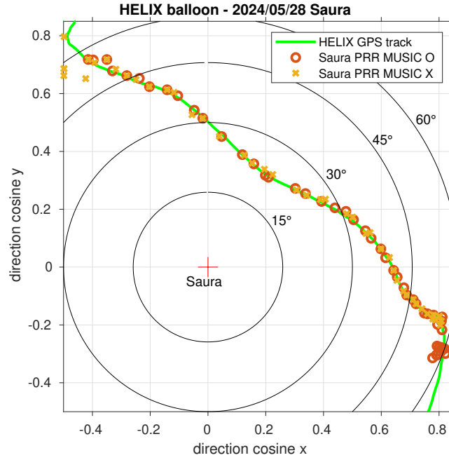
Figure 6. Helix trajectory (green) superimposed with the derived MUSIC positions for O- and X-mode of Saura with corresponding symbols.
