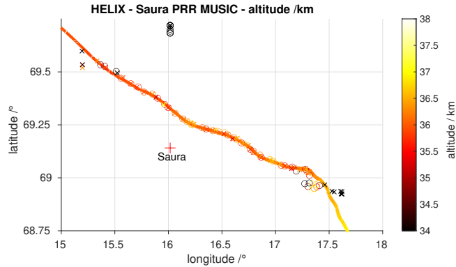
Figure 7. Trajectory of HELIX (dots) superimposed by derived AoA positions for Saura using MUSIC (O and X symbols for corresponding magneto-ionic mode), color-coded are the altitudes for both.
