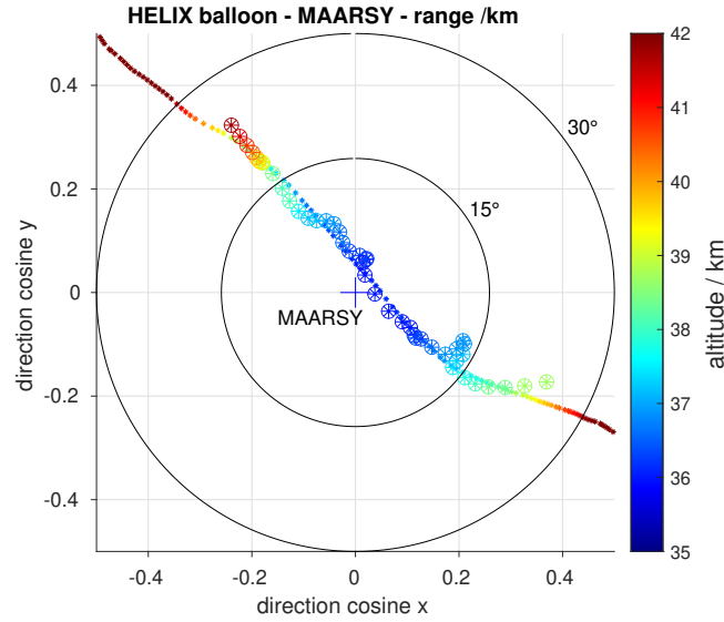
Figure 8. Trajectory of HELIX converted to spherical coordinates at MAARSY location superimposed by the derived MUSIC positions using eight hexagon-shaped subarray groups.
