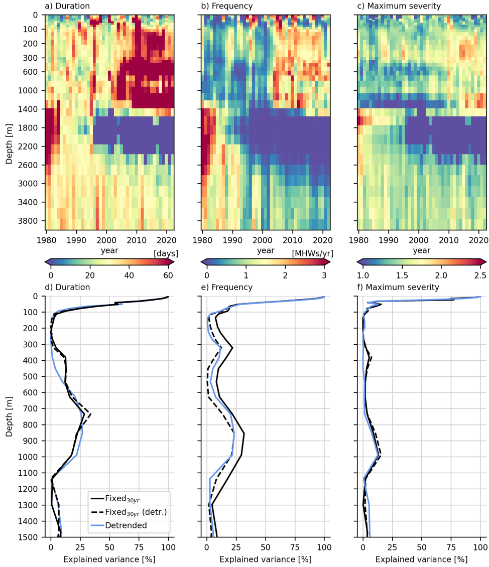
Figure 9. Annual mean MHW duration, frequency and sealed-maximum intensity-severity in the Cape Verde archipelago (fixed 30yr baseline; VIKING20X-6th; a-c). Explained variance of the MHW duration, frequency and sealed-maximum intensity-severity at different depth by their annual mean values at the surface (d-f). The explained variance was calculated for the fixed 30yr baseline (black, solid) and for the detrended baseline (blue). Additionally, the dashed lines represent the explained variance based on the same fixed 30yr baseline detection, with the trend in the MHW characteristics removed.
