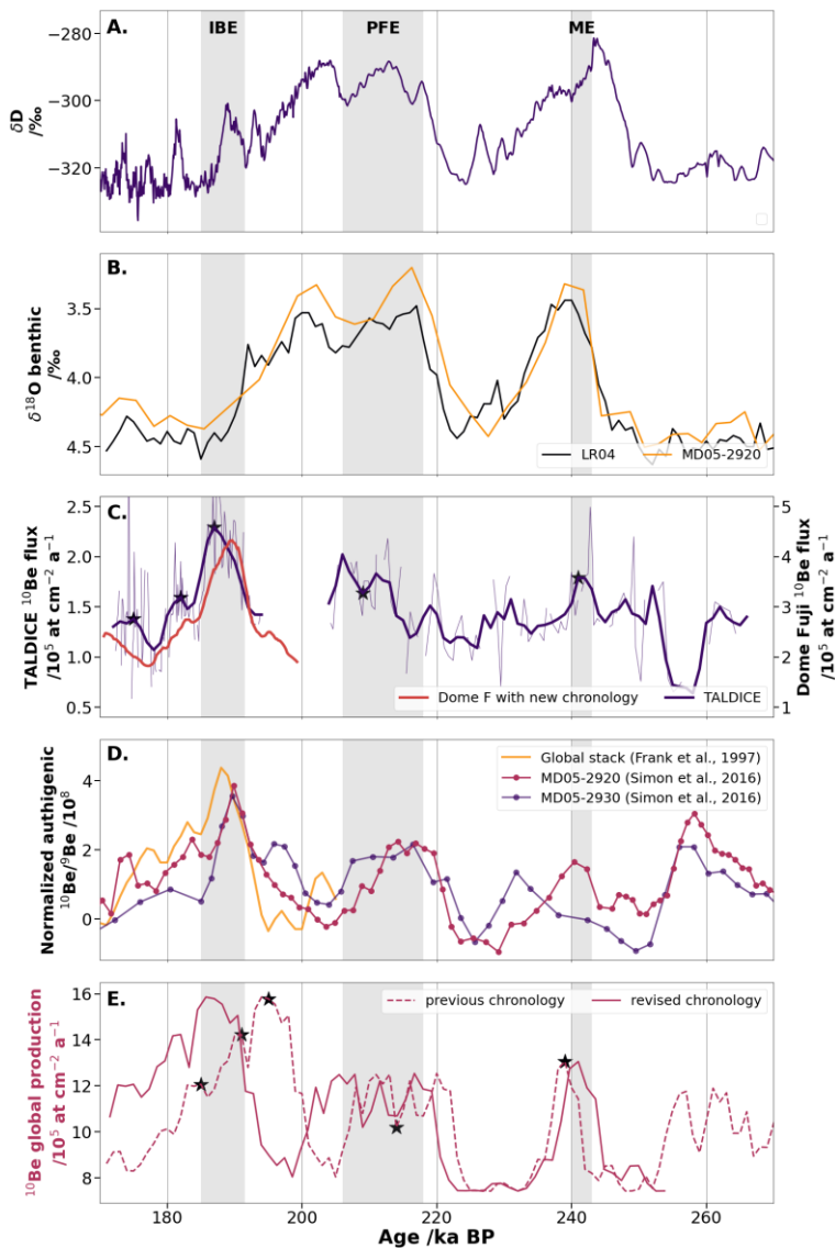
Figure 5: Comparison of ^{10}\text{Be} and climate records from ice cores and marine sediments over 170–270 ka BP with, in order : A. TALDICE \delta D (‰), B. benthic \delta^{18}\text{O} (‰) from LR04 stack (Lisiecki and Raymo, 2005) and MD05-2920 (Tachikawa et al., 515 C. TALDICE and Dome Fuji ^{10}\text{Be} (in purple and red respectively, /\text{at cm}^{-2} \text{a}^{-1} ), D. authigenic ^{10}\text{Be}/^9\text{Be} from global stack reconstruction (yellow, (Frank et al., 1997)) , MD05-2920 (red), and MD05-2930 (purple) MD05-2920 (yellow) and MD05- 2930 (orange) (Simon et al., 2016), and E. the ^{10}\text{Be} global production ( /\text{at cm}^{-2} \text{a}^{-1} ; Poluianov et al., 2016) calculated from RPI-based VADM (Channell et al., 2009). Grey bars highlight the main geomagnetic excursions discussed in the text (IBE, PFE, ME). Timing of identifiable geomagnetic features (black stars in TALDICE, MD05-2920, and RPI-based VADM) is used 520 to obtain a revised chronology of RPI-based VADM used for calculating the ^{10}\text{Be} production, noting though a lower confidence on the star around 210 ka BP.
