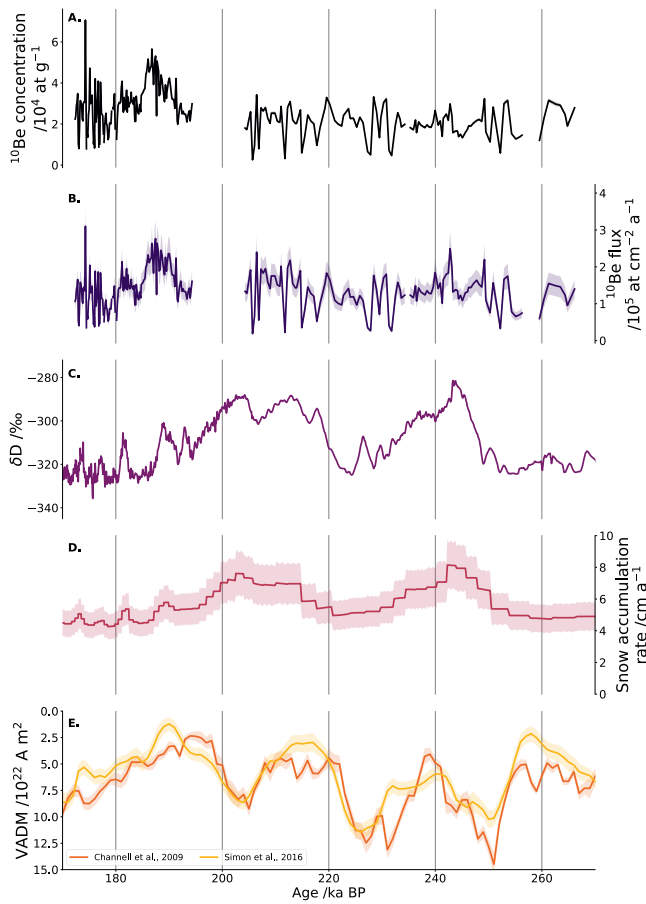
Figure 2: A) TALDICE ^{10}\text{Be} concentration ( 10^4 at \text{g}^{-1} ; A ) with the concentration uncertainty (shaded black; 3.6 % on average). B) ^{10}\text{Be} and flux ( 10^5 at \text{cm}^{-2} \text{a}^{-1} ; B ) with the uncertainty (shaded purple) which, in the case of flux, the variation of the accumulation (see section 4). C) Climate variations are recorded in TALDICE with \delta\text{D} water isotopes (‰; C ; Stenni et al., 2011), from which Marine isotope stage can be listed (6.4 to 8.3; Railsback et al., 2015). D) Snow accumulation rate ( \text{cm} \text{a}^{-1} ; D ) is retrieved from the AICC2023 chronology (Bouchet et al., 2023). E) Virtual Axial Dipole Moment (VADM, \text{A} \text{m}^2 ) is estimated from Relative Paleointensity (PISO-1500; Channell et al., 2009) (orange) or from authigenic ^{10}\text{Be}/^9\text{Be} (Simon et al., 2016). Note that the y-axis is reversed.
